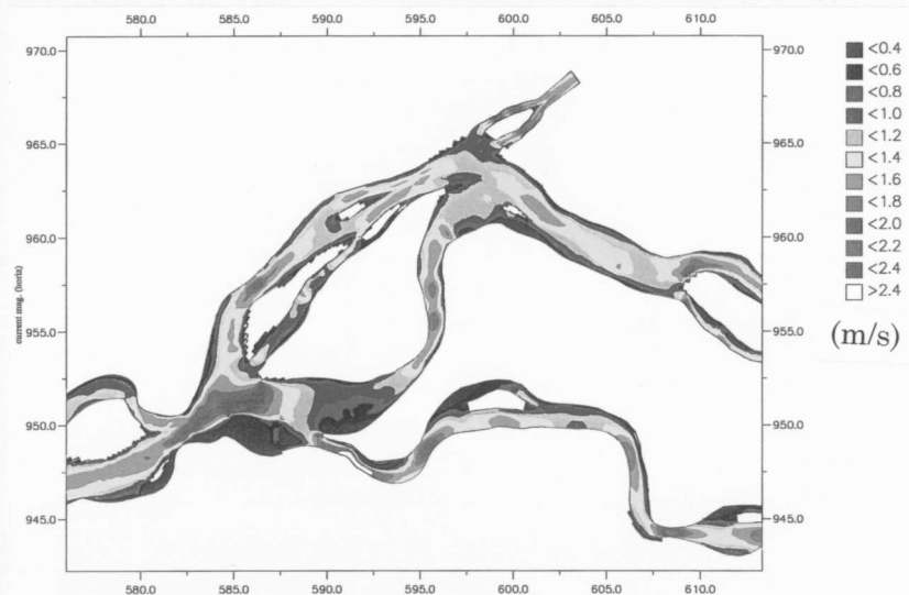
Contour of Current Magnitude (Alt. B2-6, Q=66,000 m 3 /s)
