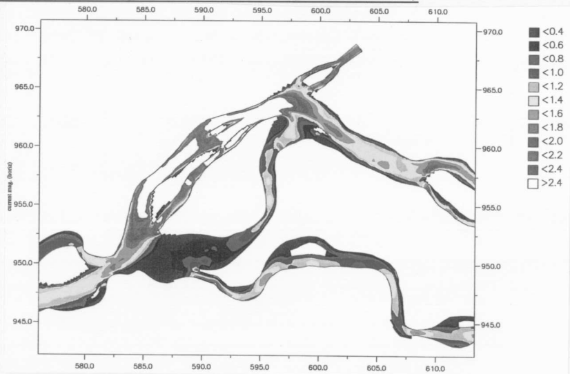
Contour of Current Magnitude (Alt. B2-8, Q=66,000 m 3 /s)
