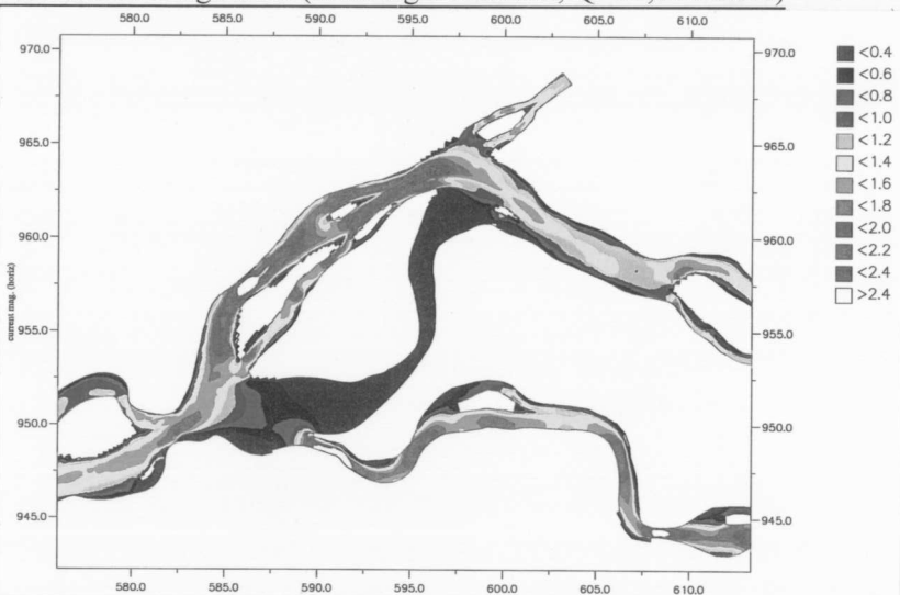
Contour of Current Magnitude (Alt. B2-1, Q=66,000 m3/s)
