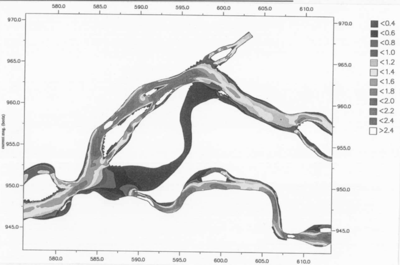
Contour of Current Magnitude (Alt. B2-2, Q=66,000 m3/s)
