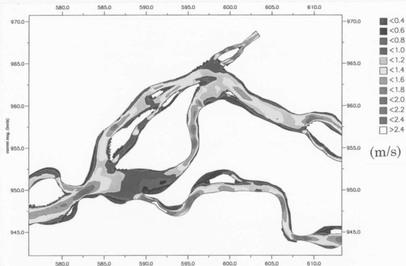
Contour of Current Magnitude (Existing Condition, Q=66,000 m3/s)
