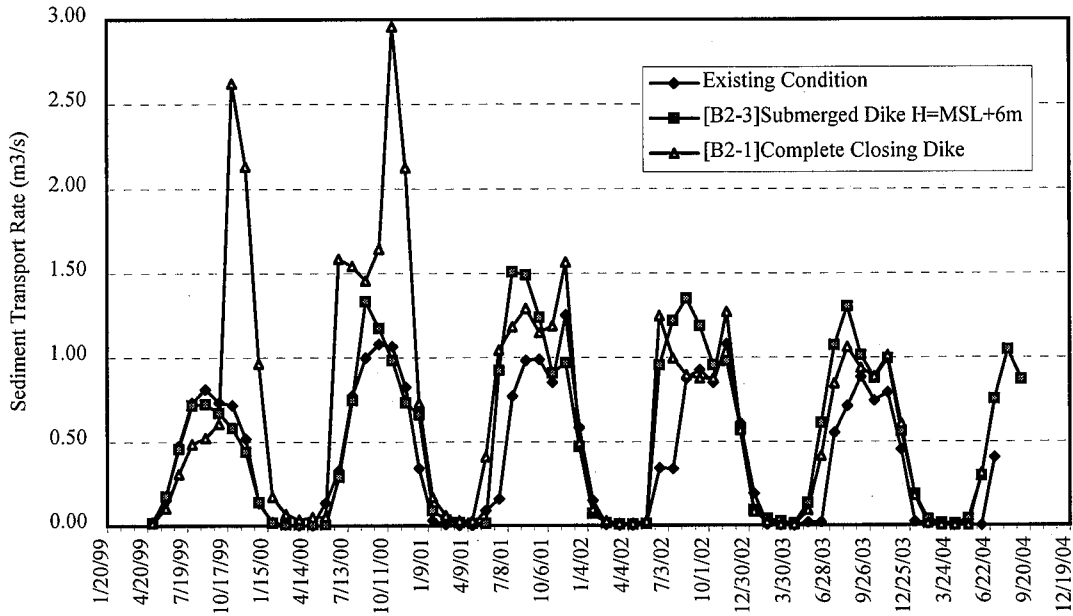
Sediment Transport Rate at Ya-Ya (C-9)
