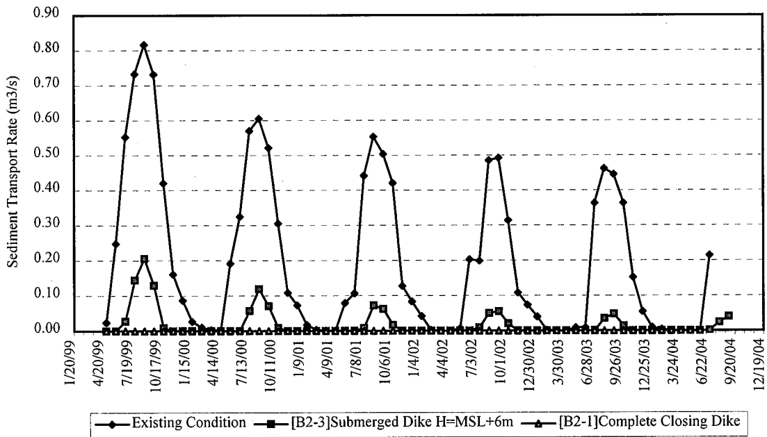
Sediment Transport Rate at Tortola Downstream (C-4)
