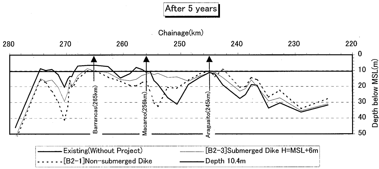
Fig. 7-3-30 Longitudinal Profiles of Bed Elevation Change for [B2-1] and [B2-3]
