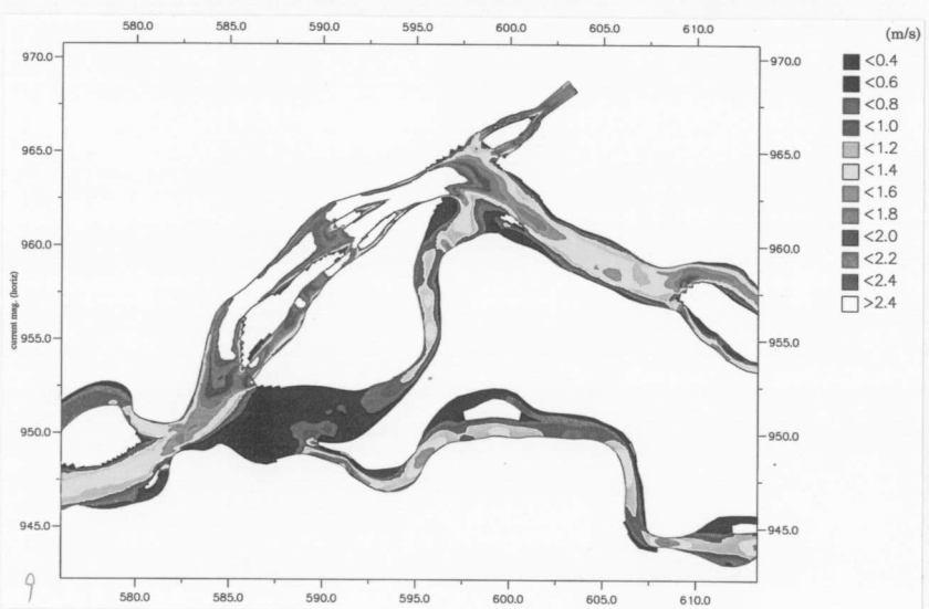
Fig.7-3-25(3/3) Contour of Current Magnitude of Alternative
