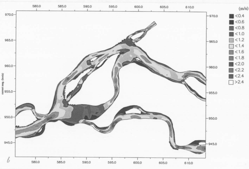
Fig.7-3-25 (2/3) Contour of Current Magnitude of Alternative
