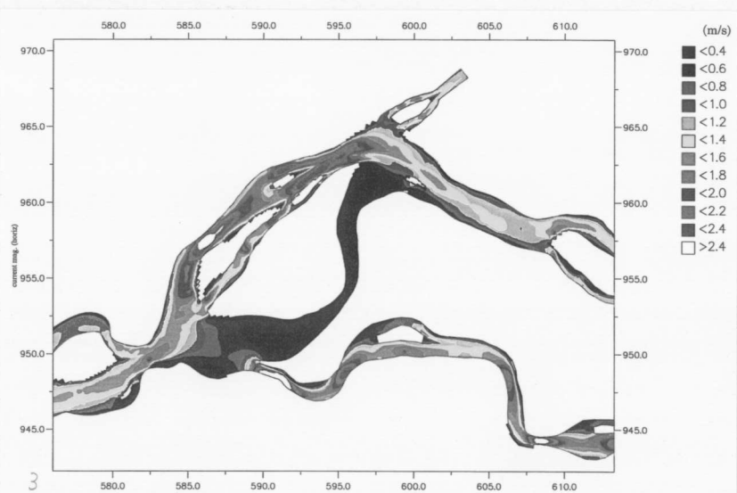
Fig.7-3-25 (1/3) Contour of Current Magnitude of Alternative
