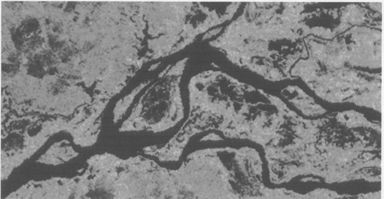
Radarsat Image of July 1998 by JICA Study Team
