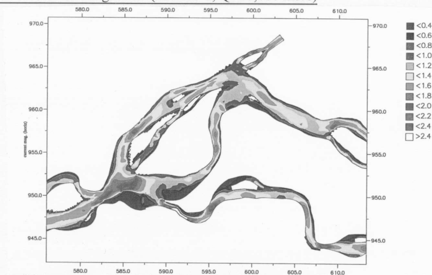
Contour of Current Magnitude (Alt. B2-7, Q=66,000 \text{ m}^3/\text{s} )
