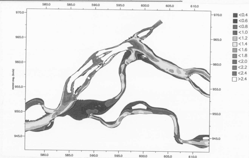
Contour of Current Magnitude (Alt. B2-8, Q=66,000 \text{ m}^3/\text{s} )
