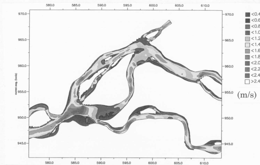
Contour of Current Magnitude (Alt. B2-6, Q=66,000 \text{ m}^3/\text{s} )
