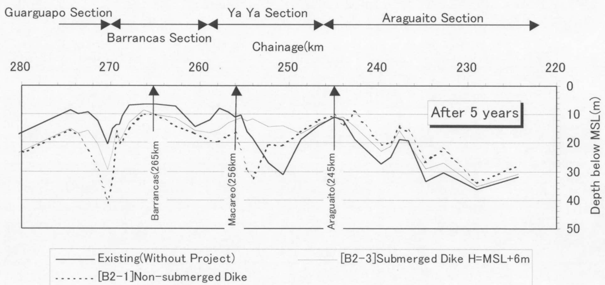
Fig. S-7-1 Results of 2 Dimensional Simulation Analysis
