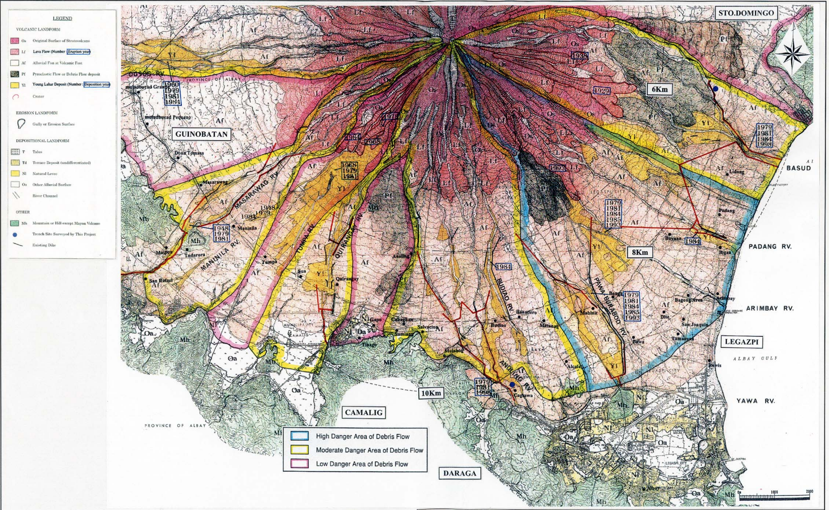
COMPREHENSIVE DISASTER PREVENTION AROUND MAYON VOLCANO IN THE REPUBLIC OF THE PHILIPPINES Figure VI 3.9 Hazard Map of Lahar and Debris Flow (2) JAPAN INTERNATIONAL COOPERATION AGENCY
