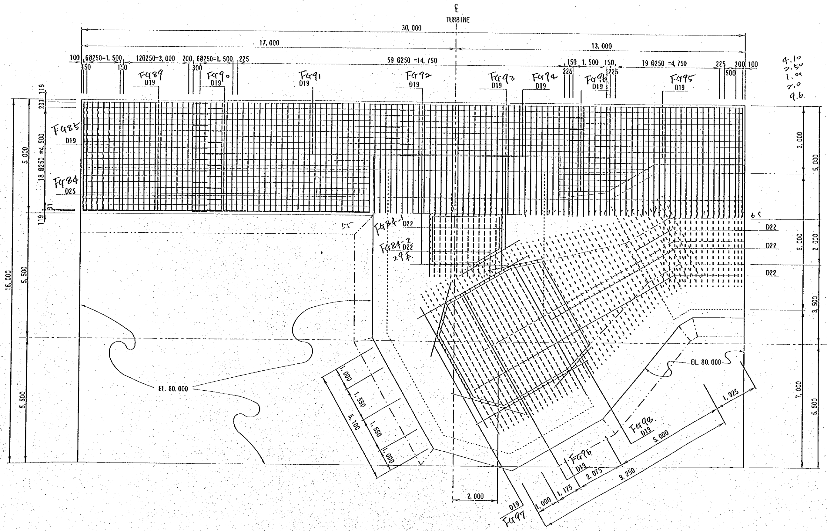
EL. 80.000 FLOOR
