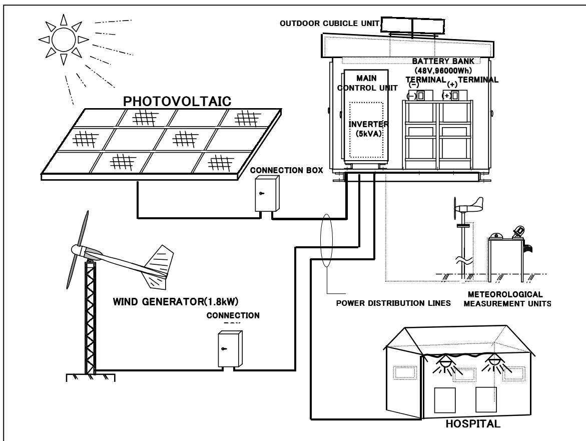
Figure II.1-1 Composition of the pilot plant
