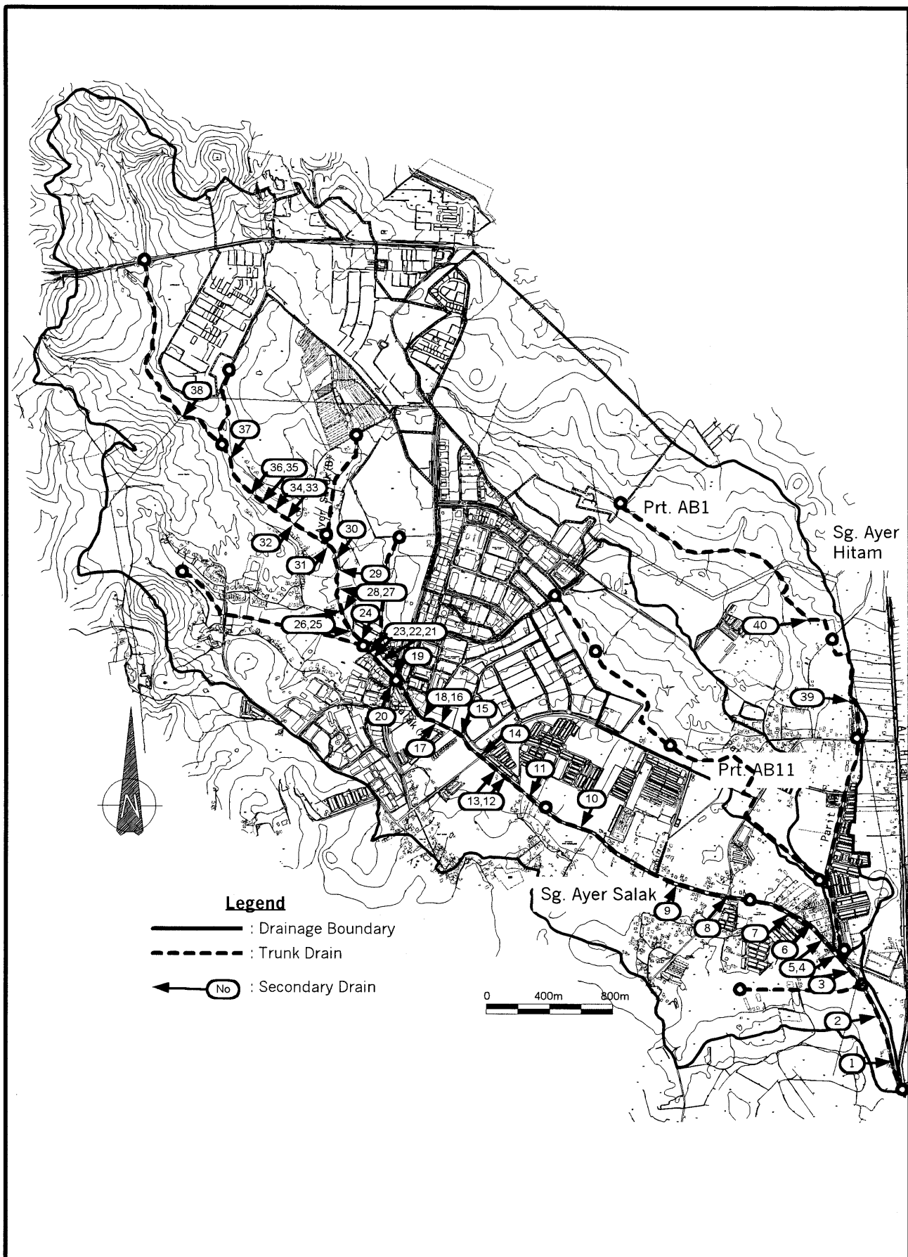
Fig. IV-6(4/4) Major Secondary Drains in Sg. Ayer Salak Drainage Basin
