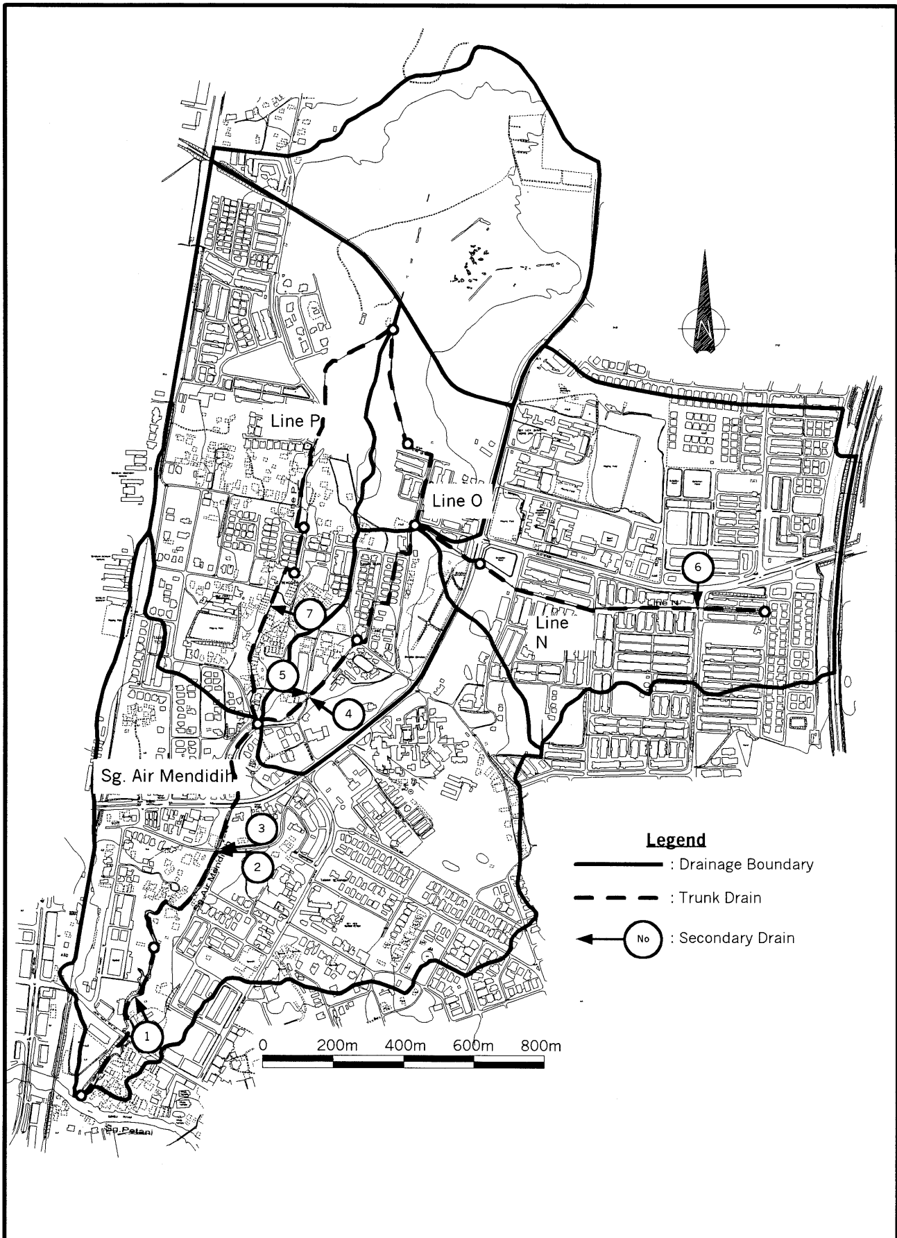
Fig. IV-6(1/4) Major Secondary Drains in Sg. Air Mendidih Drainage Basin
