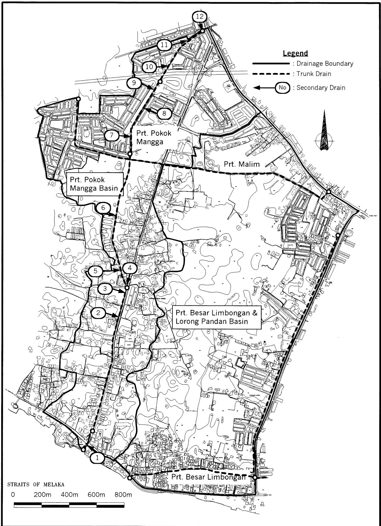
Fig. IV-6(3/4) Major Secondary Drains in Prt. Pokok Mangga Drainage Basin
