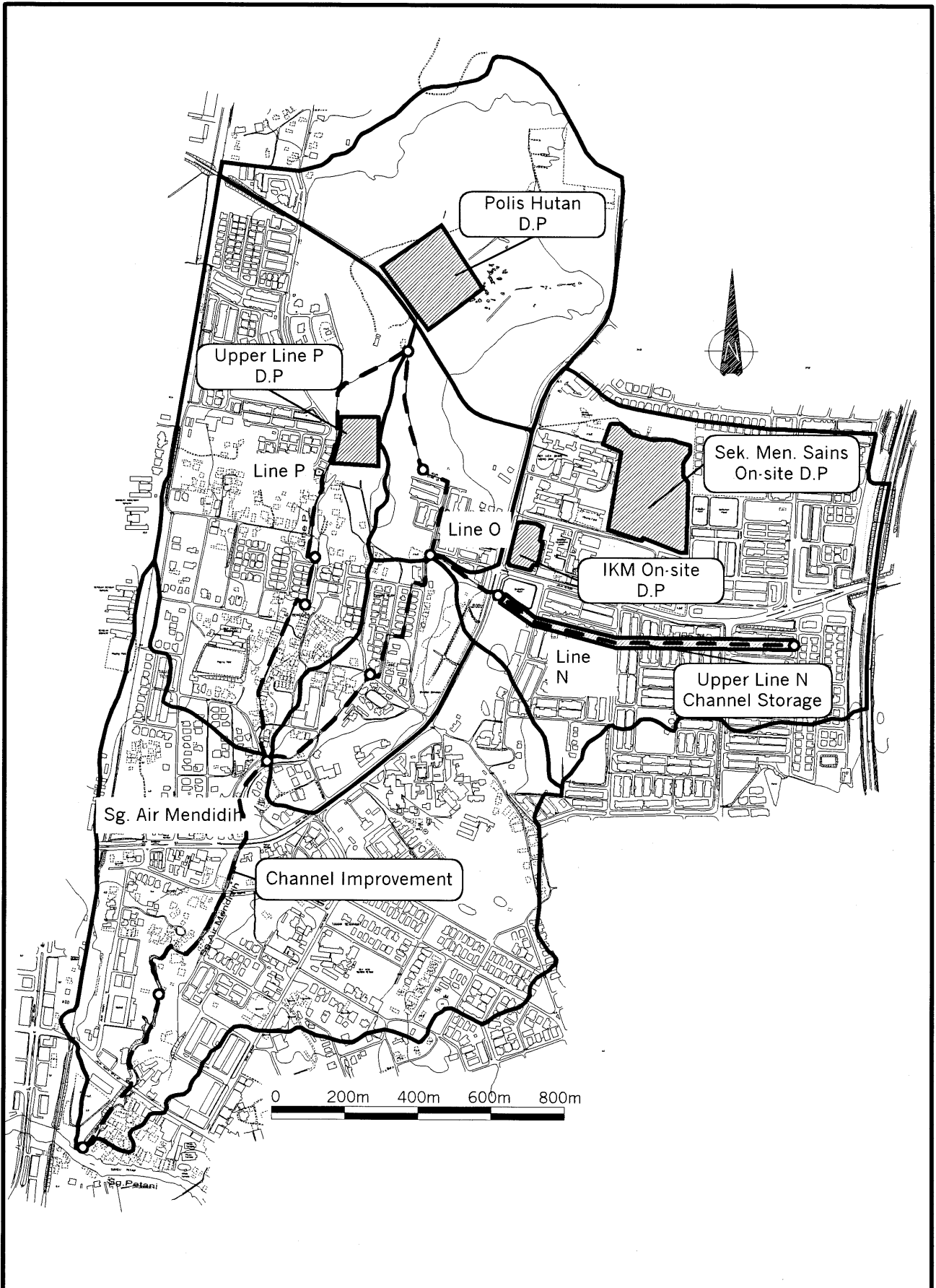
Fig. IV-7 Possible Structural Measures for Drainage Improvement in Sg. Air Mendidih Basin
