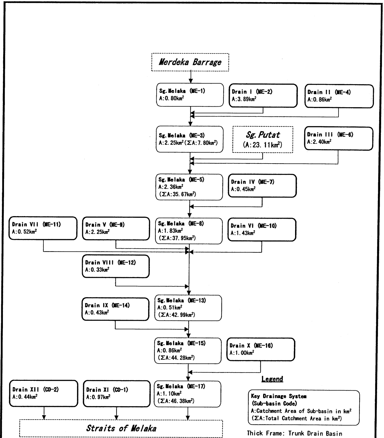
Sg. Melaka Basin and Individual Coastal Drains (Downstream of Merdeka Barrage)
