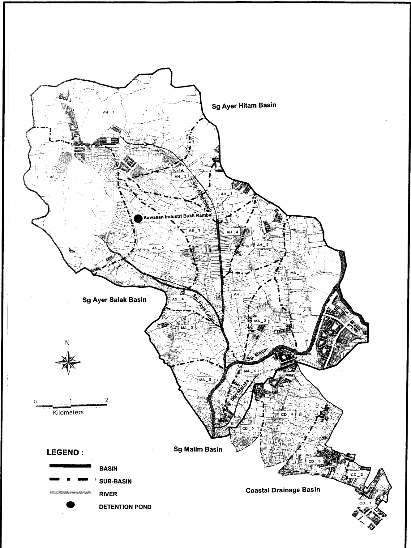
Fig. IV-5(5/5) Location Map of Detention Pond (Sg. Ayer Salak Basin)
