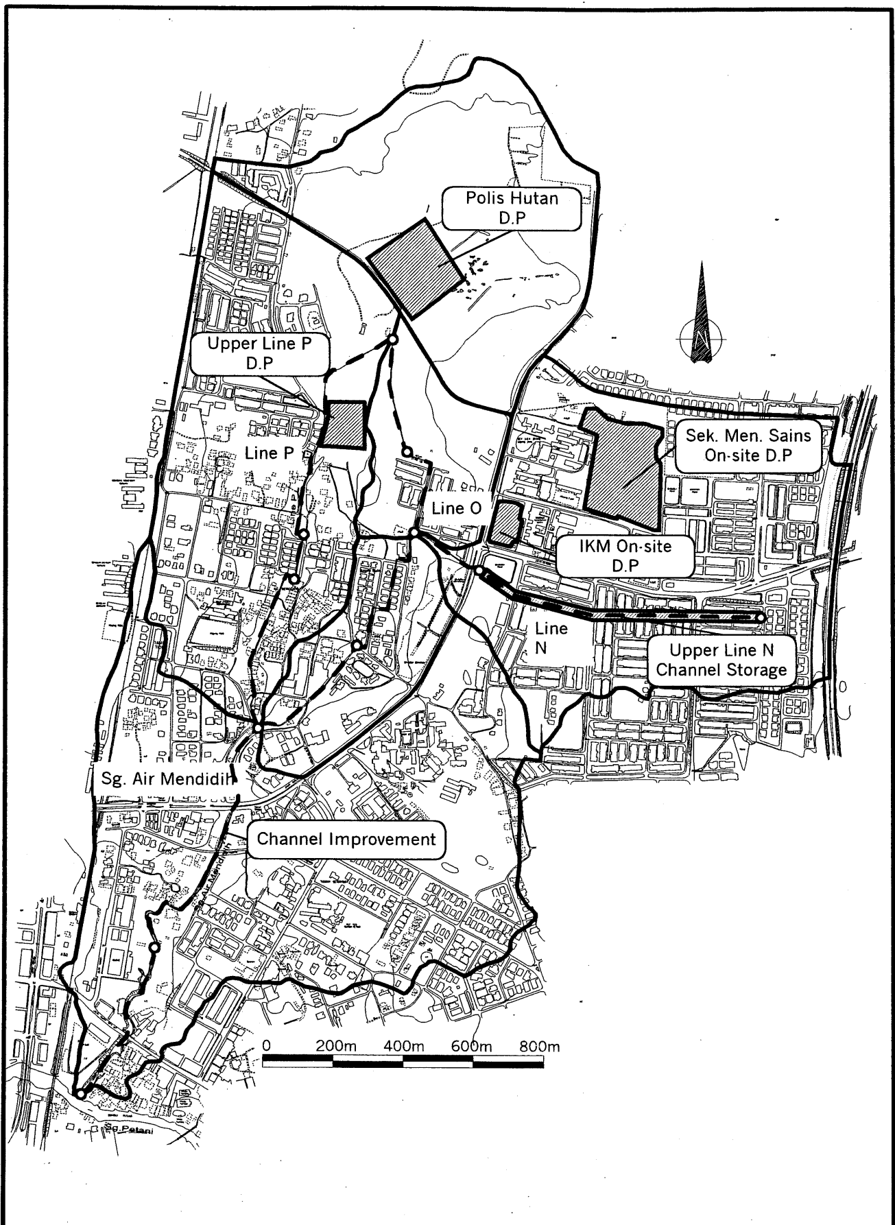
Fig. 4-1 Possible Structural Measures for Drainage Improvement in Sg. Air Mendidih Basin
