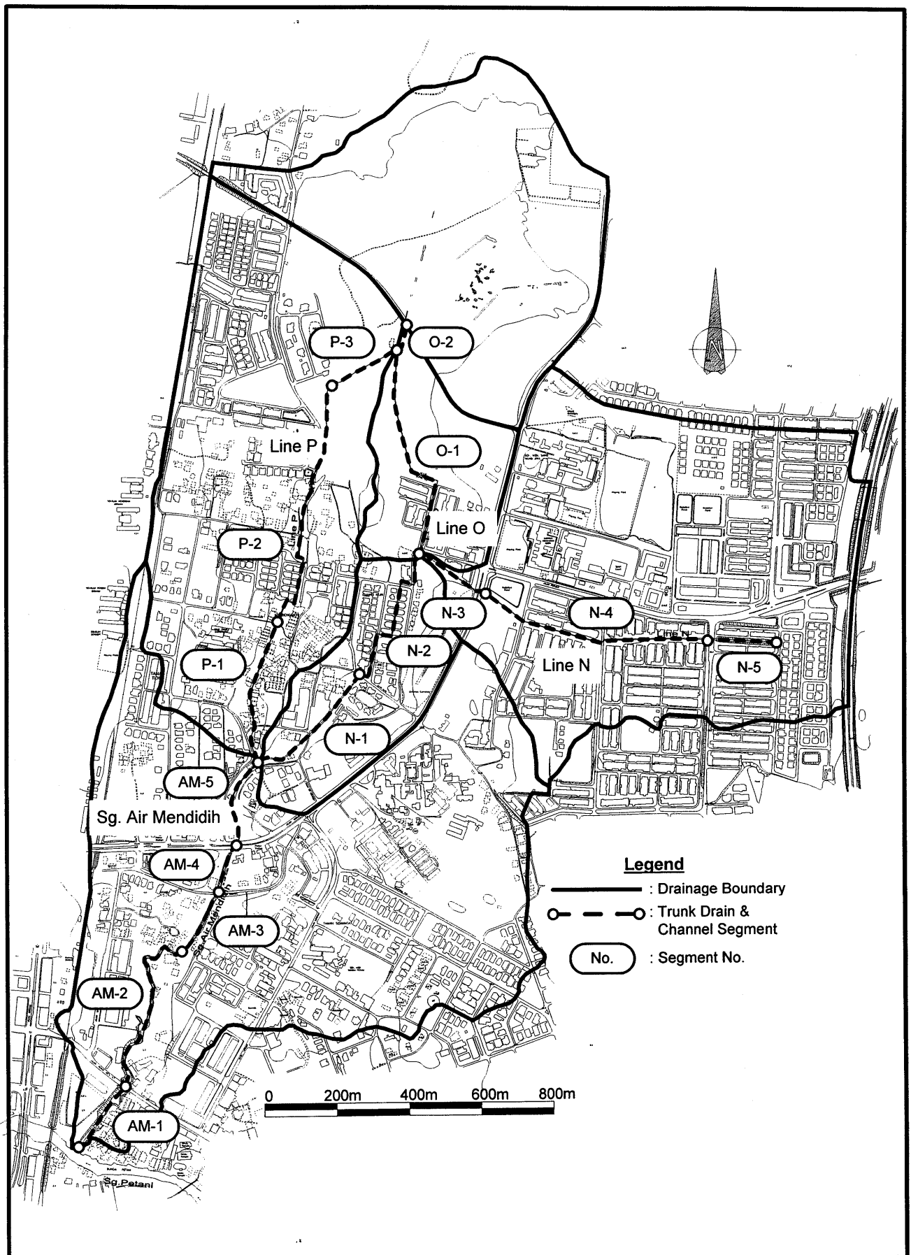
Fig. 4-2 Trunk Drain Network in Sg. Air Mendidih Basin
