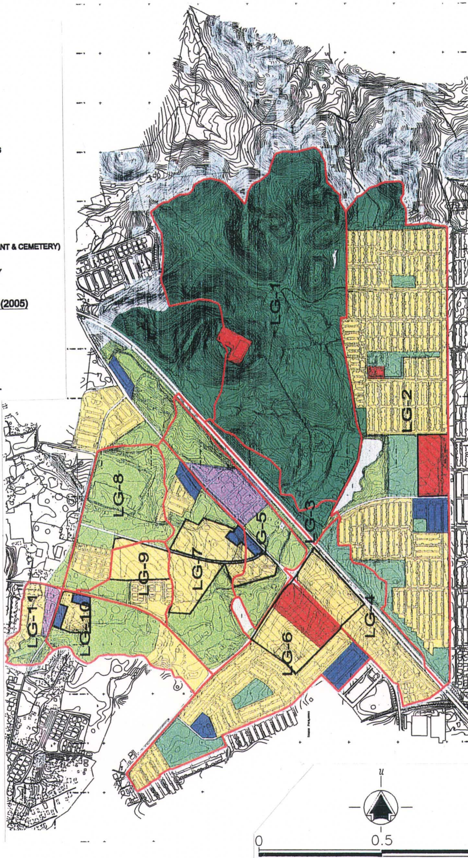
Fig. 2-12 Committed Land Use by 2005 for Drainage Area of Line G
