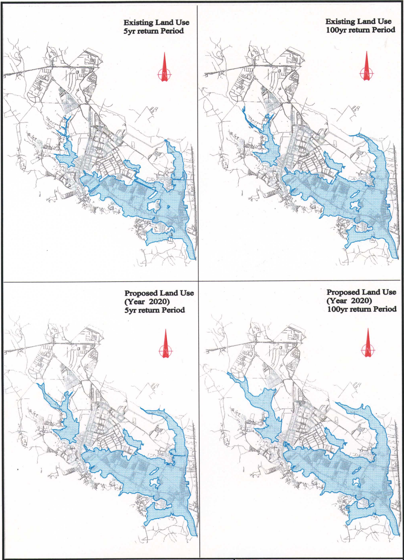
Fig.3-13(4/4) Probable Extent of Flood Inundation Area (Sg. Ayer Salak)
