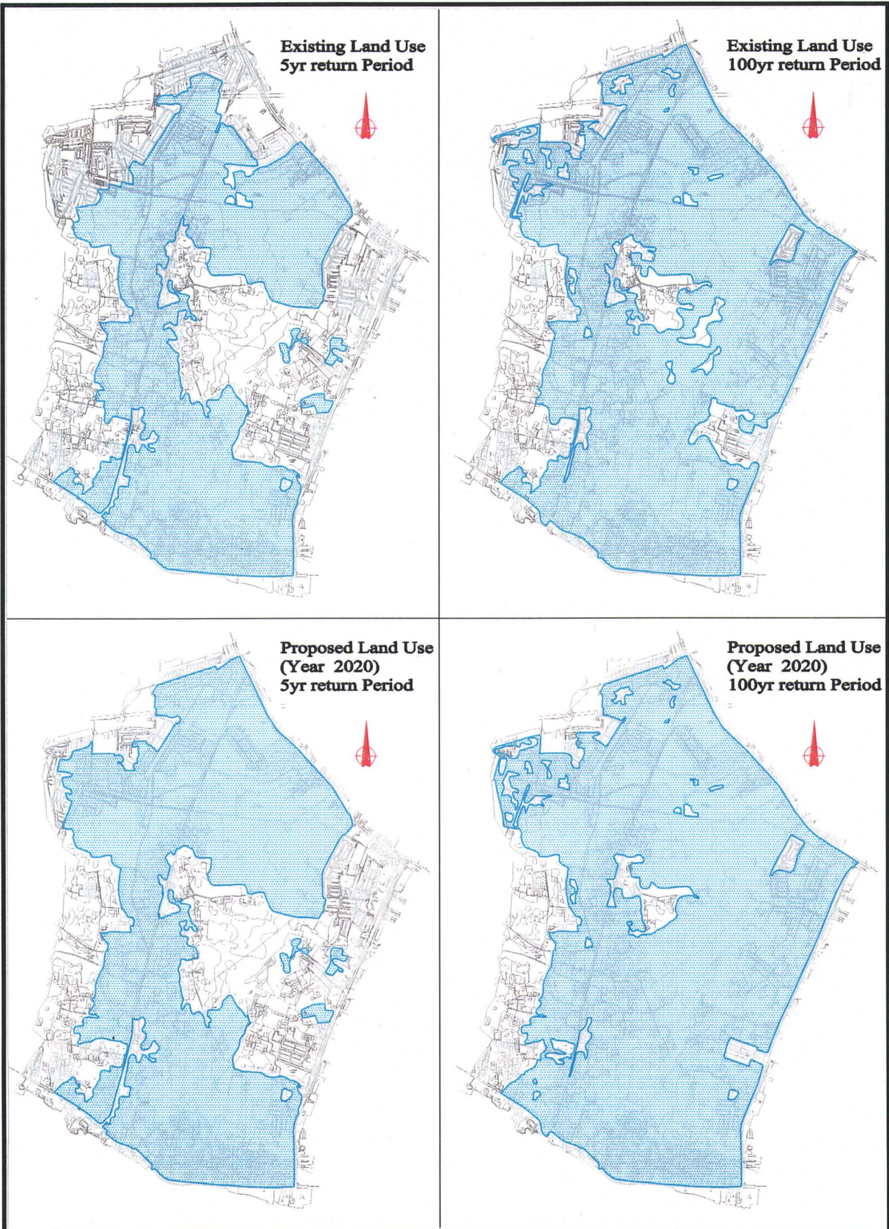
Fig.3-13(3/4) Probable Extent of Flood Inundation Area (Prt.Pokok Mangga)
