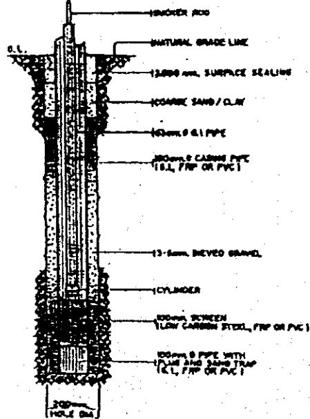
OPEN HOLE DRILLING & GRAVEL PACK METHOD
