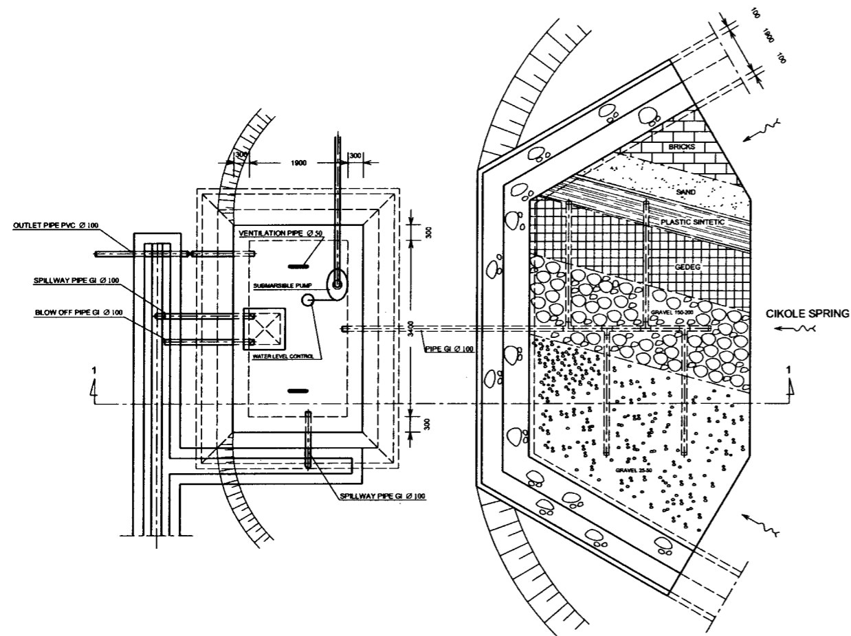
INTAKE (CAPTURING) SCALE 1:100
