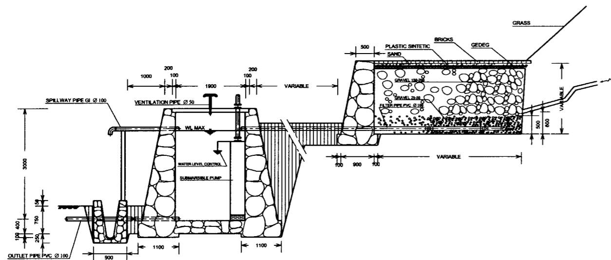
SECTION 1-1 SCALE 1:100
