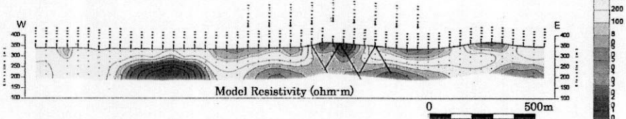
Result of 2D_Inversion Line-N750 Kekoro Area
