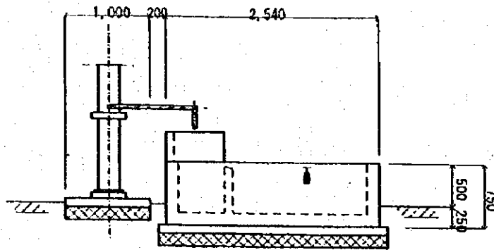
Section (1) — (1) S = 1/30
