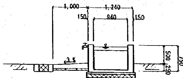
Section (2) — (2) S = 1/30
