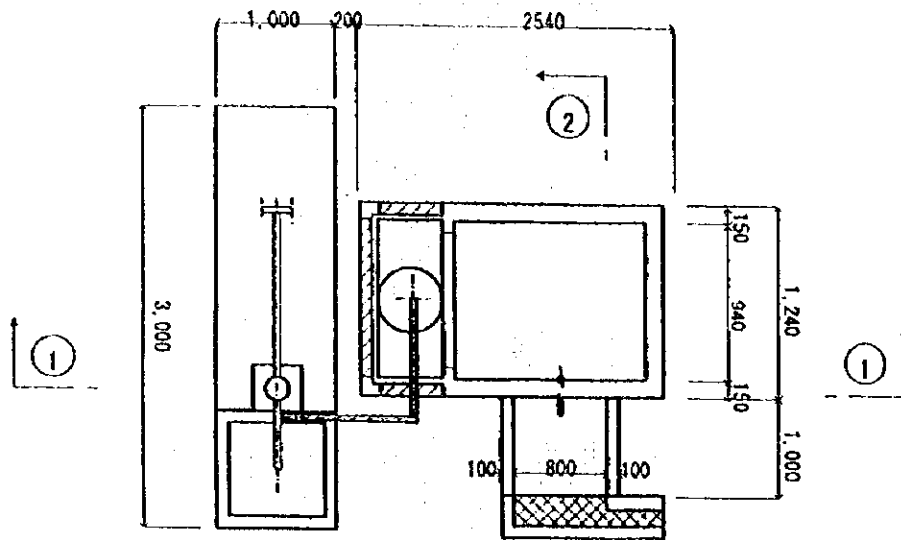
PLAN S = 1/30 (2)
