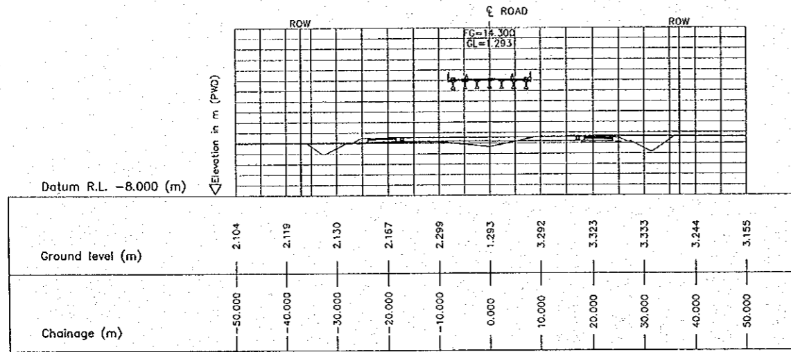
3 CROSS SECTION (STA. 8000.000) E-23 SCALE 1:500
