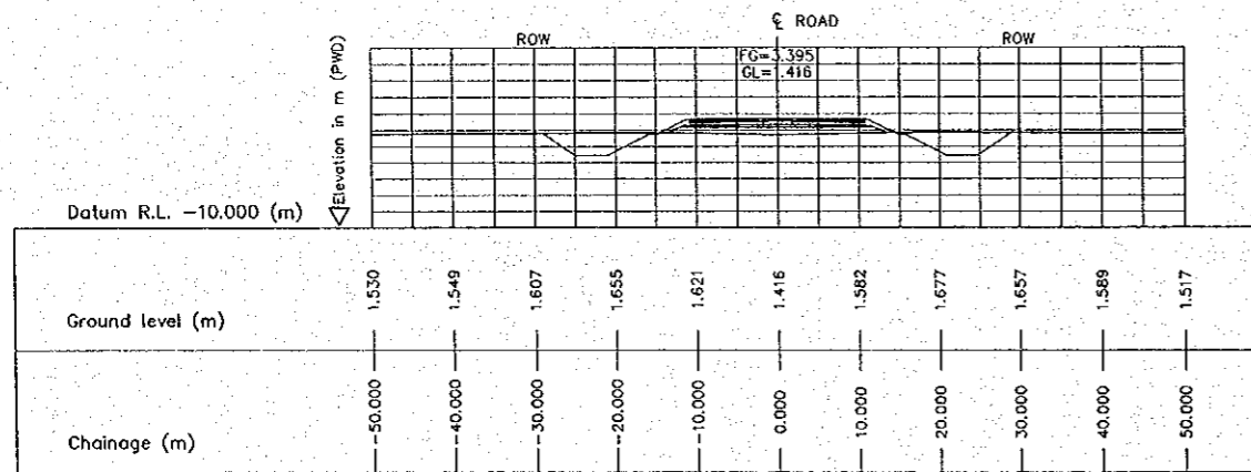
2 CROSS SECTION (STA. 5250.000) E-15 SCALE 1:500
