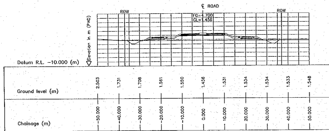
3 CROSS SECTION (STA. 6800.000) E-20 SCALE 1:500
