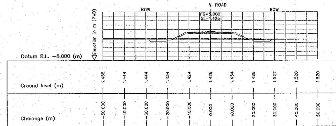
6 CROSS SECTION (STA. 5750.000) E-16 SCALE 1:500
