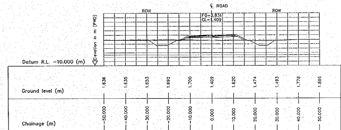
5 CROSS SECTION (STA. 6600.000) E-19 SCALE 1:500
