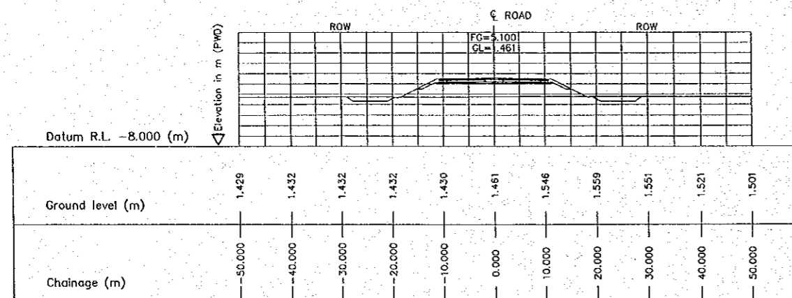
1 CROSS SECTION (STA. 5800.000) E-17 SCALE 1:500
