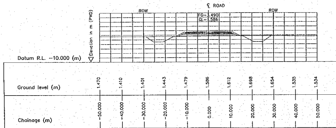
3 CROSS SECTION (STA. 4100.000) E-11 SCALE 1:500
