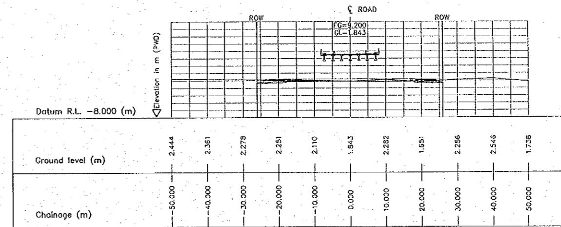
6 CROSS SECTION (STA. 6950.000) E-20 SCALE 1:500
