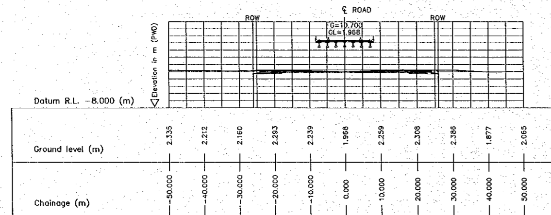
1 CROSS SECTION (STA. 7000.000) E-21 SCALE 1:500
