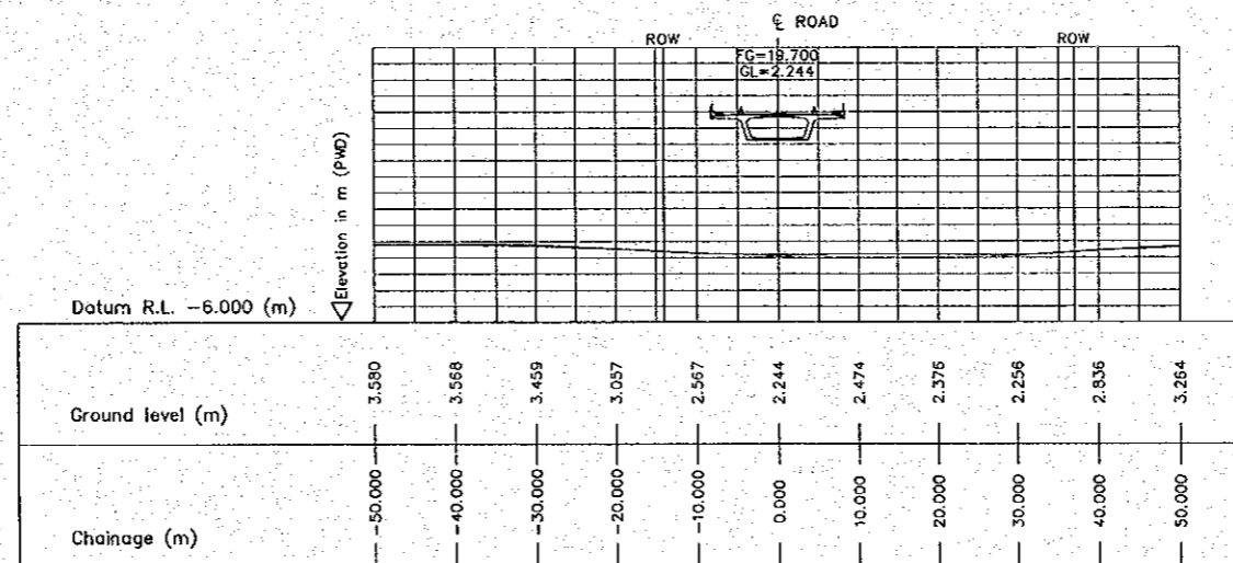
1 CROSS SECTION (STA. 7300.000) E-22 SCALE 1:500
