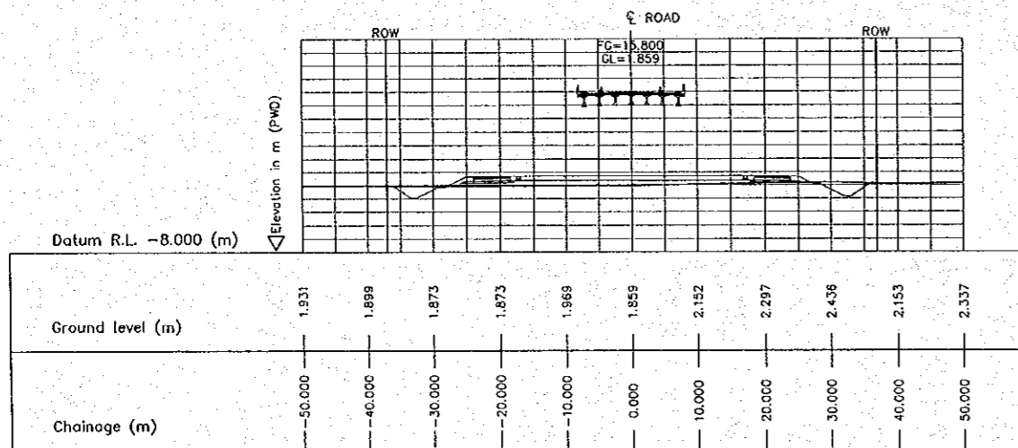
2 CROSS SECTION (STA. 7950.000) E-23 SCALE 1:500
