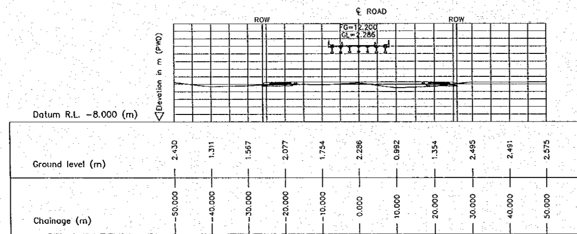
3 CROSS SECTION (STA. 7100.000) E-21 SCALE 1:500
