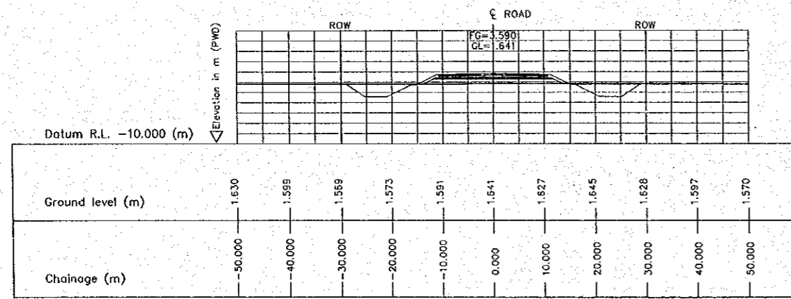
2 CROSS SECTION (STA. 4050.000) E-11 SCALE 1:500
