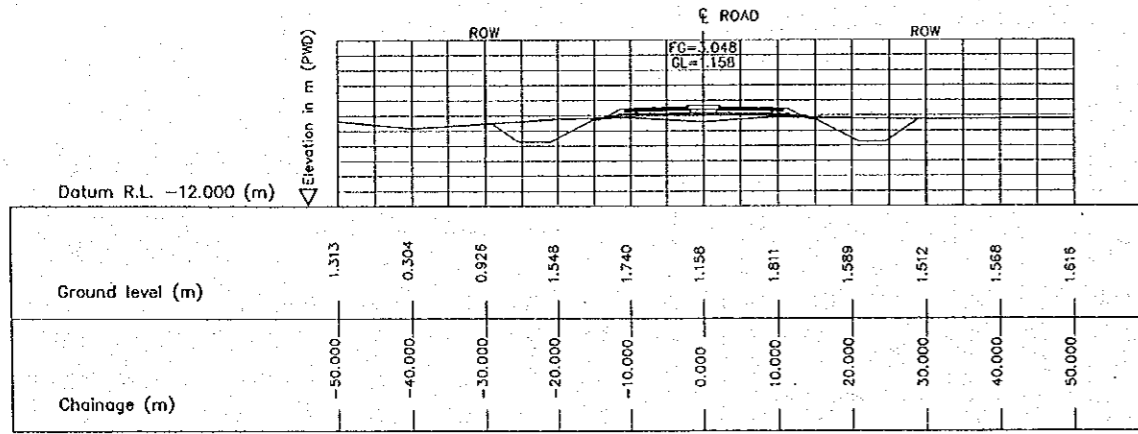
3 CROSS SECTION (STA. 1100.000) E-01 SCALE 1:1000
