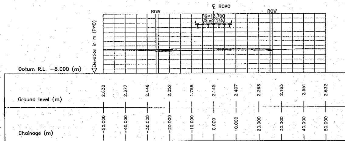
3 CROSS SECTION (STA. 7100.000) E-21 SCALE 1:500
