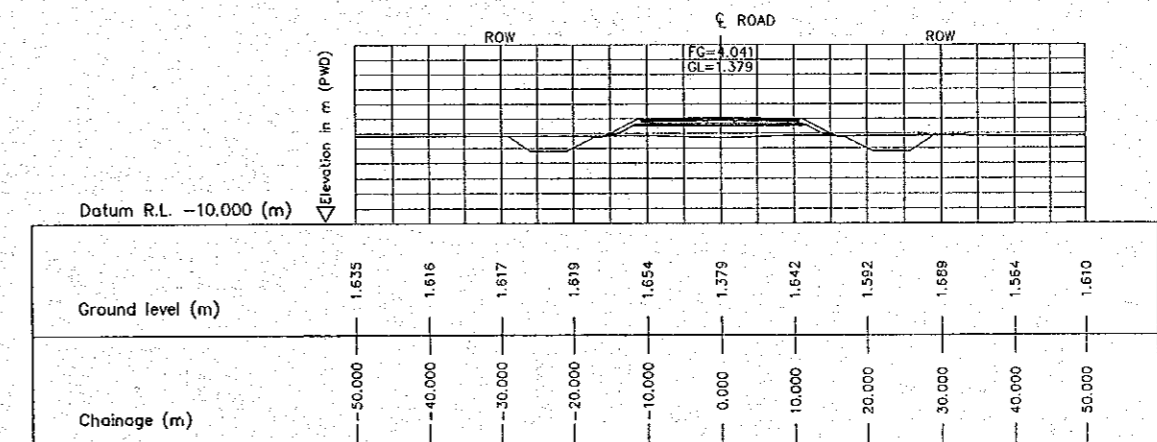
4 CROSS SECTION (STA. 6550.000) E-19 SCALE 1:500
