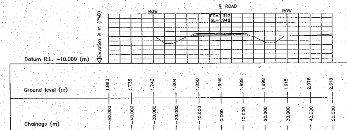
4 CROSS SECTION (STA. 3250.000) E-08 SCALE 1:500
