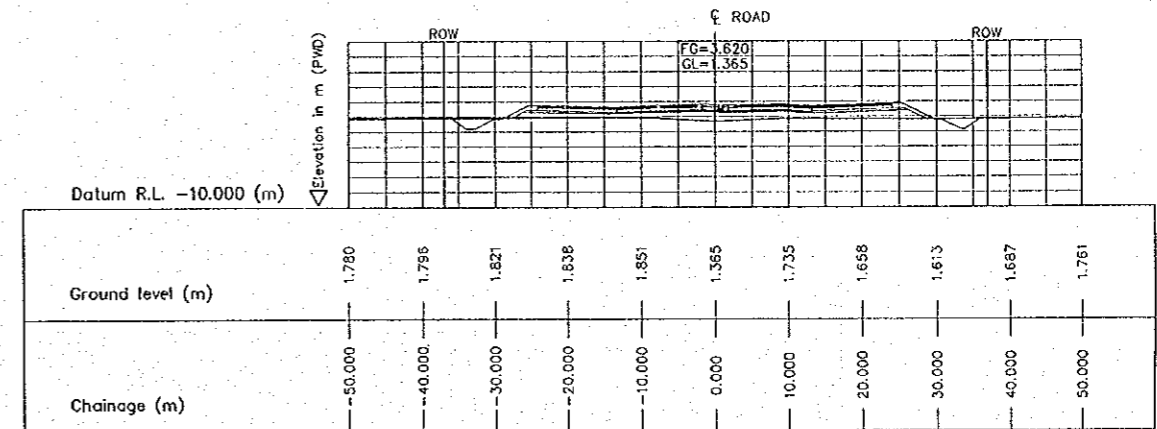
6 CROSS SECTION (STA. 6650.000) E-19 SCALE 1:500
