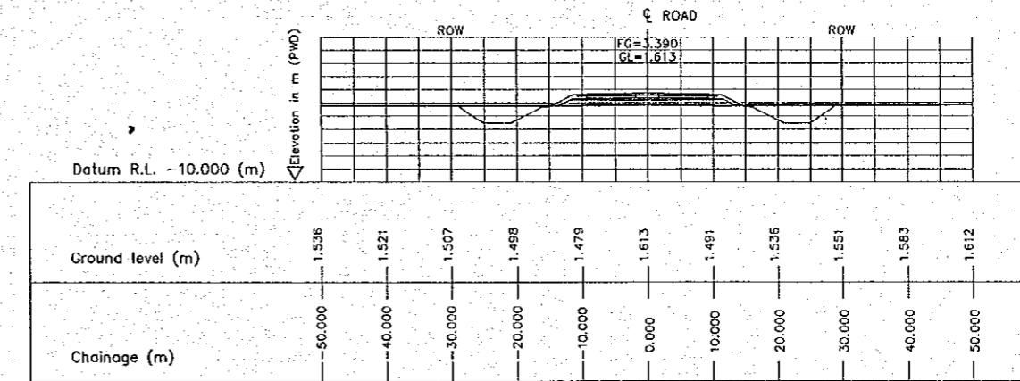
4 CROSS SECTION (STA. 4150.000) E-11 SCALE 1:500
