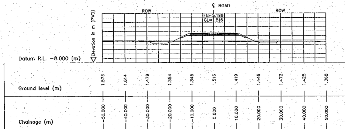
2 CROSS SECTION (STA. 5850.000) E-17 SCALE 1:500
