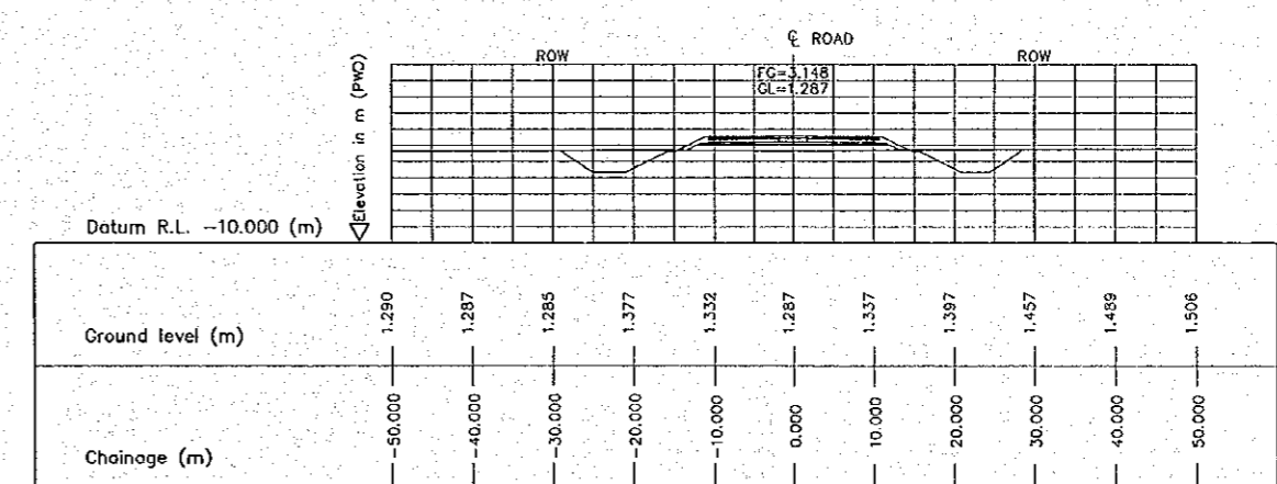
4 CROSS SECTION (STA. 1150.000) E-01 SCALE 1:1000
