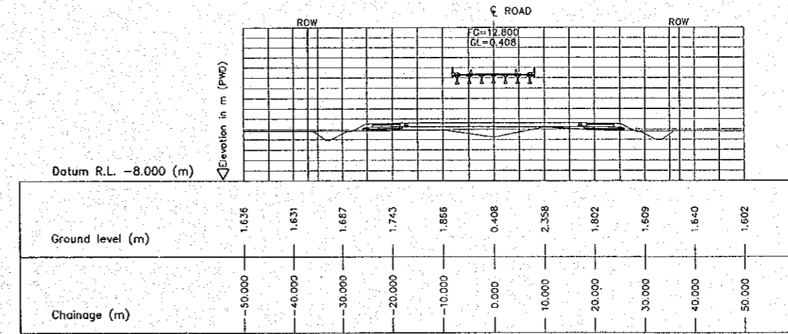
4 CROSS SECTION (STA. 8050.000) E-23 SCALE 1:500
