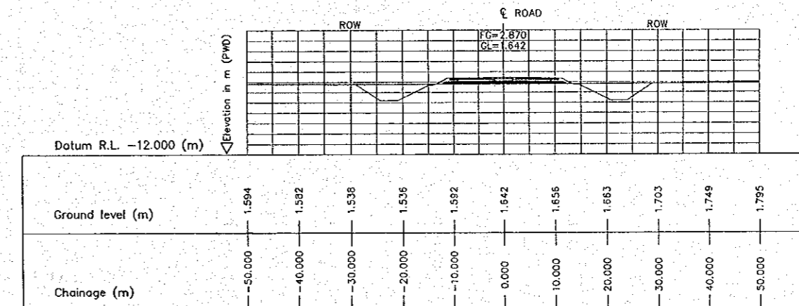
4 CROSS SECTION (STA. 4450.000) E-12 SCALE 1:500
