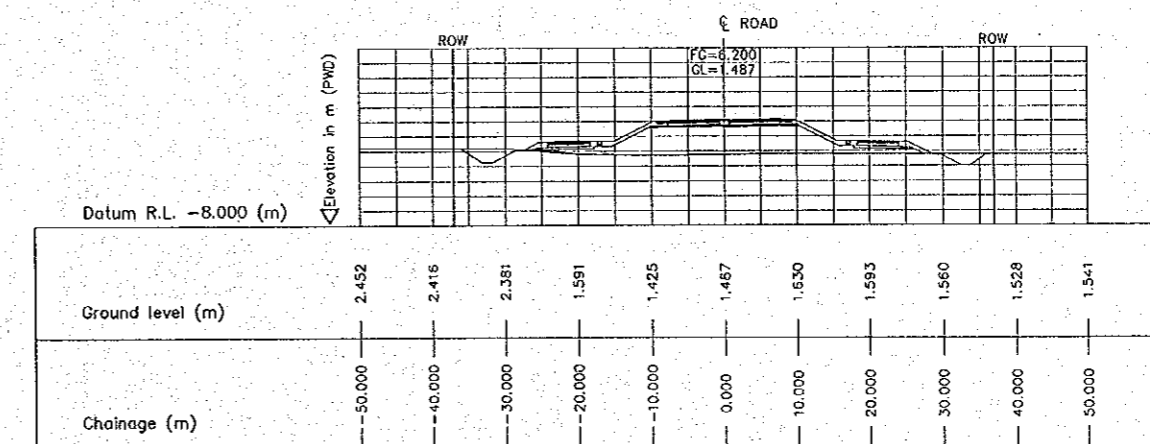
4 CROSS SECTION (STA. 6850.000) E-20 SCALE 1:500
