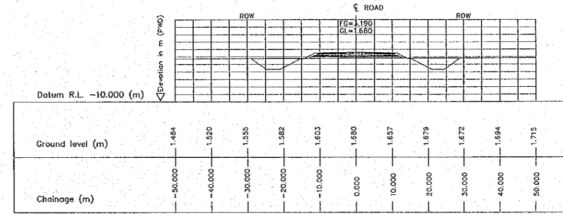
6 CROSS SECTION (STA. 4250.000) E-11 SCALE 1:500
