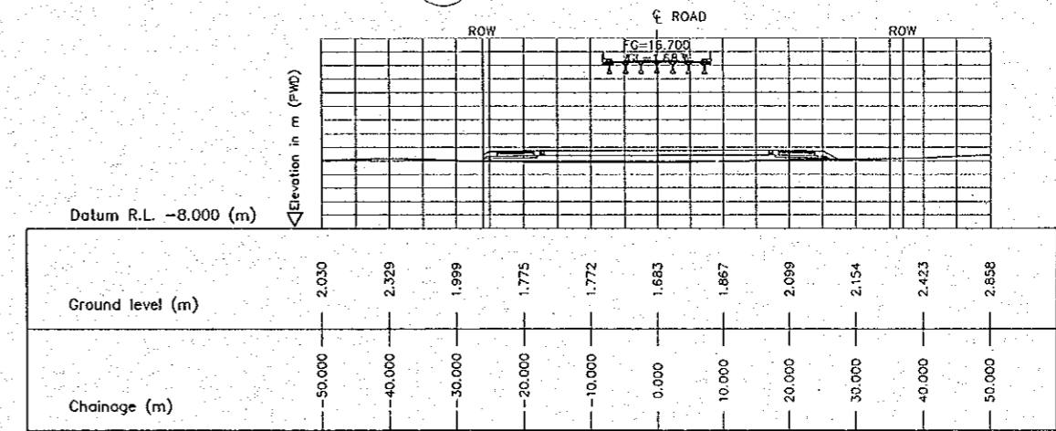
6 CROSS SECTION (STA. 7250.000) E-21 SCALE 1:500
