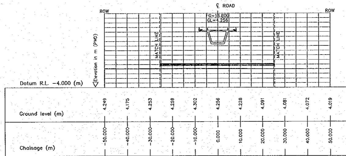
2 CROSS SECTION (STA. 7850.000) E-22 SCALE 1:500
