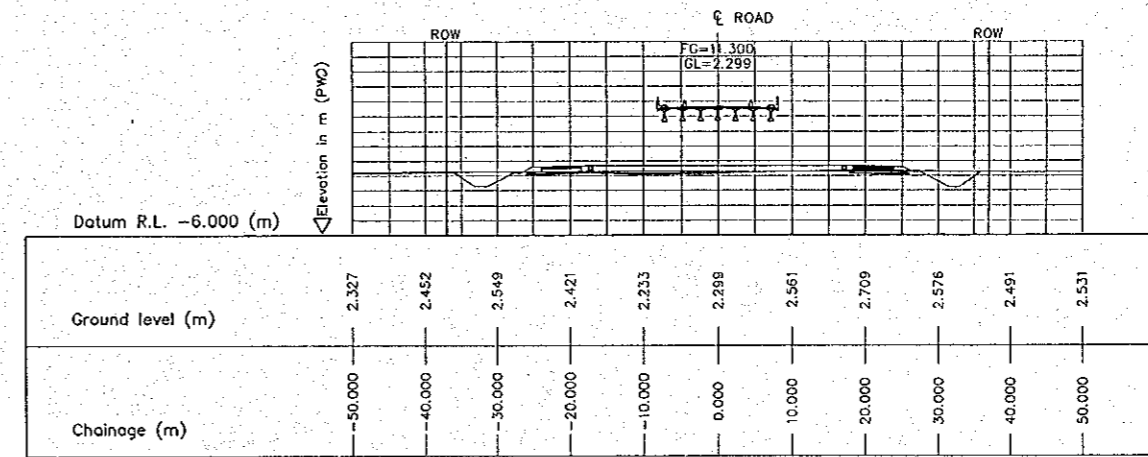
5 CROSS SECTION (STA. 8100.000) E-23 SCALE 1:500
