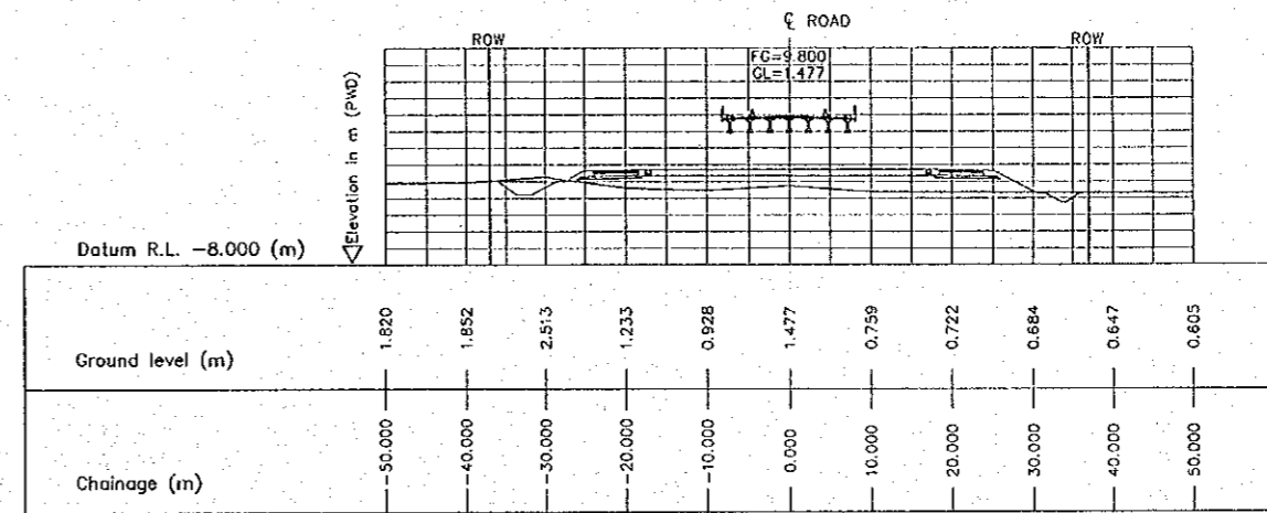
6 CROSS SECTION (STA. 8150.000) E-23 SCALE 1:500
