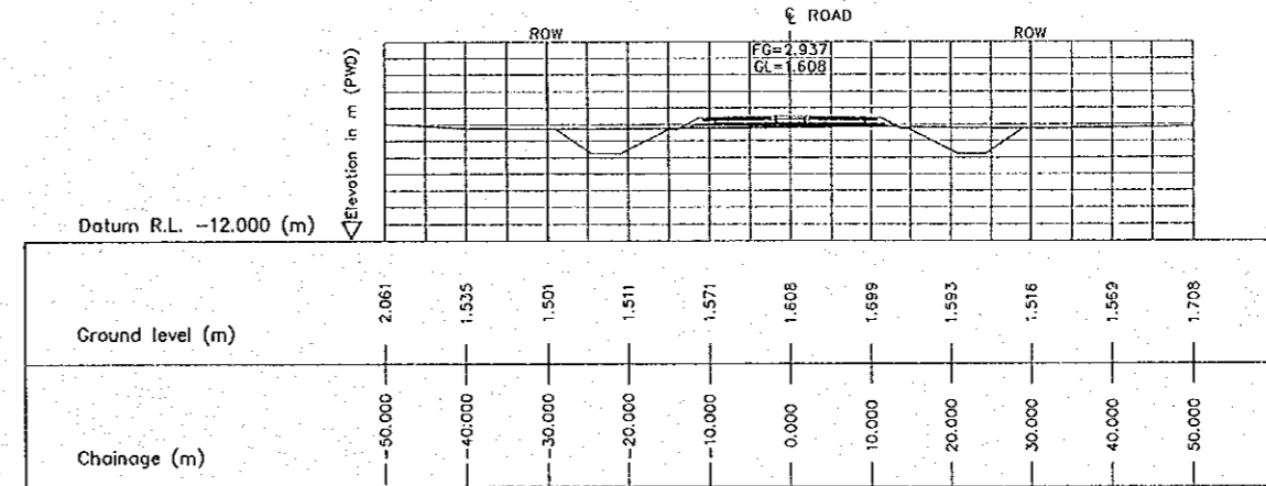
6 CROSS SECTION (STA. 6050.000) E-17 SCALE 1:500
