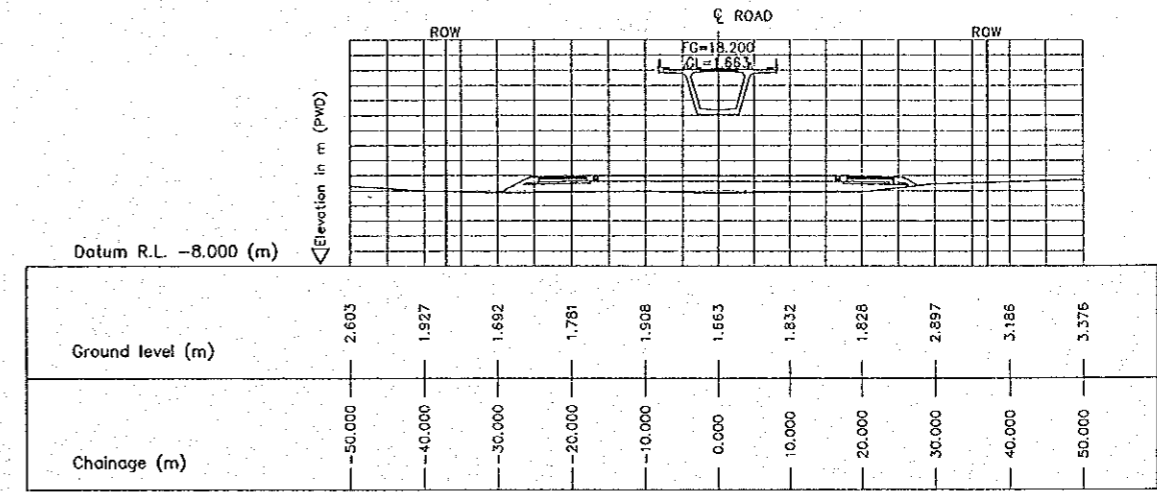
6 CROSS SECTION (STA. 7250.000) E-21 SCALE 1:500
