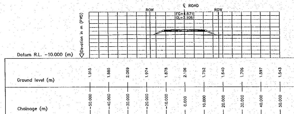
1 CROSS SECTION (STA. 6400.000) E-19 SCALE 1:500
