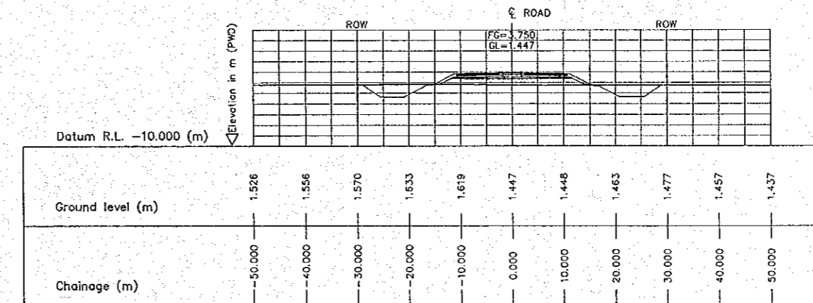
4 CROSS SECTION (STA. 5350.000) E-15 SCALE 1:500
