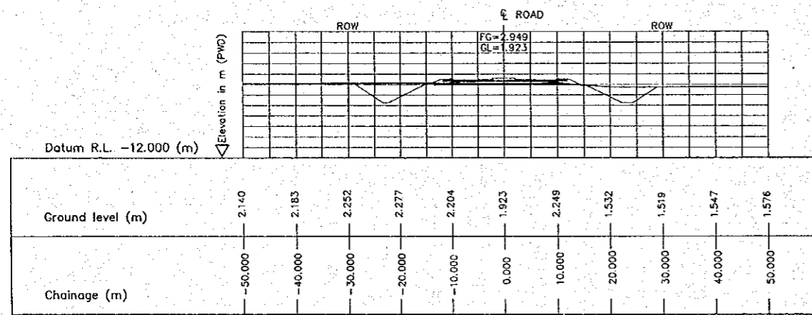
2 CROSS SECTION (STA. 1050.000) E-01 SCALE 1:1000
