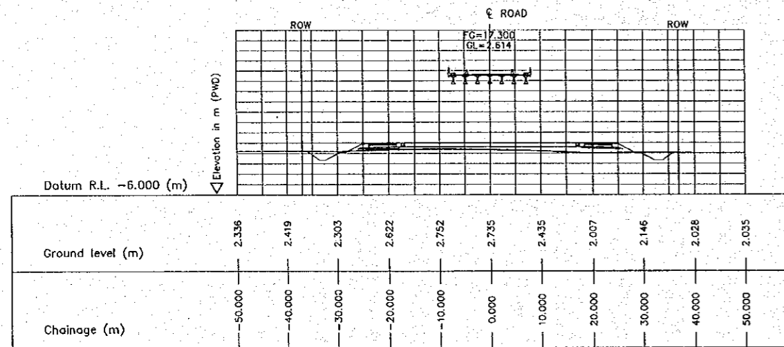
1 CROSS SECTION (STA. 7900.000) E-23 SCALE 1:500
