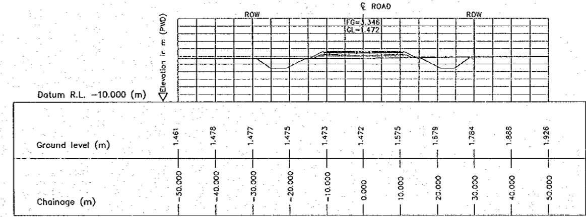
6 CROSS SECTION (STA. 1250.000) E-01 SCALE 1:1000
