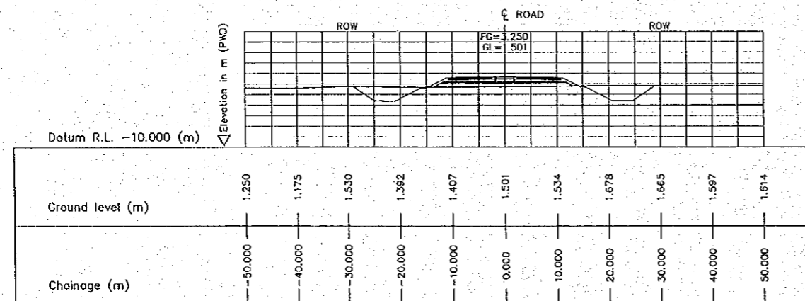
1 CROSS SECTION (STA. 6100.000) E-18 SCALE 1:500
