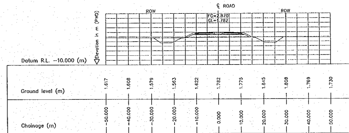
6 CROSS SECTION (STA. 4550.000) E-12 SCALE 1:500
