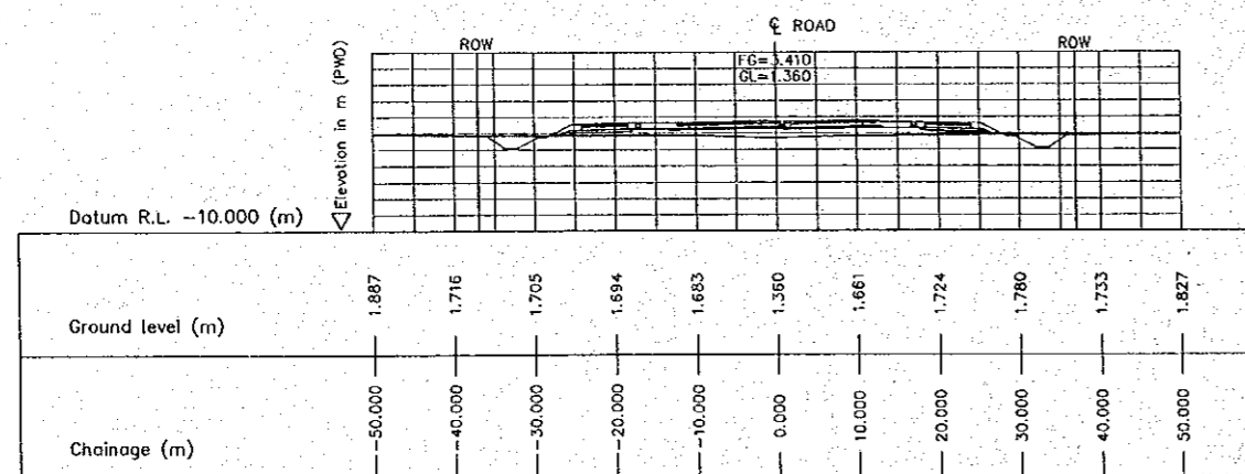
1 CROSS SECTION (STA. 6700.000) E-20 SCALE 1:500
