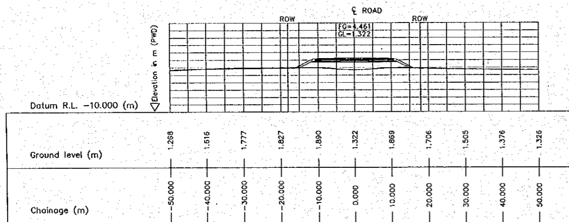
2 CROSS SECTION (STA. 6450.000) E-19 SCALE 1:500
