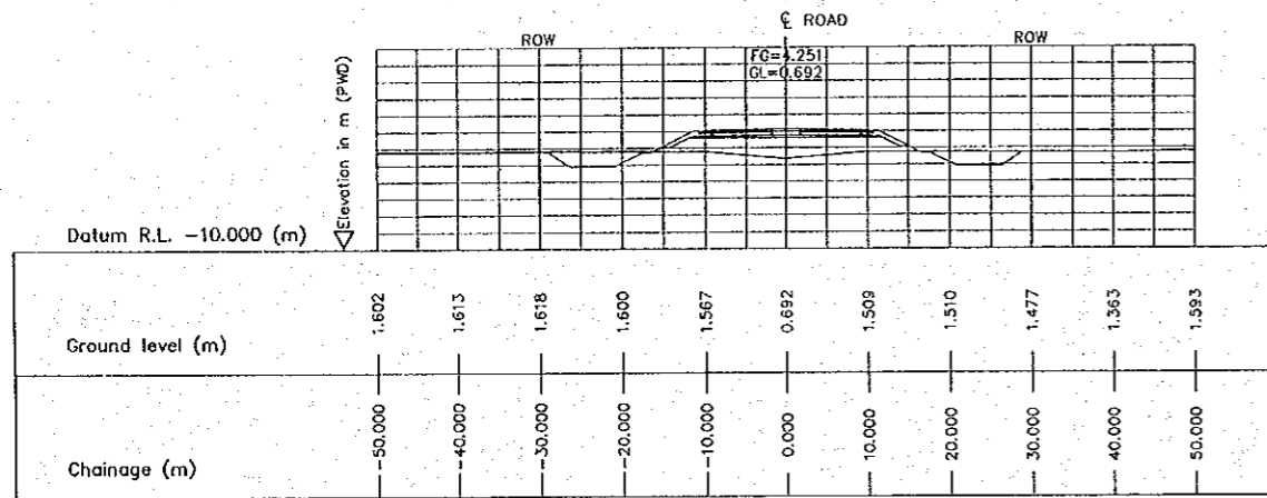
3 CROSS SECTION (STA. 6500.000) E-19 SCALE 1:500
