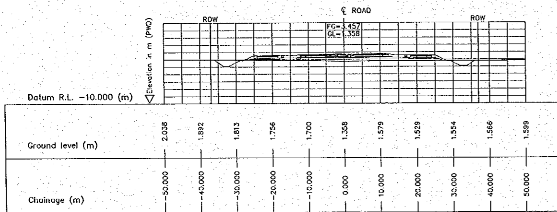
2 CROSS SECTION (STA. 6750.000) E-20 SCALE 1:500
