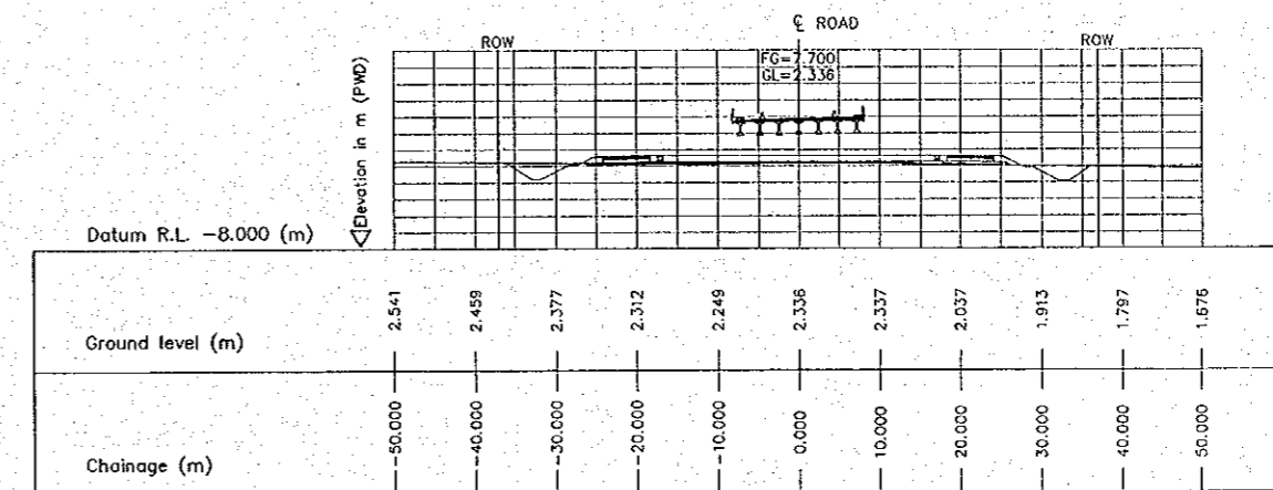
6 CROSS SECTION (STA. 6950.000) E-20 SCALE 1:500
