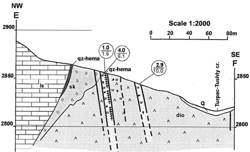
Appendix 13 Geological Cross Section of the Turpac-Tushty Ore Manifestation (C-D, E-F)
