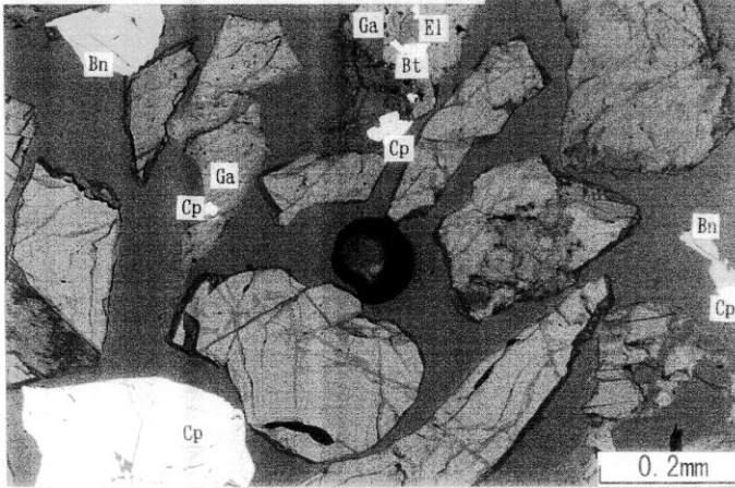
Heavy minerals by shaking table (transmitted light)
