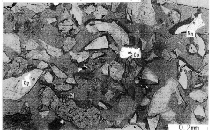
Medium minerals by shaking table (reflected light)
