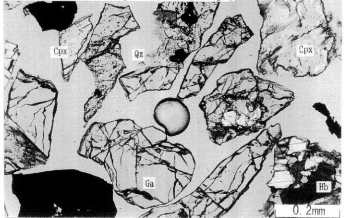
Heavy minerals by shaking table (reflected light)
