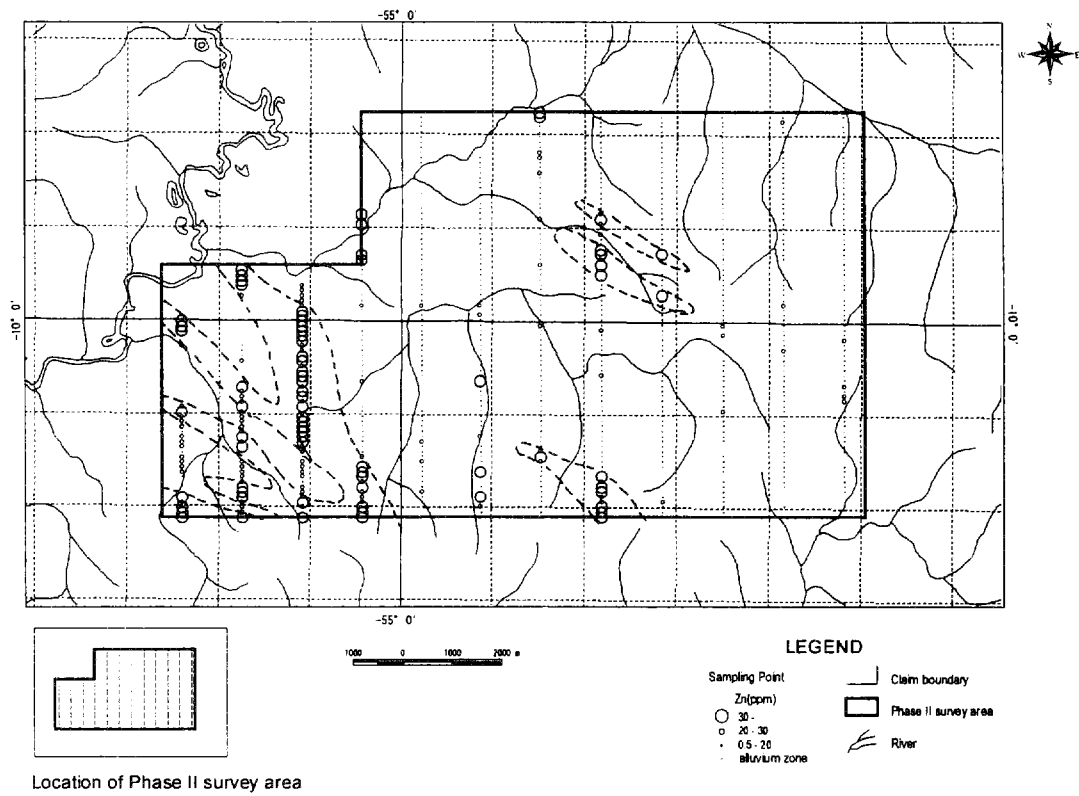
Distribution map of Zn anomalies in Block F
