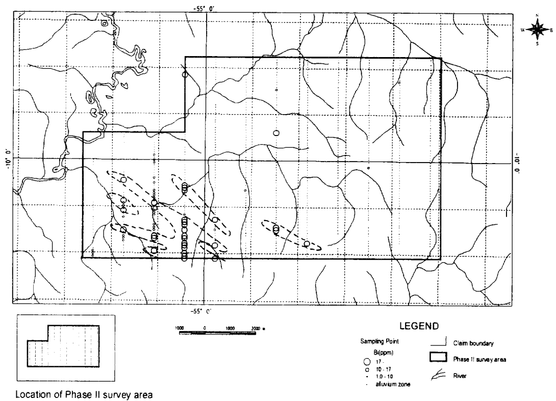
Distribution map of Bi anomalies in Block F
