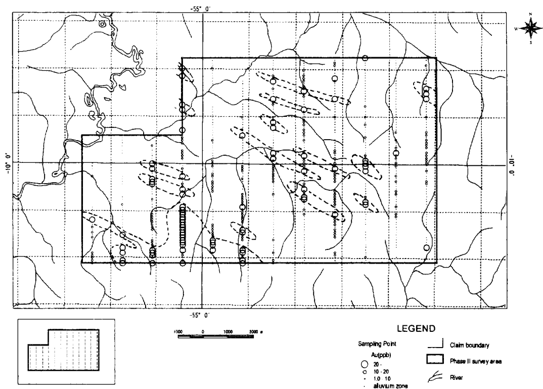
Distribution map of Au anomalies in Block F
