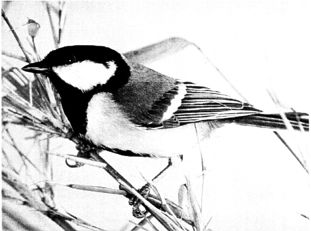
Figure 13-26: Parus Major
