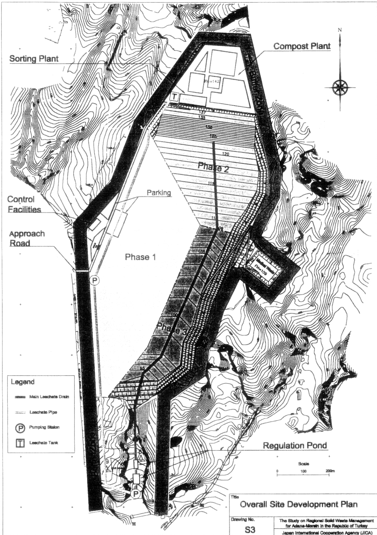
Figure 13-3: Location of Solid Waste Management Facilities
