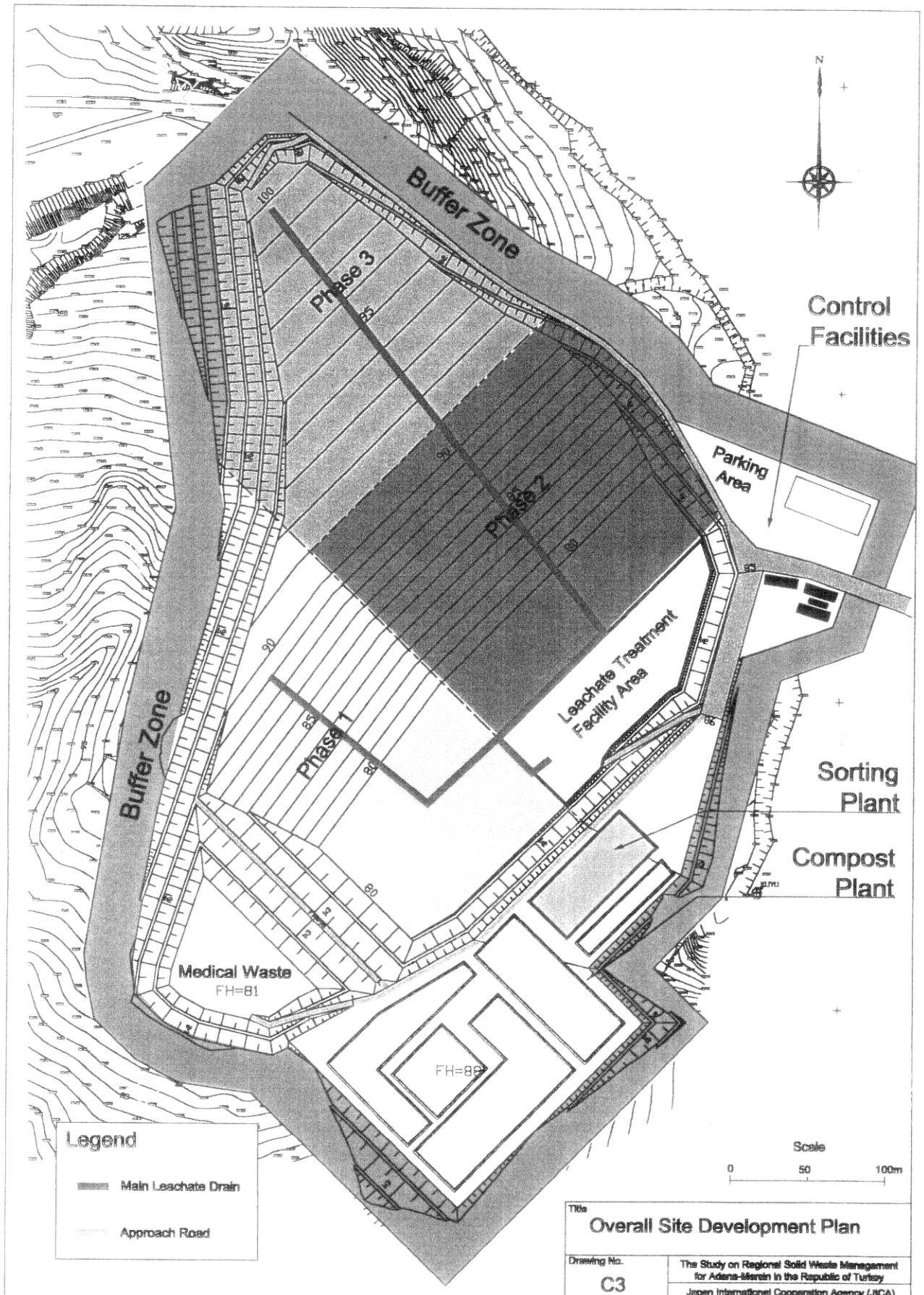
Plate 11 : Cimsa Overall Site Development Plan
