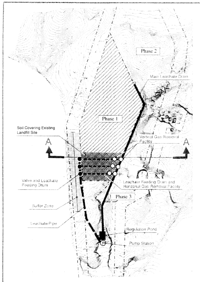
Plan of experiment on the Sofulu disposal site improvement
