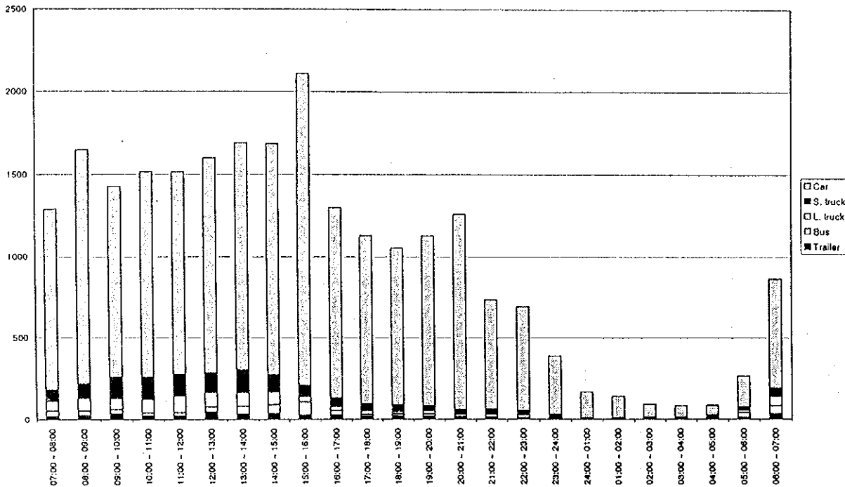
Figure D4.27(114) Hourly Traffic Volume by Vehicle Type - Measuring Point 57 (22/23.04.1998 - weekday)
