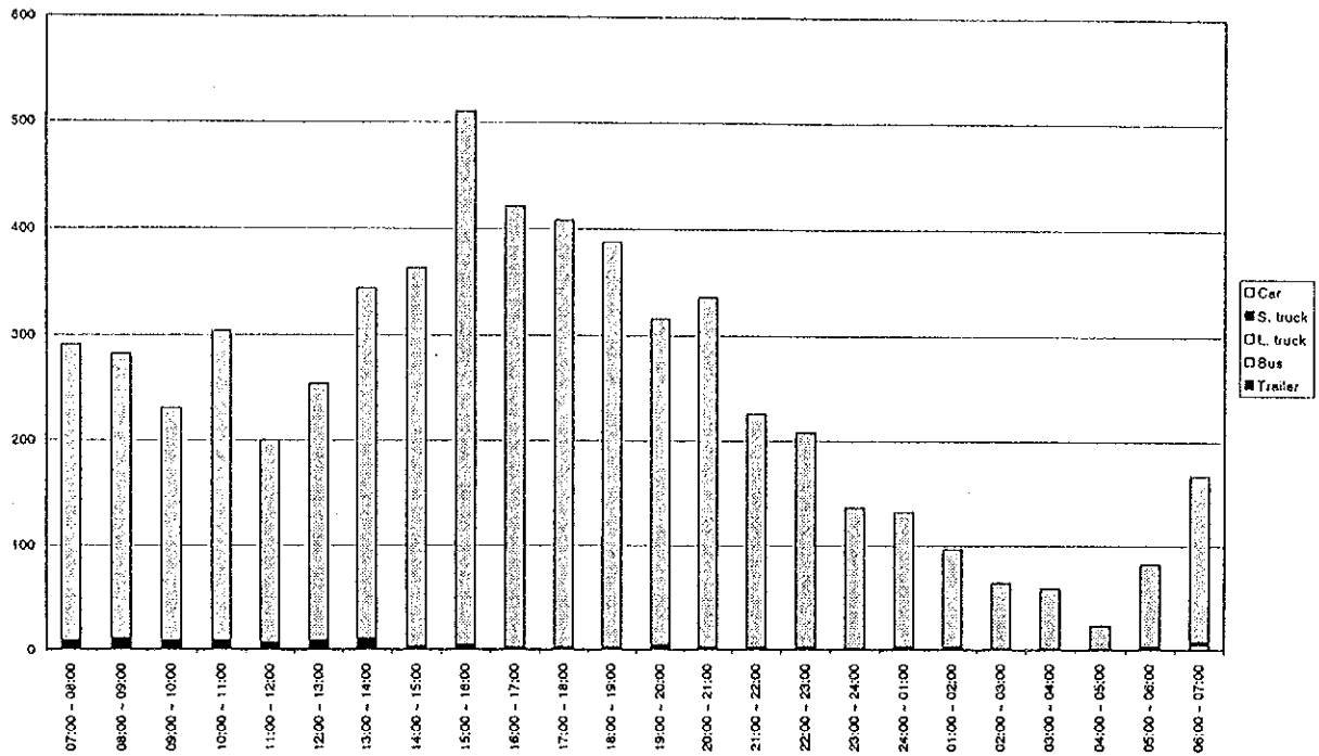
Figure D4.27(137) Hourly Traffic Volume by Vehicle Type - Measuring Point 69 (22/23.04.1998 - weekday)
