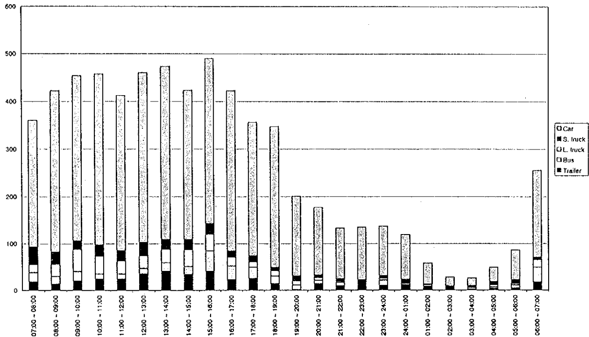
Figure D4.27(147) Hourly Traffic Volume by Vehicle Type - Measuring Point 74 (22/23.04.1998 - weekday)
