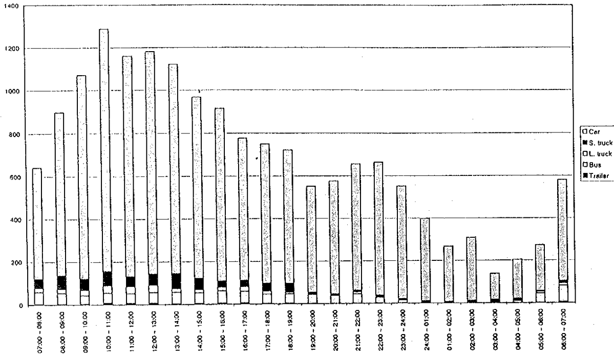
Figure D4.27(134) Hourly Traffic Volume by Vehicle Type - Measuring Point 67 (25/25.04.1998 - holiday)
