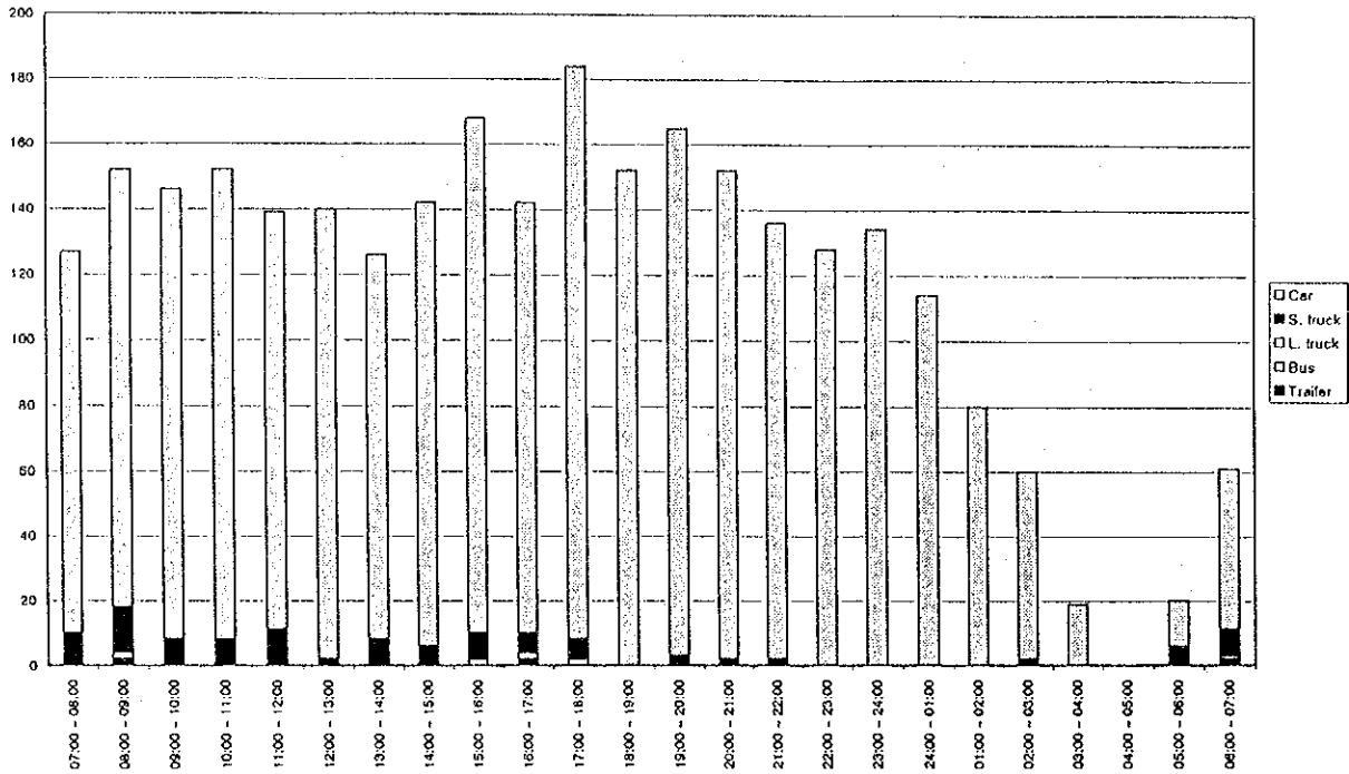
Figure D4.27(136) Hourly Traffic Volume by Vehicle Type - Measuring Point 68 (25/25.04.1998 - holiday)
