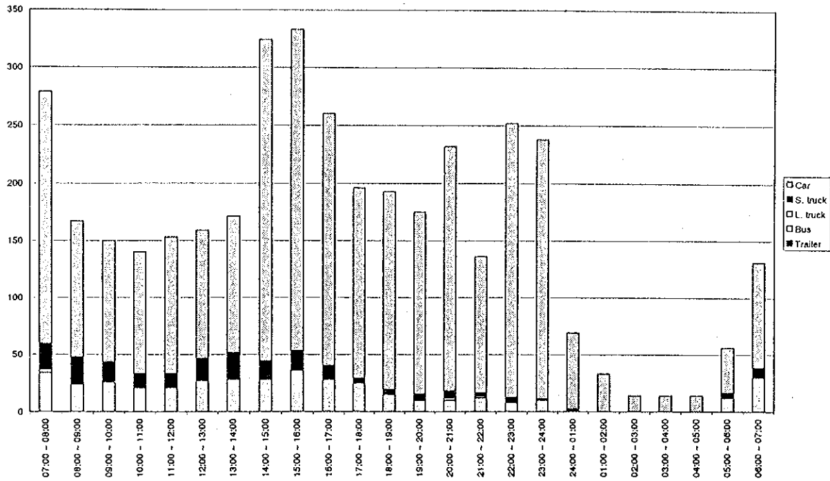
Figure D4.27(141) Hourly Traffic Volume by Vehicle Type - Measuring Point 71 (22/23.04.1998 - weekday)
