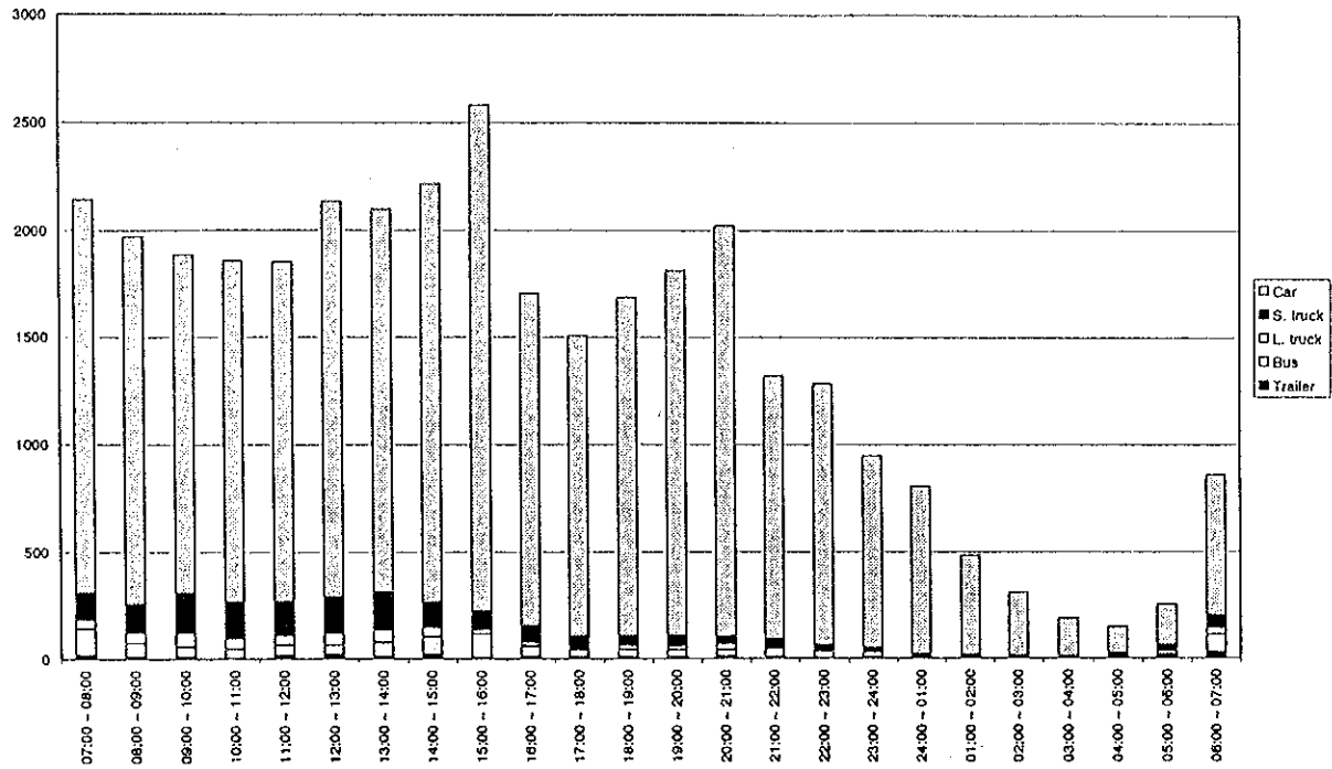
Figure D4.27(143) Hourly Traffic Volume by Vehicle Type - Measuring Point 72 (22/23.04.1998 - weekday)
