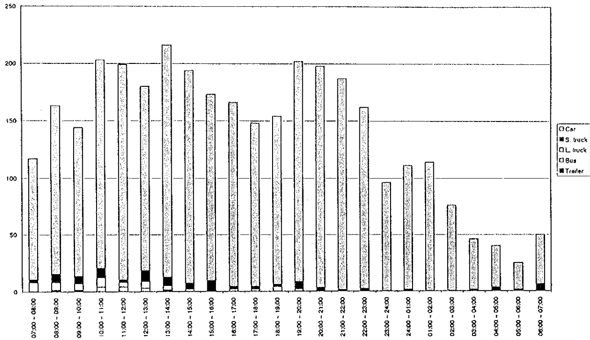
Figure D4.27(113) Hourly Traffic Volume by Vehicle Type - Measuring Point 56 (25/25.04.1998 - holiday)
