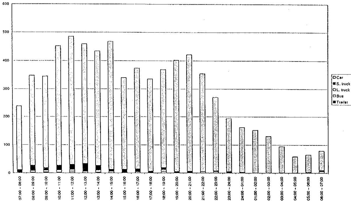
Figure D4.27(122) Hourly Traffic Volume by Vehicle Type - Measuring Point 61 (25/25.04.1998 - holiday)
