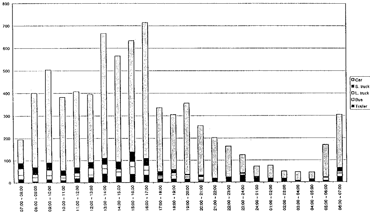
Figure D4.27(148) Hourly Traffic Volume by Vehicle Type - Measuring Point 75 (22/23.04.1998 - weekday)
