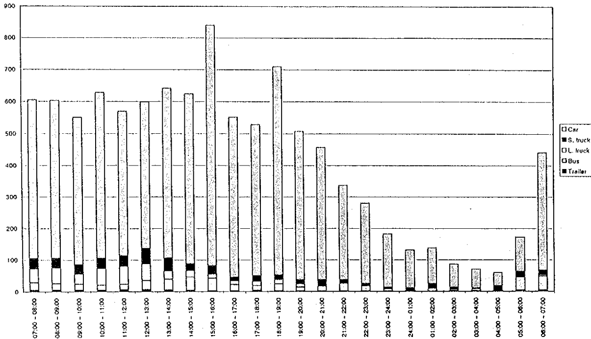
Figure D4.27(118) Hourly Traffic Volume by Vehicle Type - Measuring Point 59 (22/23.04.1998 - weekday)
