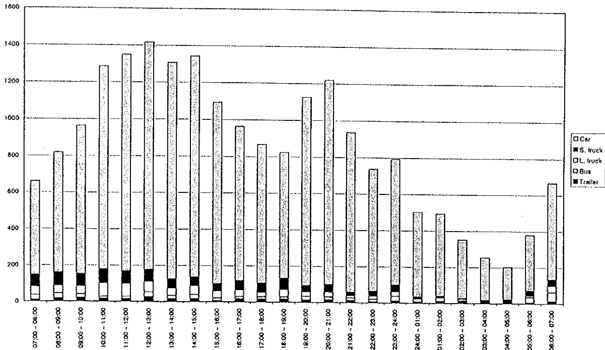
Figure D4.27(115) Hourly Traffic Volume by Vehicle Type - Measuring Point 57 (25/25.04.1998 - holiday)
