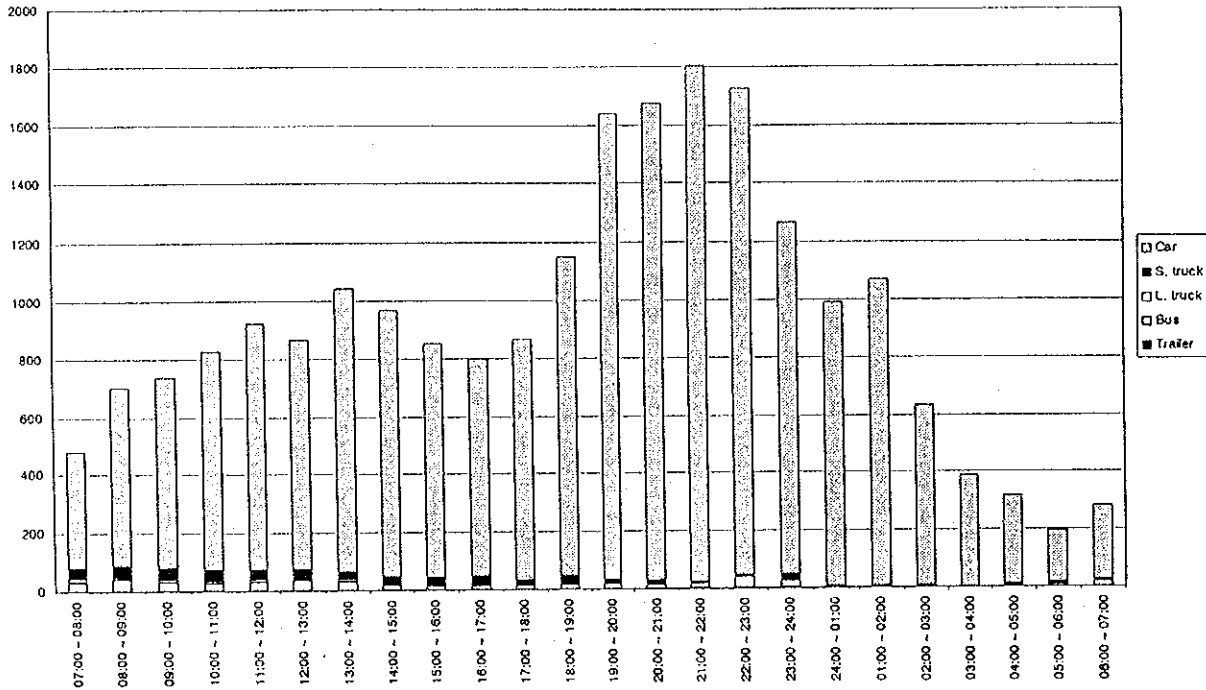
Figure D4.27(140) Hourly Traffic Volume by Vehicle Type - Measuring Point 70 (25/26.04.1998 - holiday)
