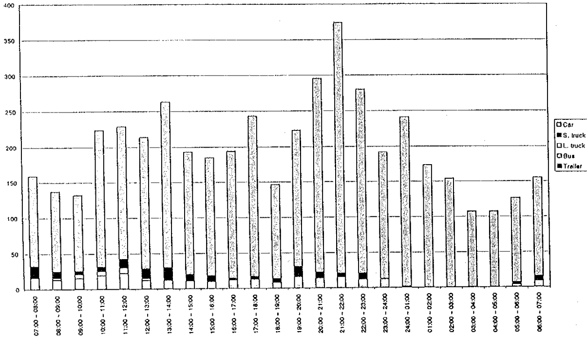
Figure D4.27(142) Hourly Traffic Volume by Vehicle Type - Measuring Point 71 (25/25.04.1998 - holiday)
