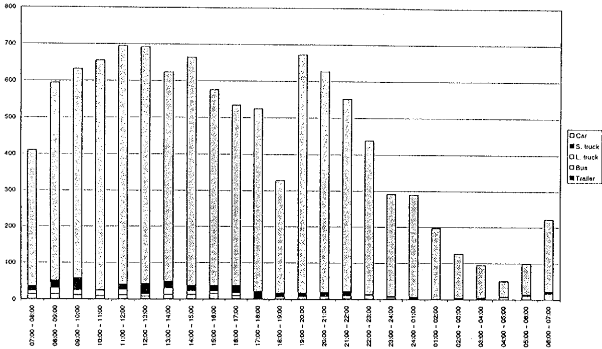
Figure D4.27(117) Hourly Traffic Volume by Vehicle Type - Measuring Point 58 (25/25.04.1998 - holiday)
