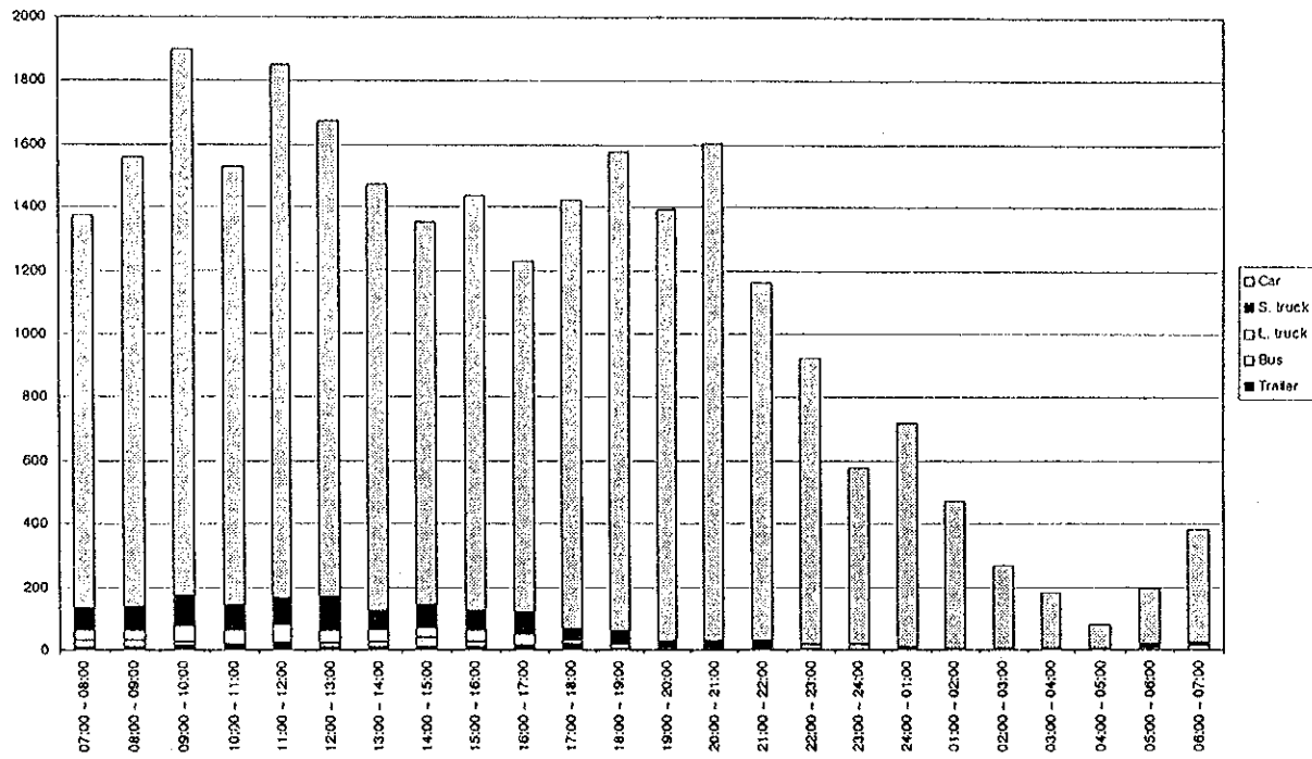
Figure D4.27(111) Hourly Traffic Volume by Vehicle Type - Measuring Point 55 (25/25.04.1998 - holiday)
