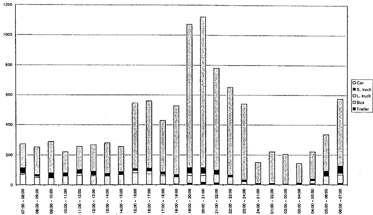
Figure D4.27(131) Hourly Traffic Volume by Vehicle Type - Measuring Point 66 (22/23.04.1998 - weekday)
