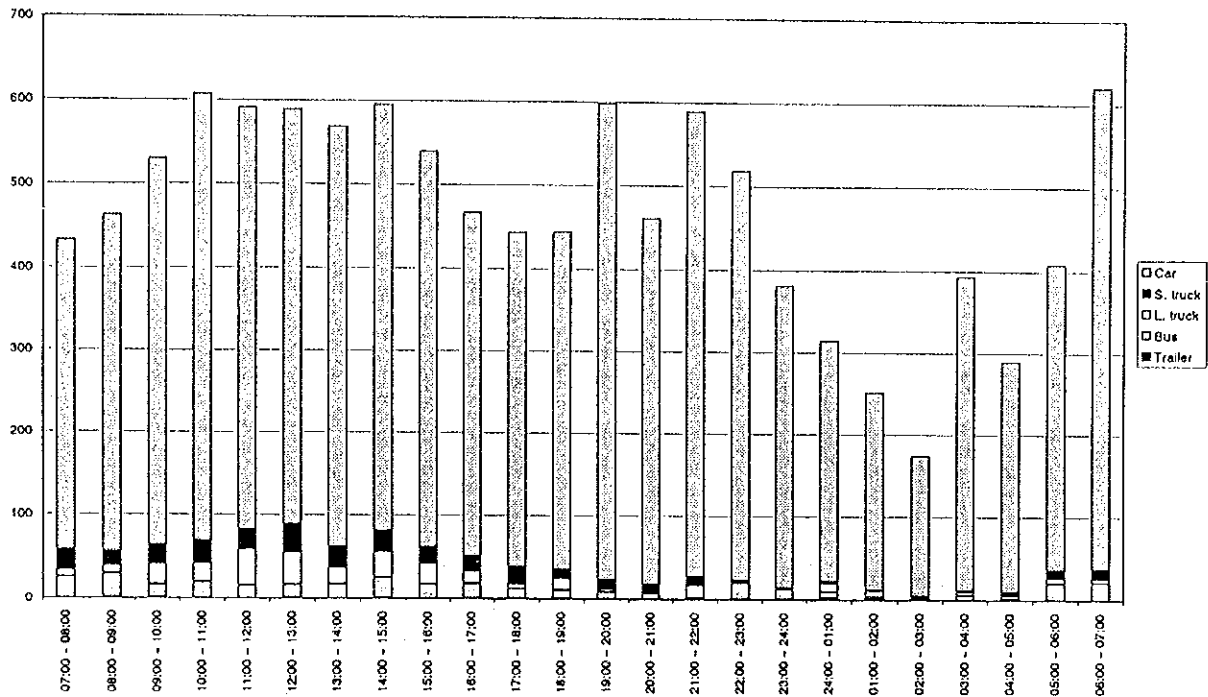
Figure D4.27(119) Hourly Traffic Volume by Vehicle Type - Measuring Point 59 (25/25.04.1998 - holiday)
