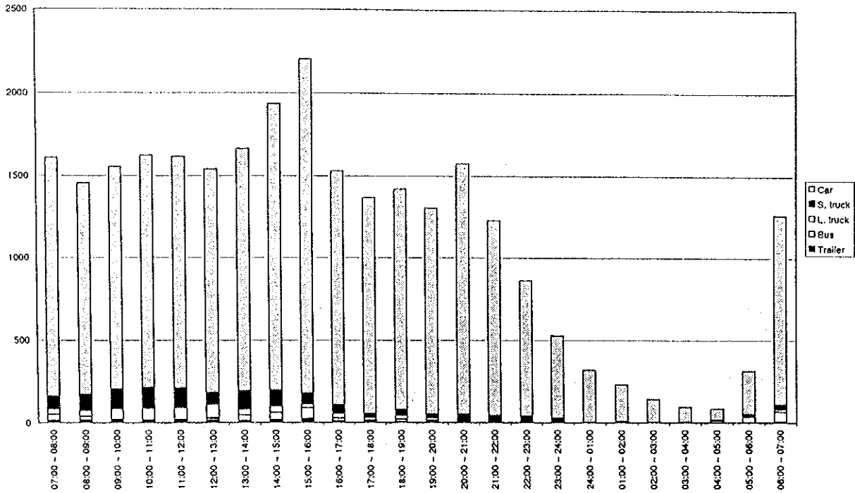
Figure D4.27(110) Hourly Traffic Volume by Vehicle Type - Measuring Point 55 (22/23.04.1998 - weekday)
