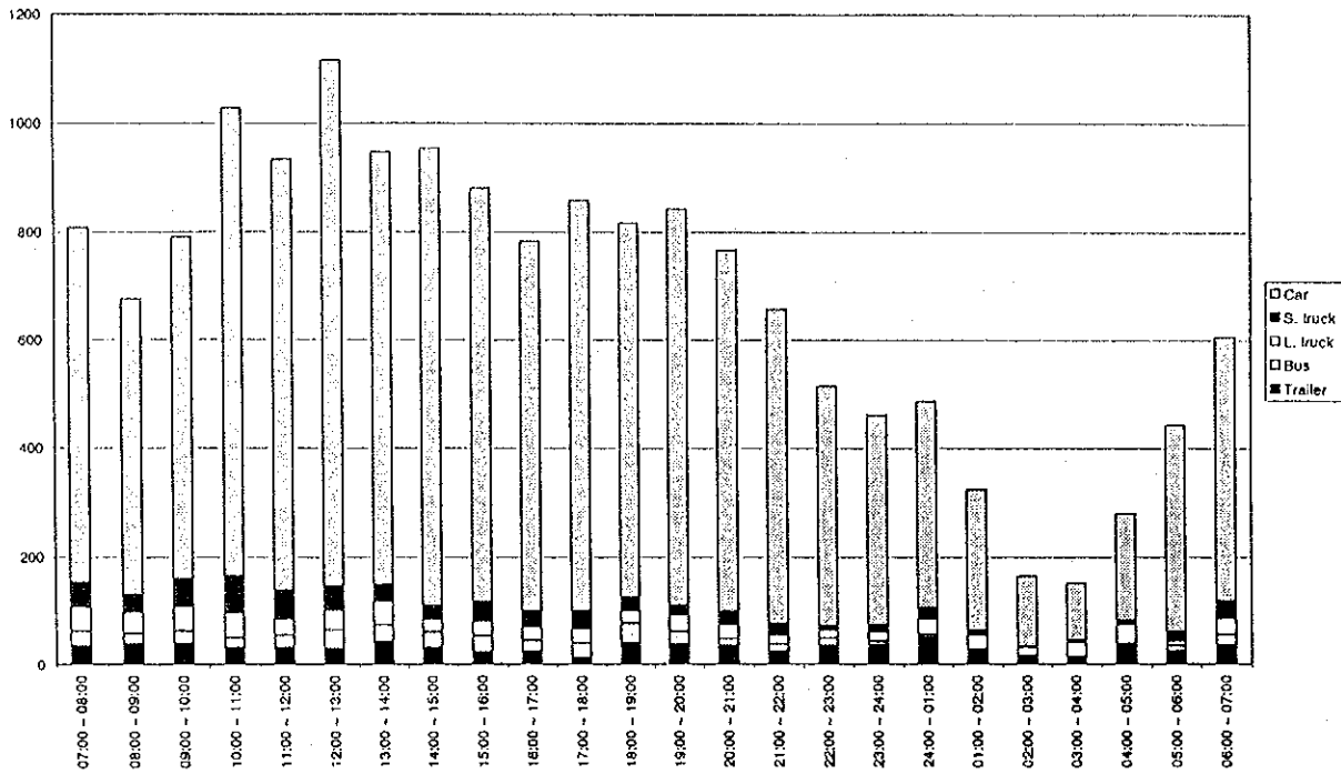
Figure D4.27(146) Hourly Traffic Volume by Vehicle Type - Measuring Point 73 (25/25.04.1998 - holiday)
