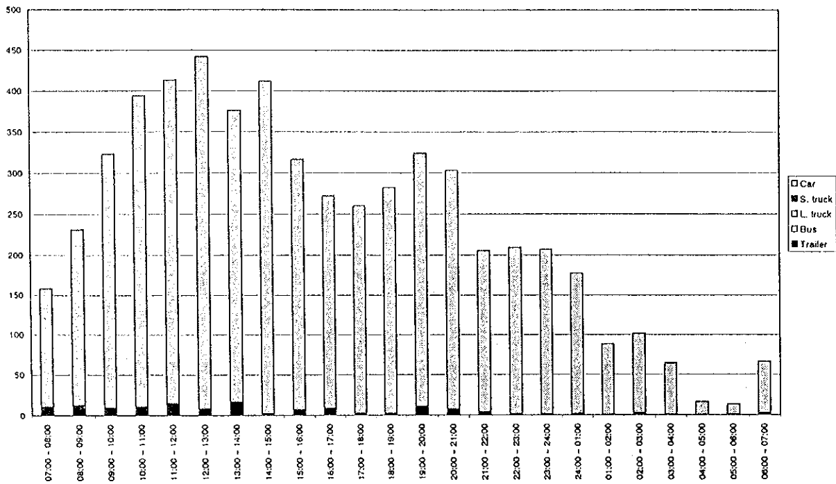
Figure D4.27(126) Hourly Traffic Volume by Vehicle Type - Measuring Point 63 (25/25.04.1998 - holiday)
