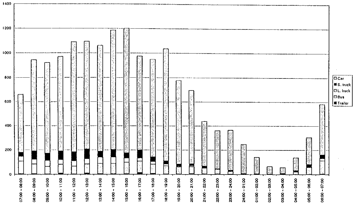
Figure D4.27(133) Hourly Traffic Volume by Vehicle Type - Measuring Point 67 (22/23.04.1998 - weekday)
