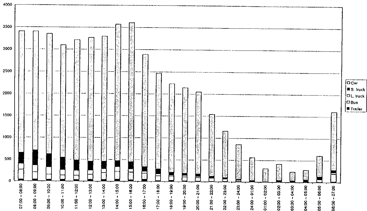
Figure D4.27(129) Hourly Traffic Volume by Vehicle Type - Measuring Point 65 (22/23.04.1998 - weekday)
