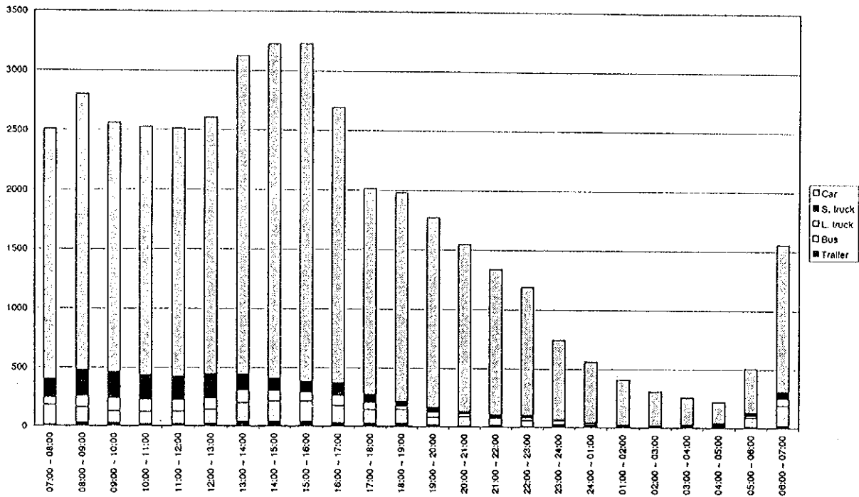
Figure D4.27(127) Hourly Traffic Volume by Vehicle Type - Measuring Point 64 (22/23.04.1998 - weekday)
