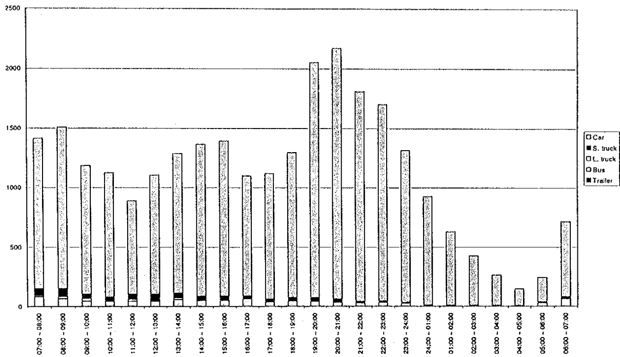
Figure D4.27(139) Hourly Traffic Volume by Vehicle Type - Measuring Point 70 (22/23.04.1998 - weekday)
