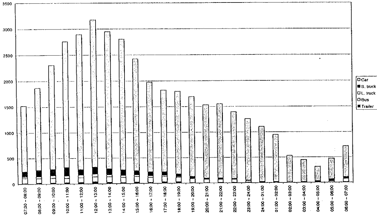
Figure D4.27(130) Hourly Traffic Volume by Vehicle Type - Measuring Point 65 (25/25.04.1998 - holiday)
