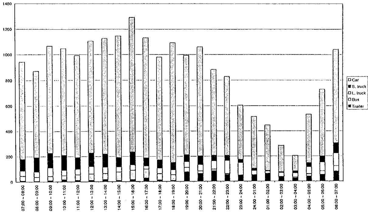
Figure D4.27(145) Hourly Traffic Volume by Vehicle Type - Measuring Point 73 (22/23.04.1998 - weekday)
