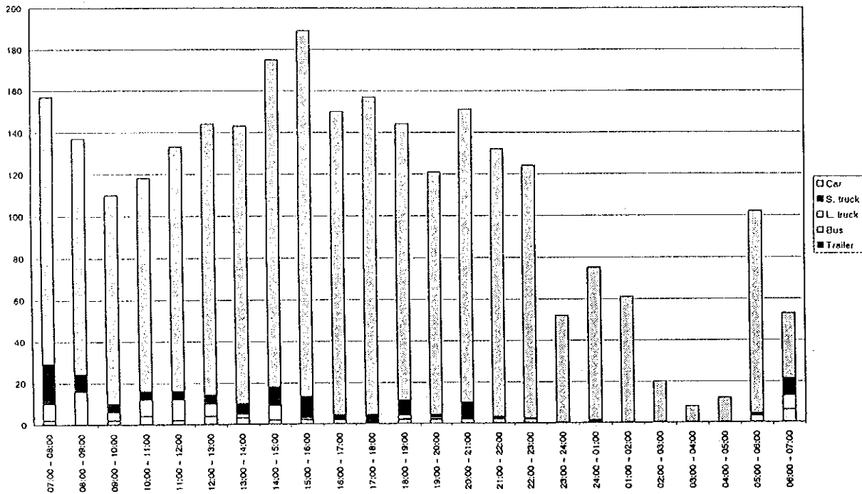
Figure D4.27(112) Hourly Traffic Volume by Vehicle Type - Measuring Point 5G (22/23.04.1998 - weekday)
