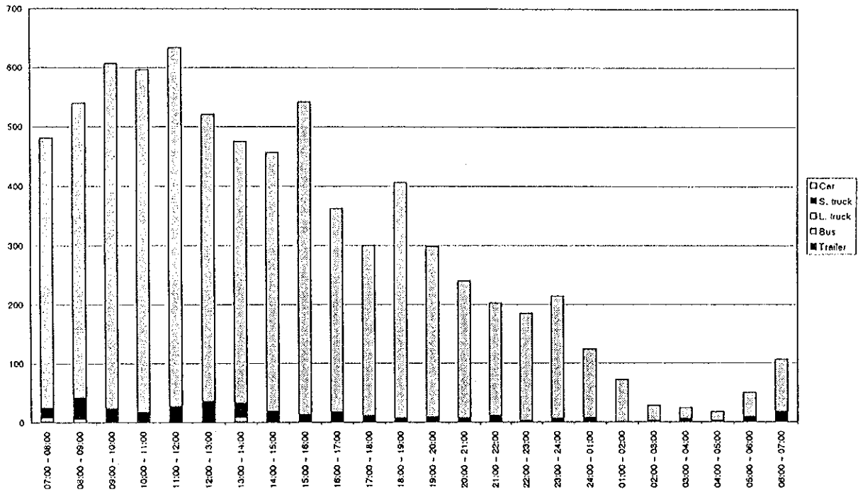
Figure D4.27(125) Hourly Traffic Volume by Vehicle Type - Measuring Point 63 (22/23.04.1998 - weekday)
