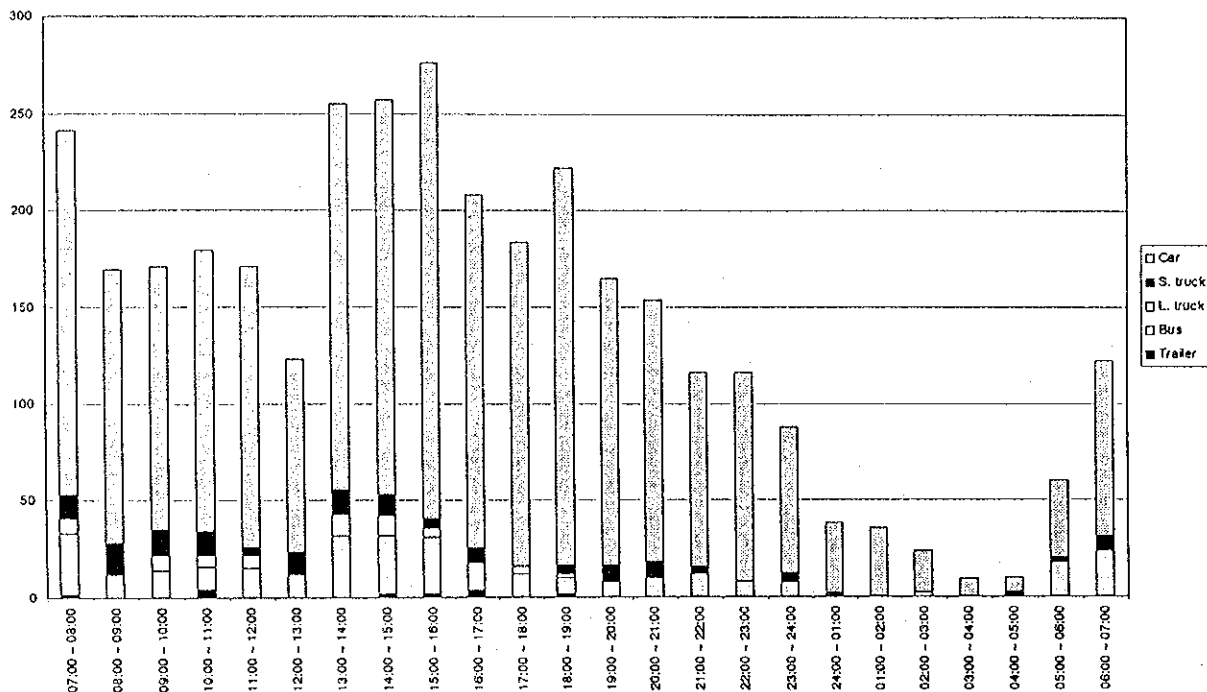
Figure D4.27(120) Hourly Traffic Volume by Vehicle Type - Measuring Point 60 (22/23.04.1998 - weekday)
