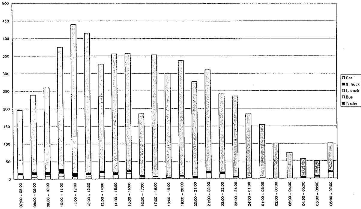
Figure D4.27(124) Hourly Traffic Volume by Vehicle Type - Measuring Point 62 (25/25.04.1998 - holiday)
