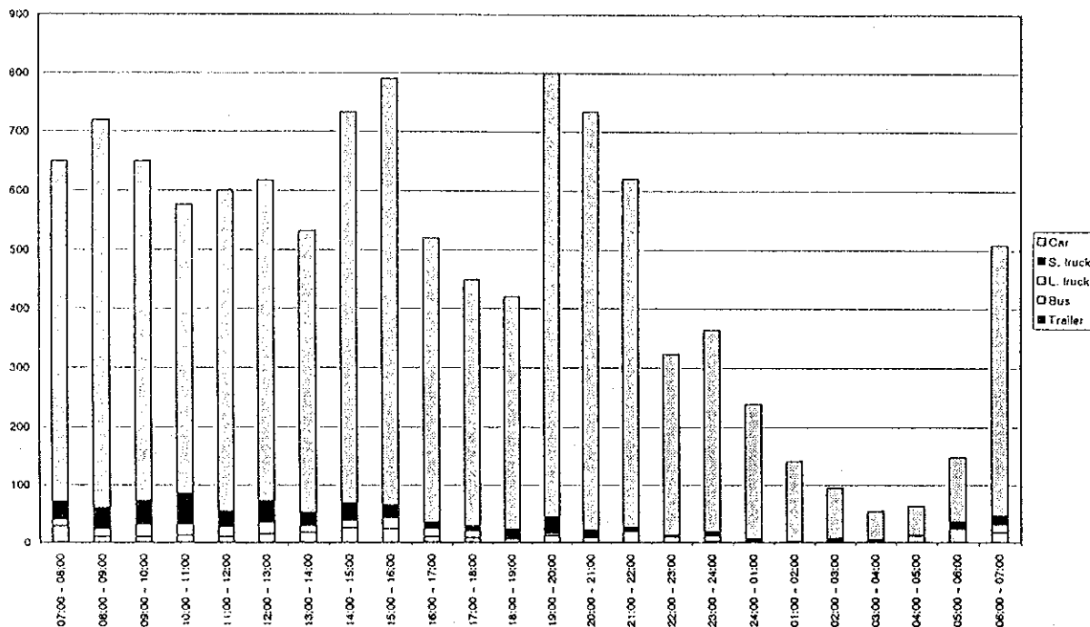
Figure D4.27(116) Hourly Traffic Volume by Vehicle Type - Measuring Point 58 (22/23.04.1998 - weekday)
