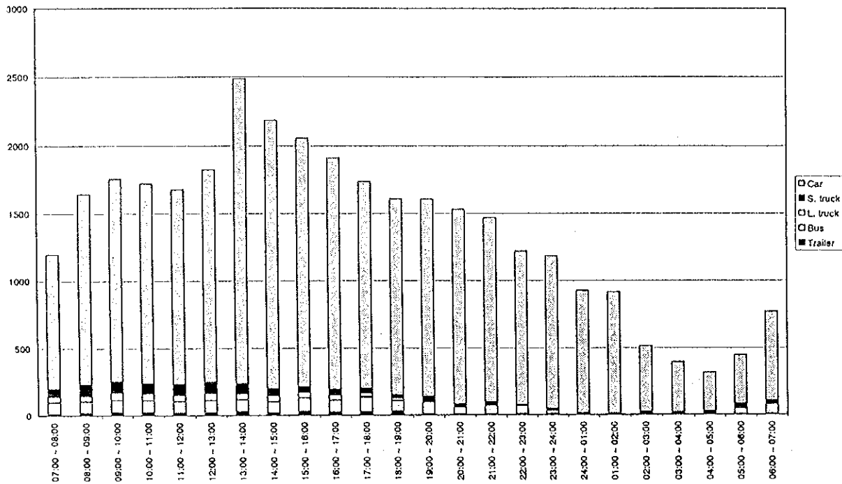
Figure D4.27(128) Hourly Traffic Volume by Vehicle Type - Measuring Point 64 (25/25.04.1998 - holiday)
