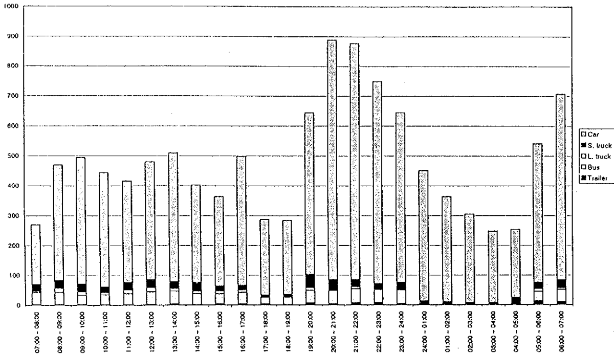
Figure D4.27(132) Hourly Traffic Volume by Vehicle Type - Measuring Point 66 (25/25.04.1998 - holiday)
