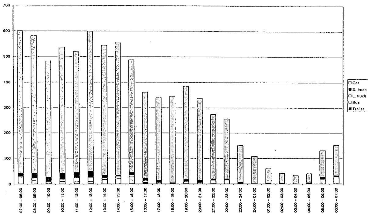
Figure D4.27(123) Hourly Traffic Volume by Vehicle Type - Measuring Point 62 (22/23.04.1998 - weekday)
