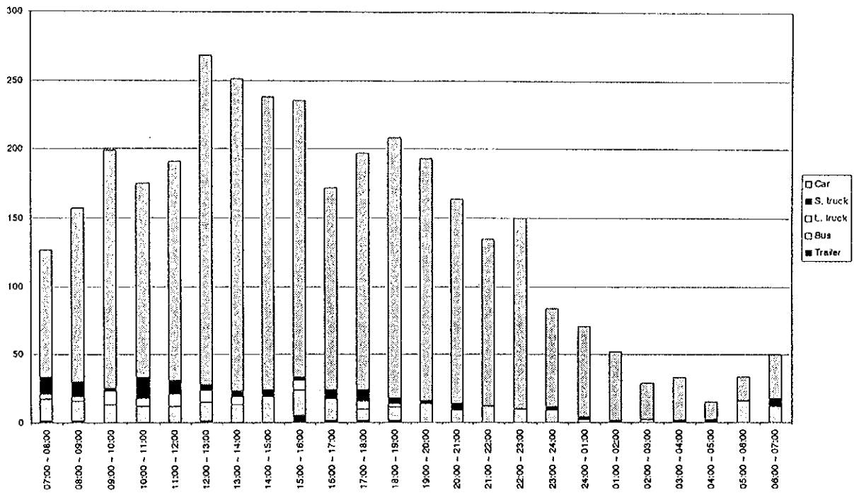
Figure D4.27(109) Hourly Traffic Volume by Vehicle Type - Measuring Point 60 (25/25.04.1998 - holiday)
