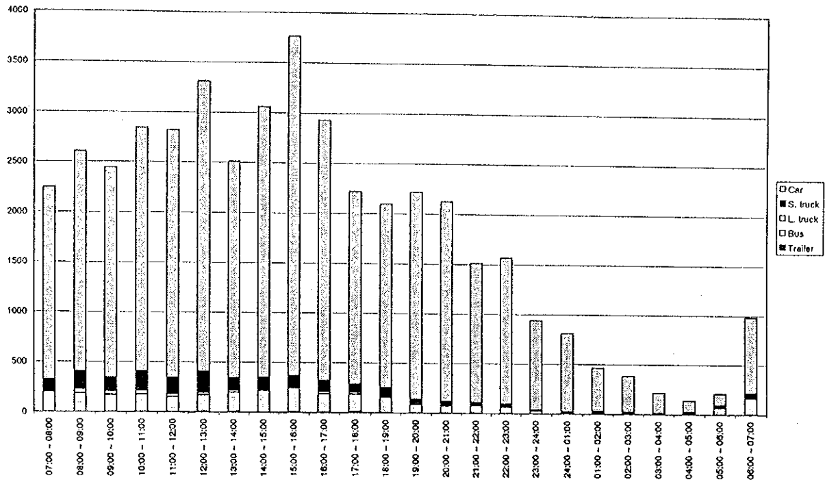
Figure D4.27(71) Hourly Traffic Volume by Vehicle Type - Measuring Point 36 (22/23.04.1998 - weekday)
