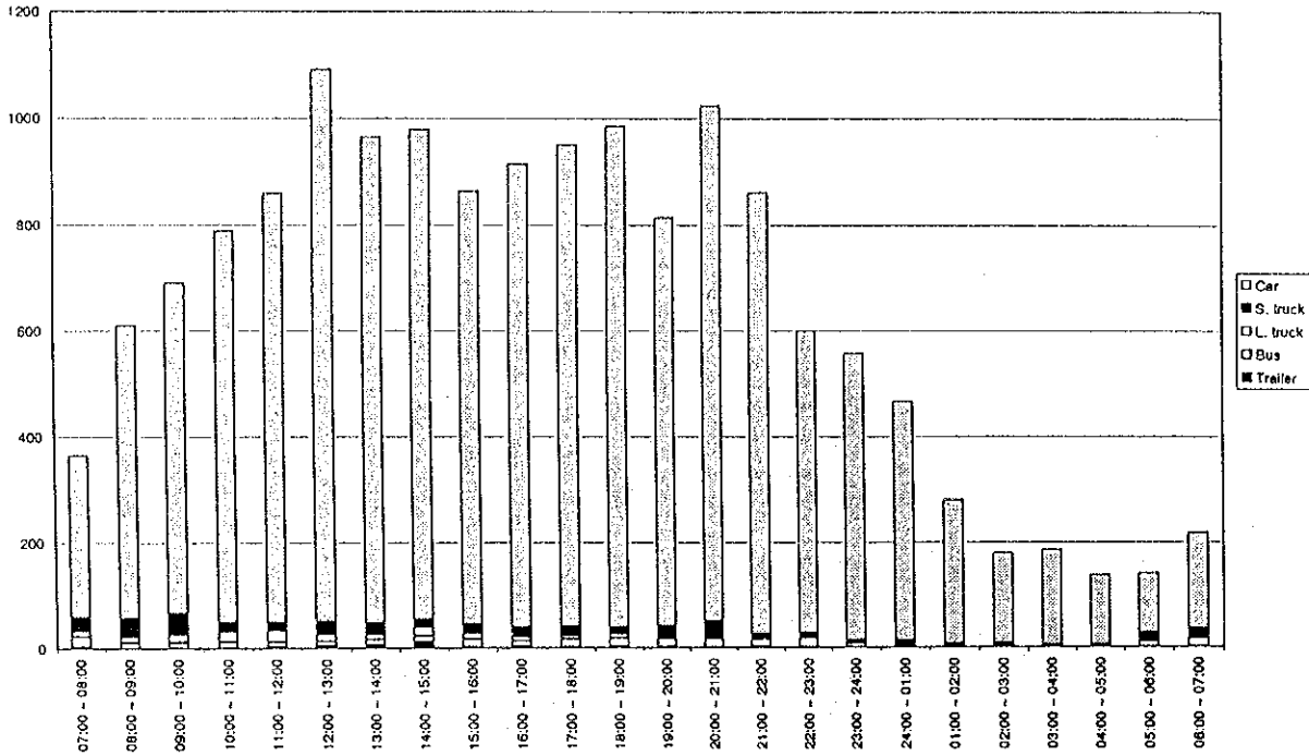
Figure D4.27(106) Hourly Traffic Volume by Vehicle Type - Measuring Point 53 (25/25.04.1998 - holiday)
