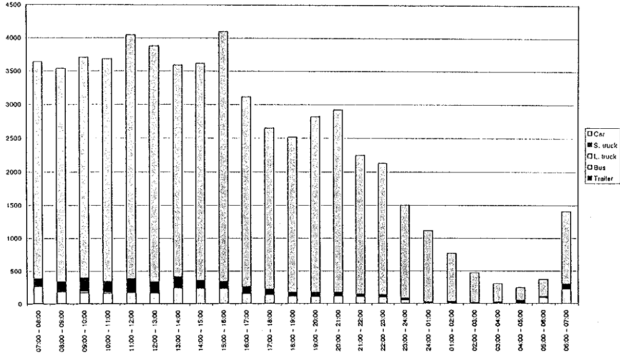
Figure D4.27(97) Hourly Traffic Volume by Vehicle Type - Measuring Point 49 (22/23.04.1998 - weekday)
