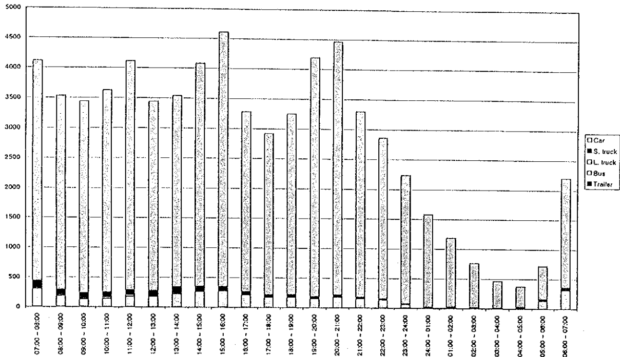
Figure D4.27(93) Hourly Traffic Volume by Vehicle Type - Measuring Point 47 (22/23.04.1998 - weekday)
