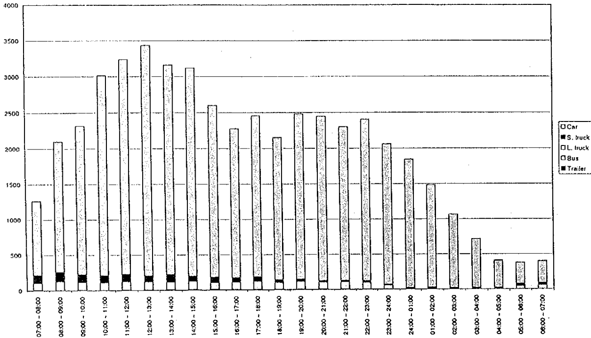
Figure D4.27(98) Hourly Traffic Volume by Vehicle Type - Measuring Point 49 (25/25.04.1998 - holiday)
