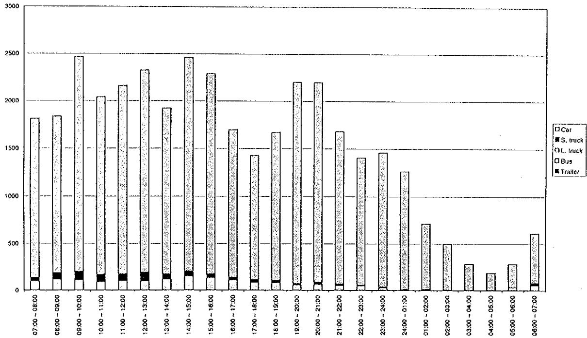
Figure D4.27(85) Hourly Traffic Volume by Vehicle Type - Measuring Point 43 (22/23.04.1998 - weekday)
