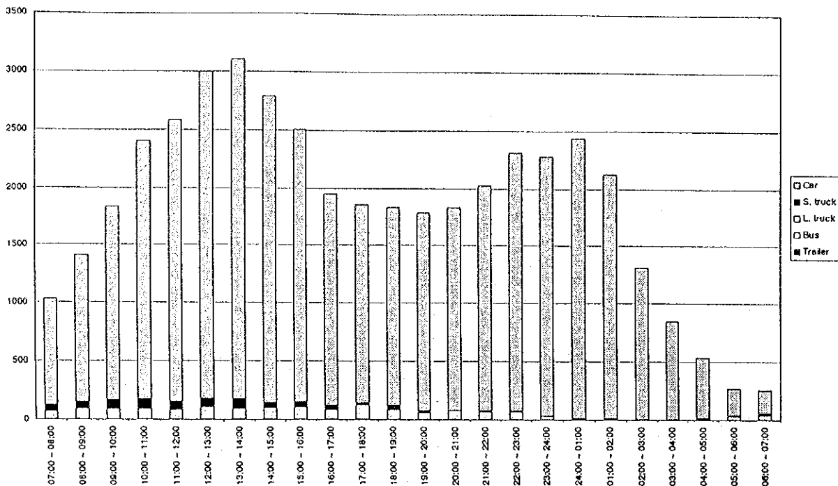
Figure D4.27(80) Hourly Traffic Volume by Vehicle Type - Measuring Point 40 (25/25.04.1998 - holiday)
