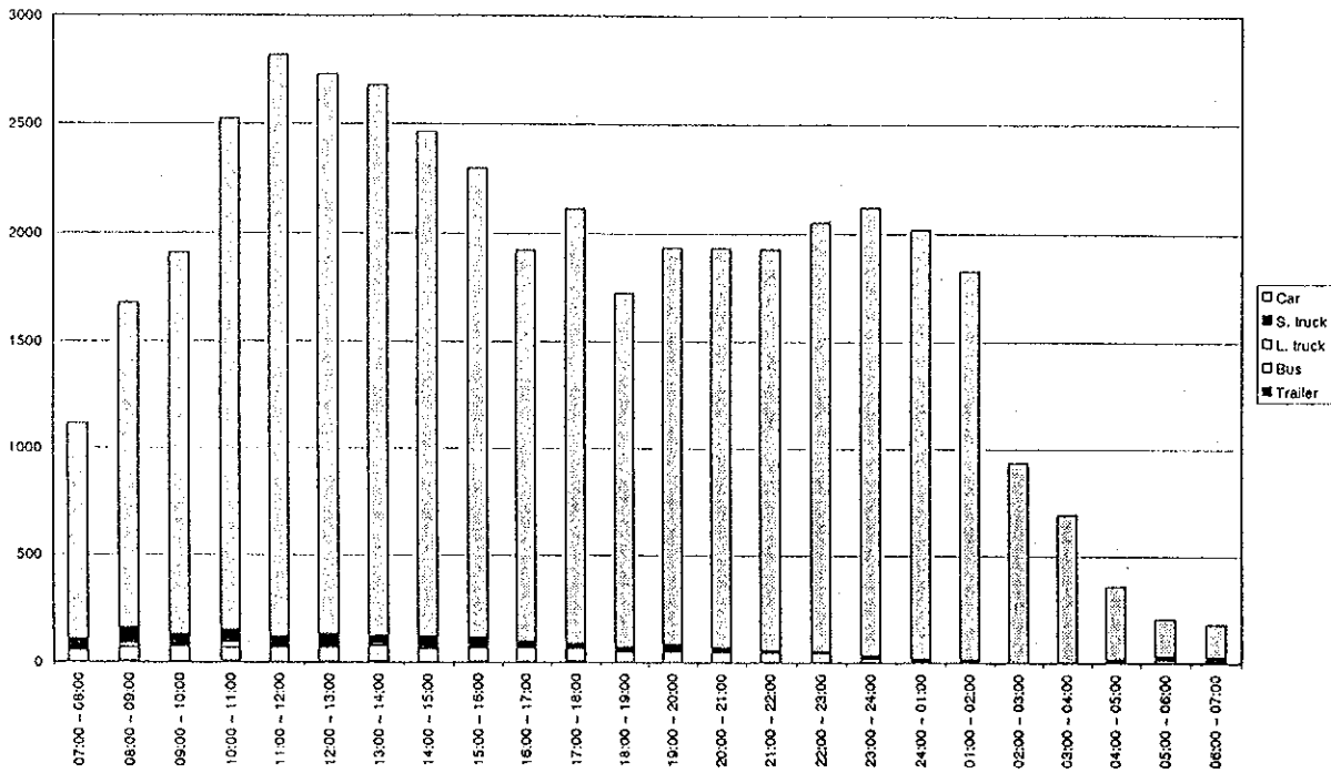
Figure D4.27(88) Hourly Traffic Volume by Vehicle Type - Measuring Point 44 (25/25.04.1998 - holiday)
