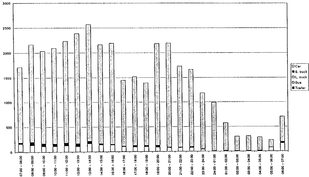
Figure D4.27(95) Hourly Traffic Volume by Vehicle Type - Measuring Point 48 (22/23.04.1998 - weekday)
