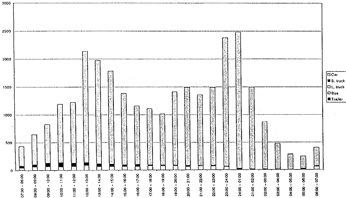
Figure D4.27(86) Hourly Traffic Volume by Vehicle Type - Measuring Point 43 (25/25.04.1998 - holiday)
