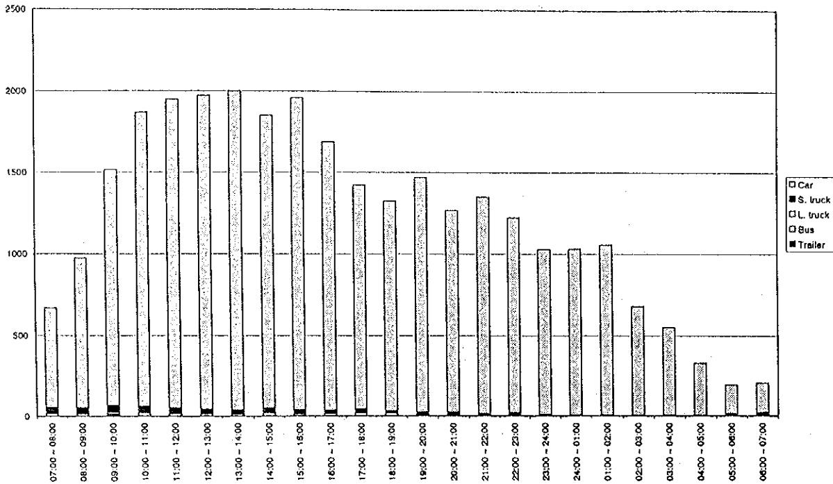
Figure D4.27(74) Hourly Traffic Volume by Vehicle Type - Measuring Point 37 (25/25.04.1998 - holiday)
