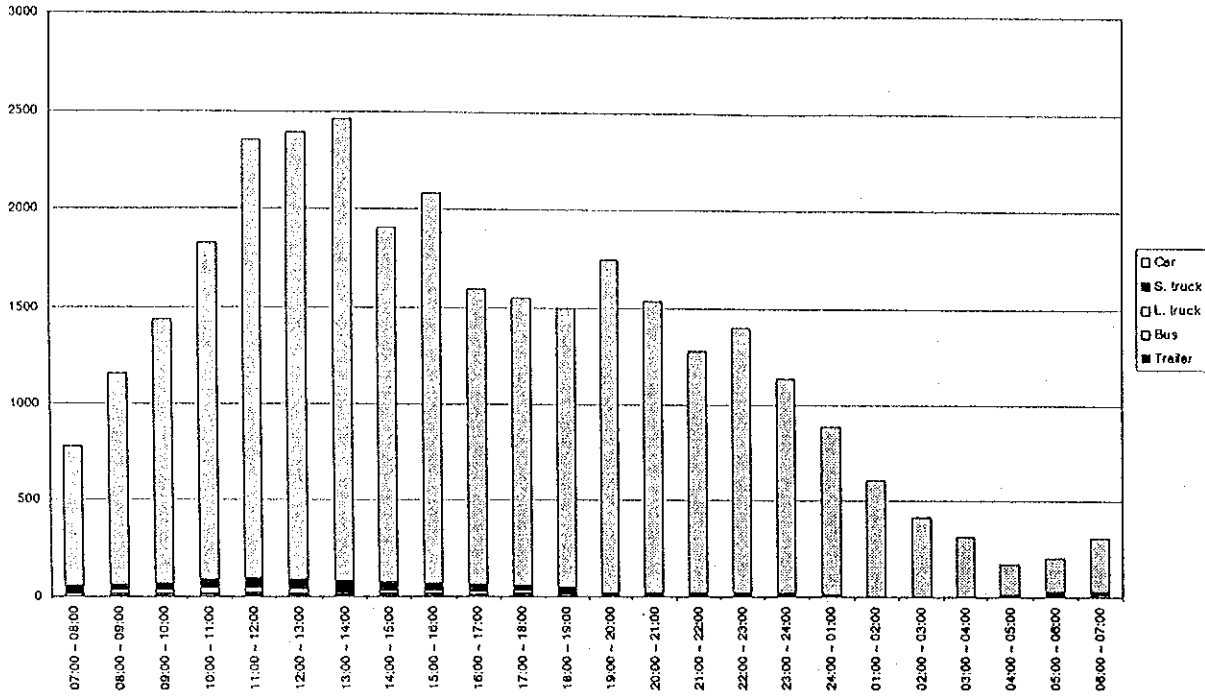
Figure D4.27(78) Hourly Traffic Volume by Vehicle Type - Measuring Point 39 (25/25.04.1998 - holiday)
