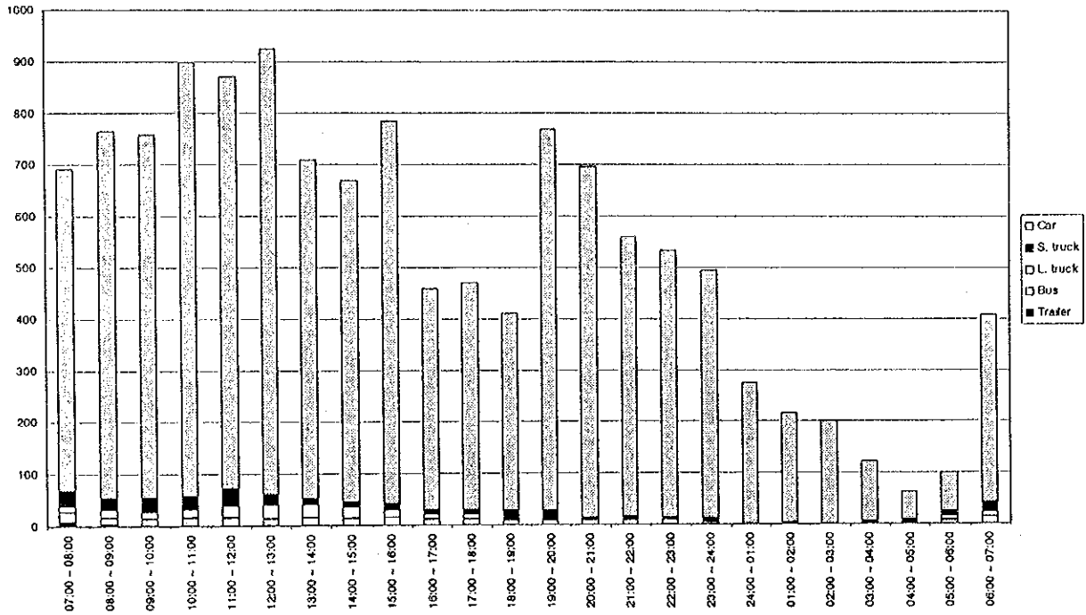
Figure D4.27(83) Hourly Traffic Volume by Vehicle Type - Measuring Point 42 (22/23.04.1998 - weekday)
