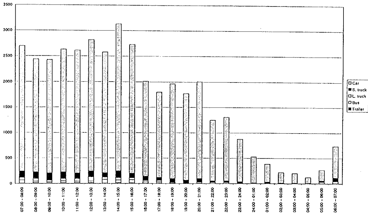
Figure D4.27(101) Hourly Traffic Volume by Vehicle Type - Measuring Point 51 (22/23.04.1998 - weekday)
