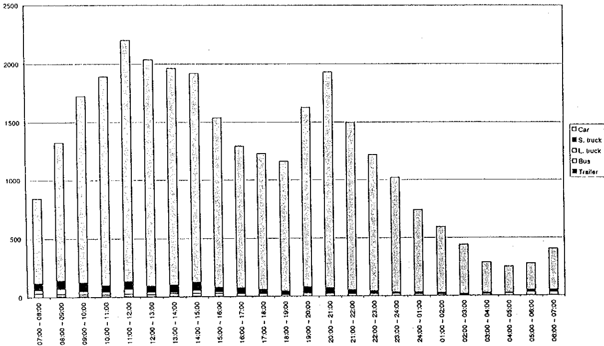
Figure D4.27(102) Hourly Traffic Volume by Vehicle Type - Measuring Point 51 (25/25.04.1998 - holiday)
