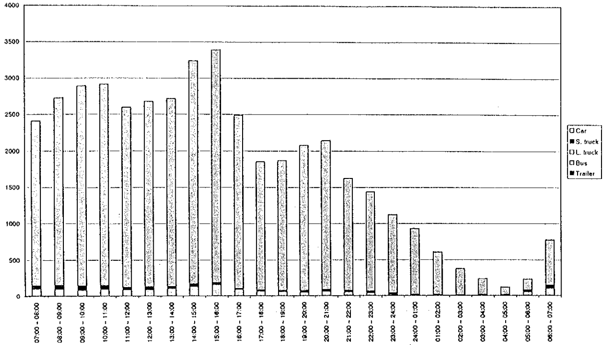
Figure D4.27(81) Hourly Traffic Volume by Vehicle Type - Measuring Point 41 (22/23.04.1998 - weekday)
