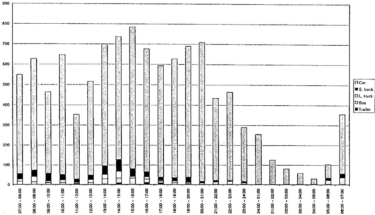
Figure D4.27(107) Hourly Traffic Volume by Vehicle Type - Measuring Point 54 (22/23.04.1998 - weekday)
