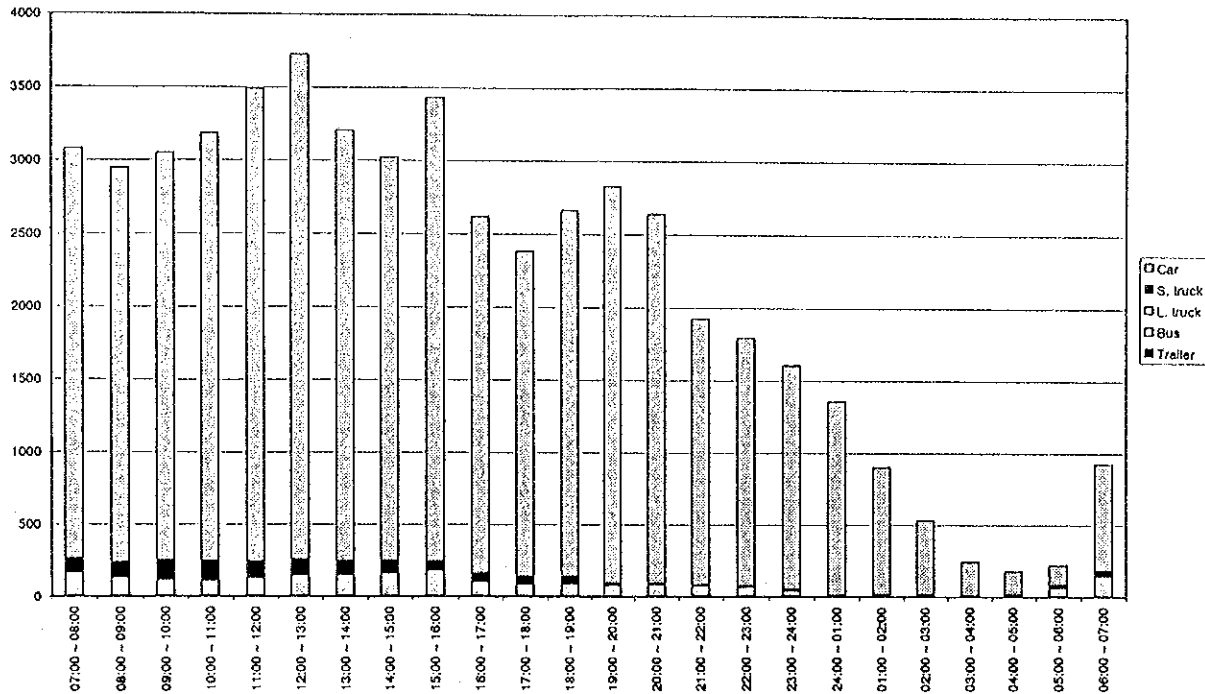
Figure D4.27(79) Hourly Traffic Volume by Vehicle Type - Measuring Point 40 (22/23.04.1998 - weekday)
