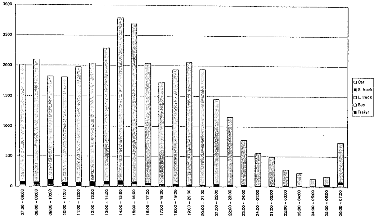
Figure D4.27(75) Hourly Traffic Volume by Vehicle Type - Measuring Point 38 (22/23.04.1998 - weekday)
