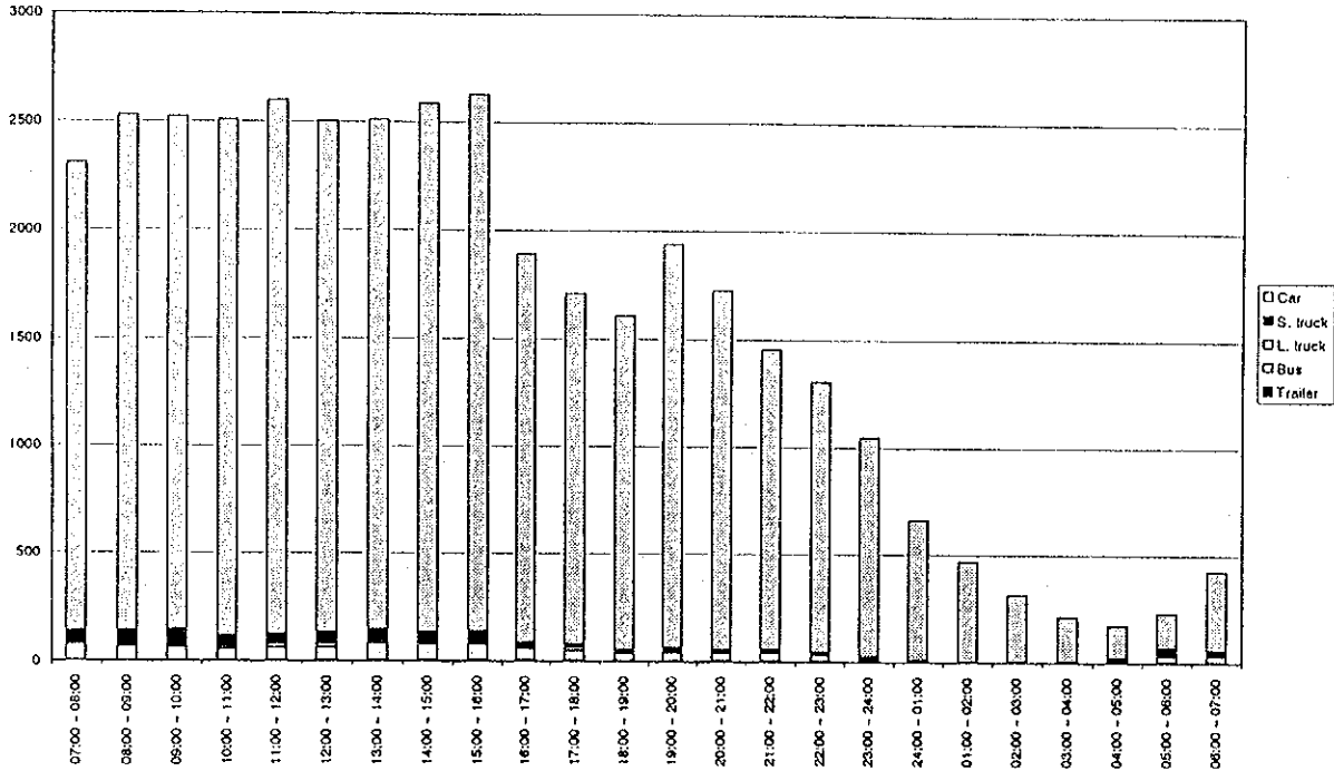
Figure D4.27(89) Hourly Traffic Volume by Vehicle Type - Measuring Point 45 (22/23.04.1998 - weekday)
