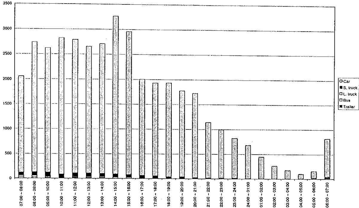
Figure D4.27(73) Hourly Traffic Volume by Vehicle Type - Measuring Point 37 (22/23.04.1998 - weekday)
