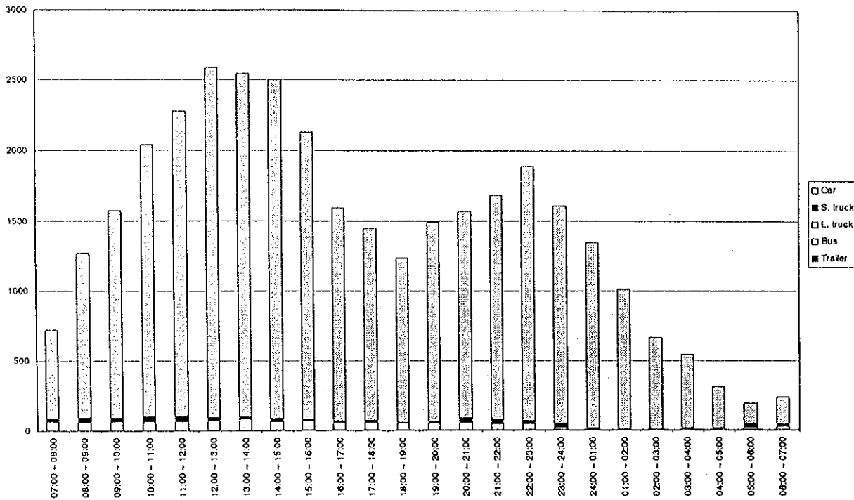
Figure D4.27(82) Hourly Traffic Volume by Vehicle Type - Measuring Point 41 (25/25.04.1998 - holiday)
