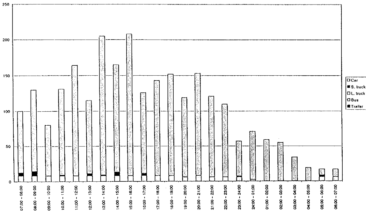
Figure D4.27(104) Hourly Traffic Volume by Vehicle Type - Measuring Point 52 (25/25.04.1998 - holiday)
