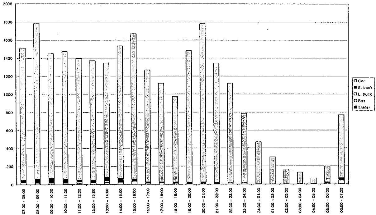
Figure D4.27(99) Hourly Traffic Volume by Vehicle Type - Measuring Point 50 (22/23.04.1998 - weekday)
