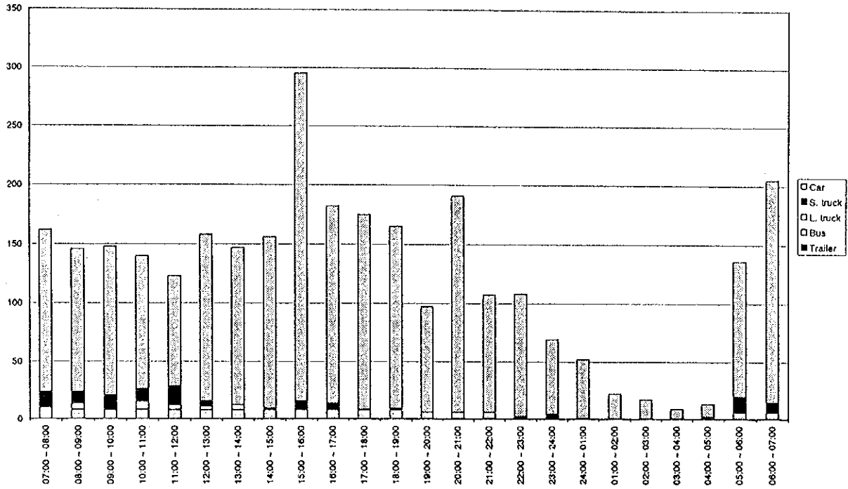
Figure D4.27(103) Hourly Traffic Volume by Vehicle Type - Measuring Point 52 (22/23.04.1998 - weekday)
