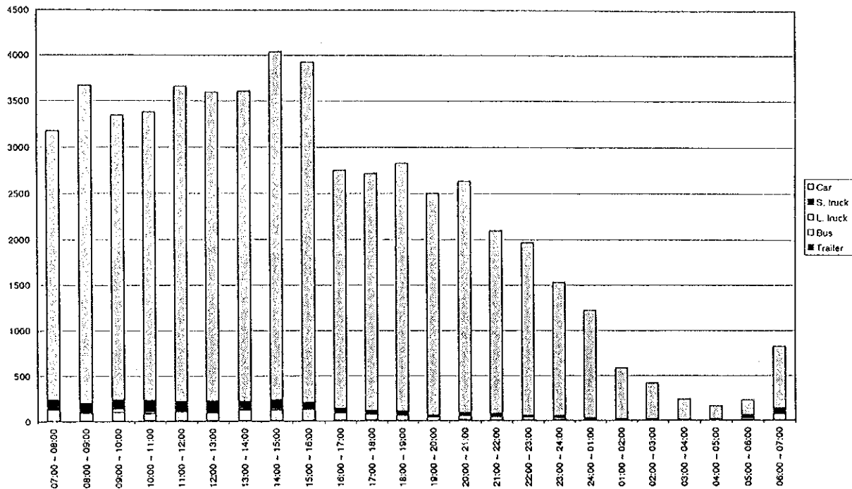
Figure D4.27(87) Hourly Traffic Volume by Vehicle Type - Measuring Point 44 (22/23.04.1998 - weekday)
