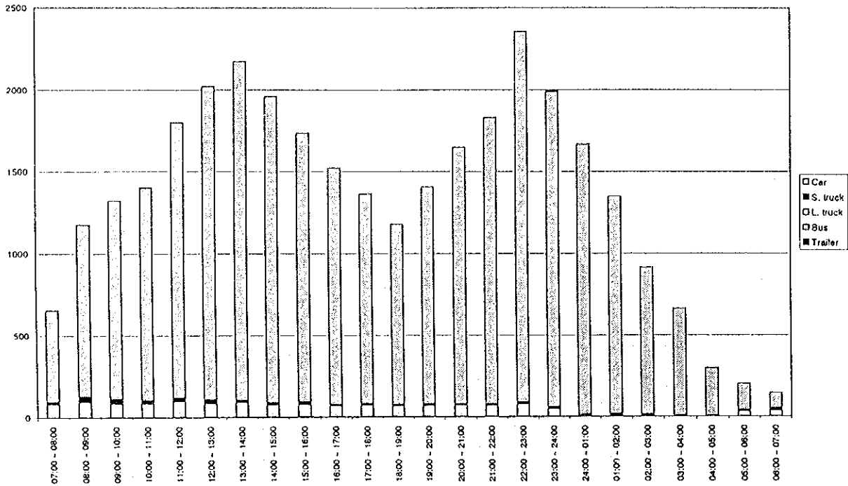
Figure D4.27(96) Hourly Traffic Volume by Vehicle Type - Measuring Point 48 (25/25.04.1998 - holiday)
