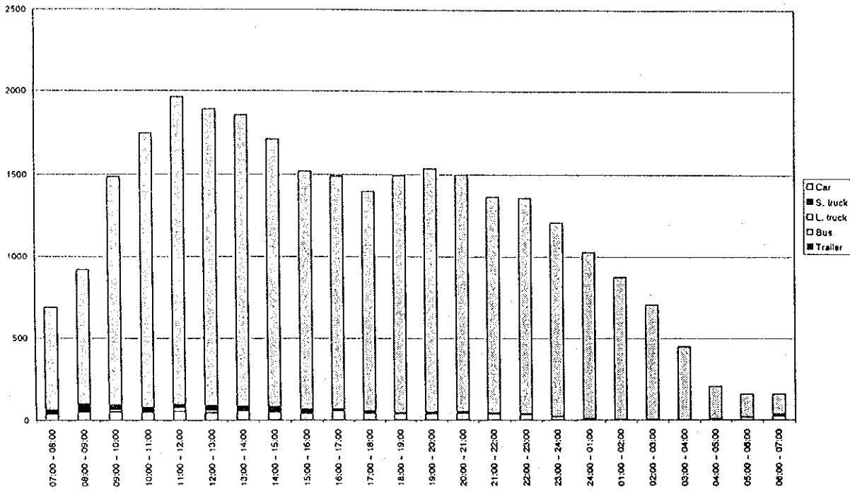
Figure D4.27(90) Hourly Traffic Volume by Vehicle Type - Measuring Point 45 (25/25.04.1998 - holiday)
