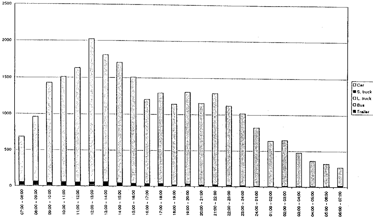
Figure D4.27(76) Hourly Traffic Volume by Vehicle Type - Measuring Point 38 (25/25.04.1998 - holiday)
