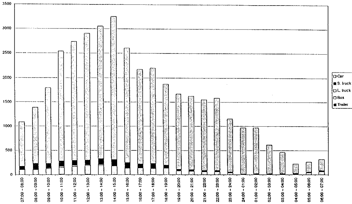
Figure D4.27(72) Hourly Traffic Volume by Vehicle Type - Measuring Point 36 (25/25.04.1998 - holiday)
