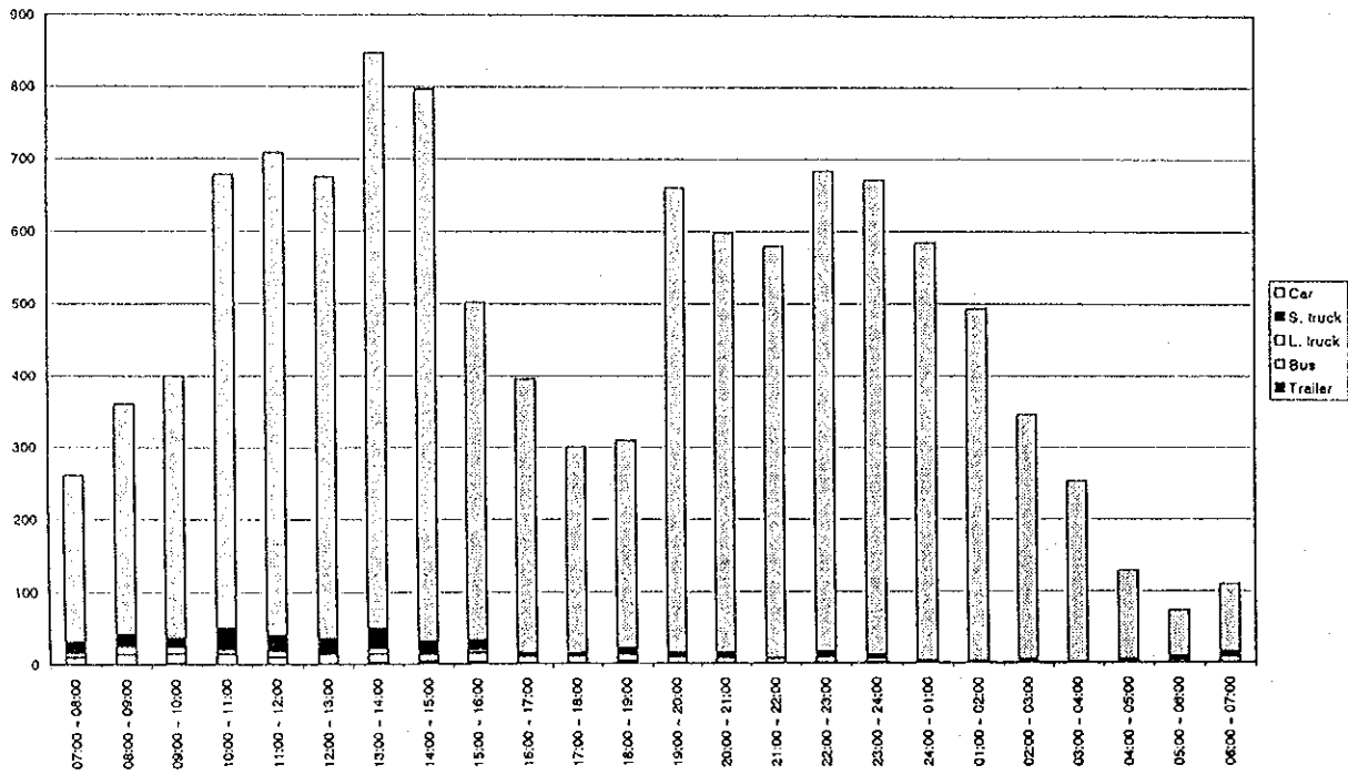
Figure D4.27(84) Hourly Traffic Volume by Vehicle Type - Measuring Point 42 (25/25.04.1998 - holiday)
