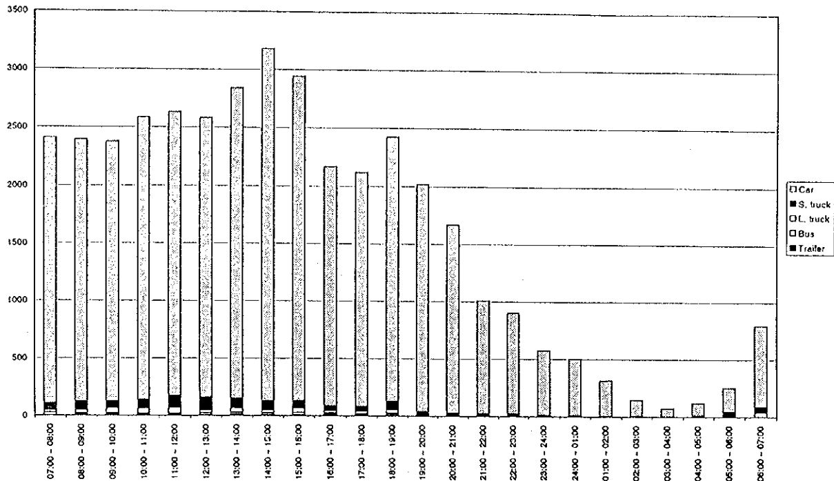
Figure D4.27(77) Hourly Traffic Volume by Vehicle Type - Measuring Point 39 (22/23.04.1998 - weekday)
