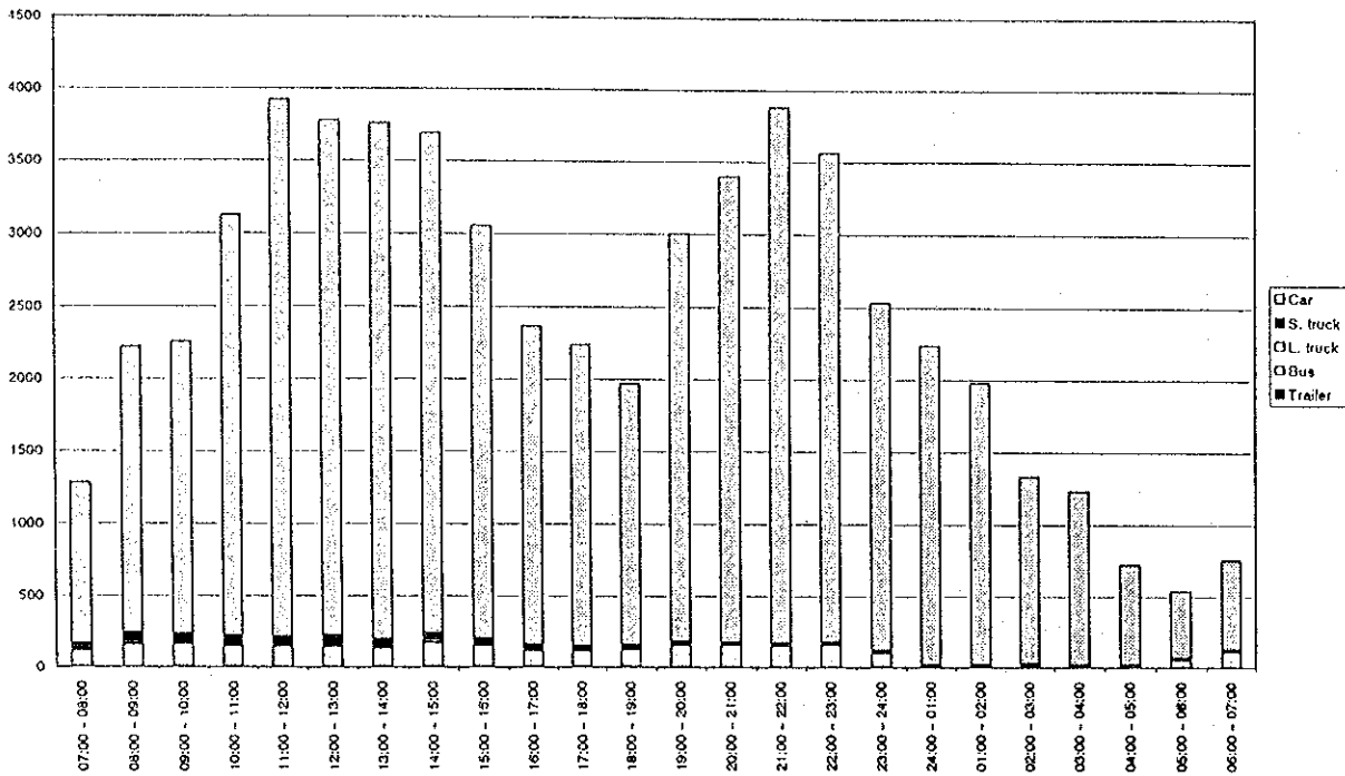
Figure D4.27(94) Hourly Traffic Volume by Vehicle Type - Measuring Point 47 (25/25.04.1998 - holiday)
