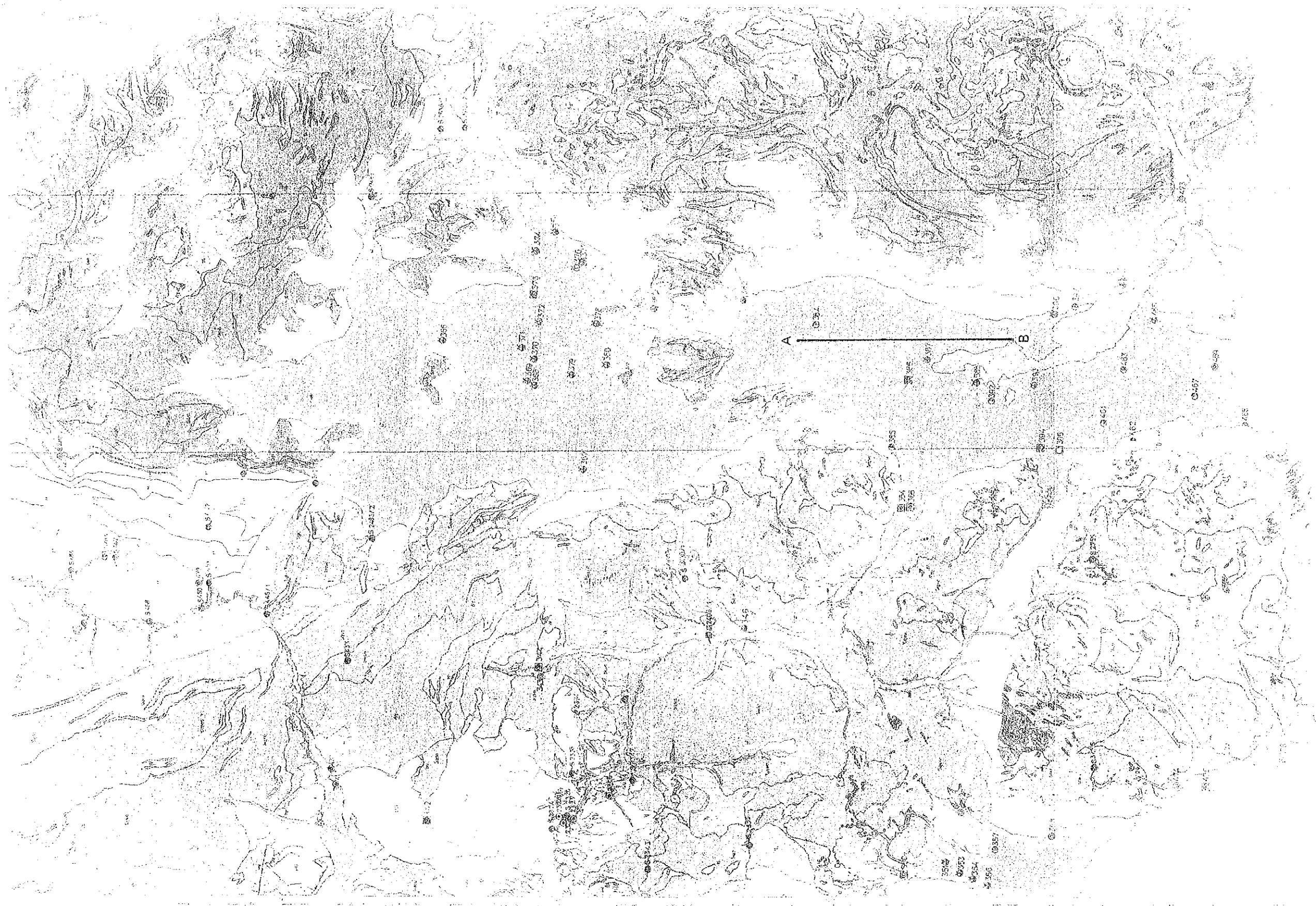
Figure B.44 Hydrogeological Map of Pelagonija Valley
