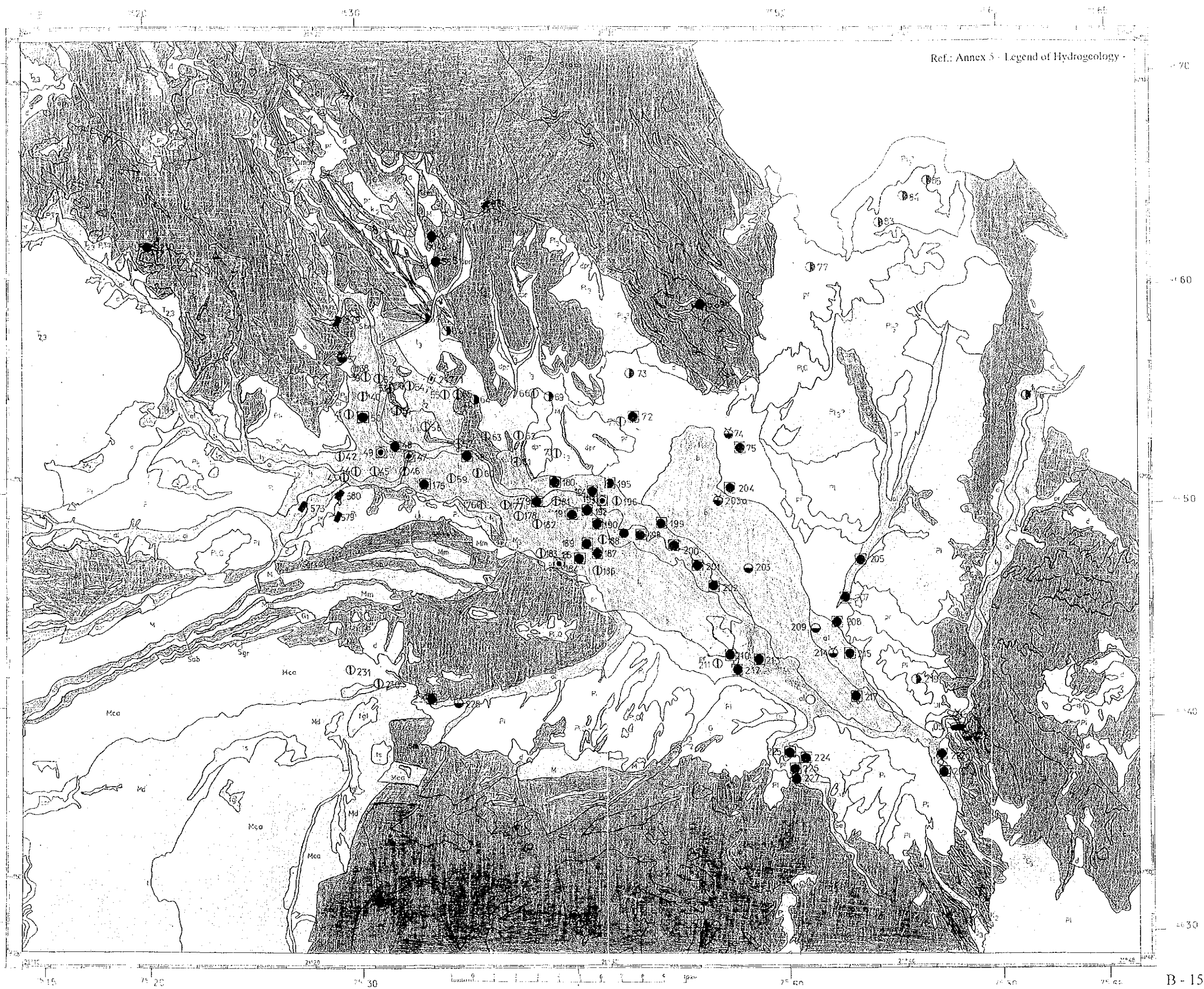
Figure B.47 Hydrogeological Map of Skopje Valley
