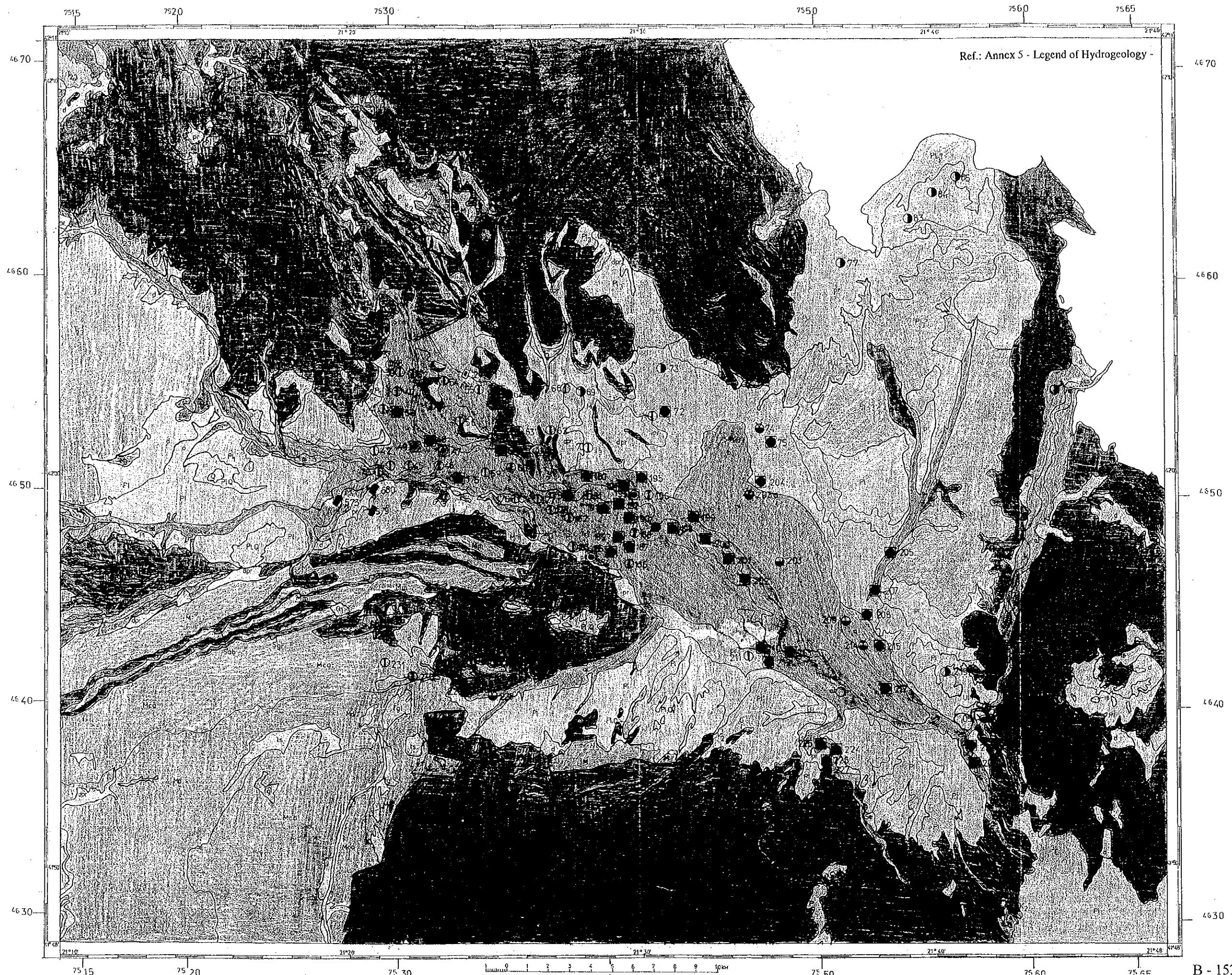
Figure B.47 Hydrogeological Map of Skopje Valley
