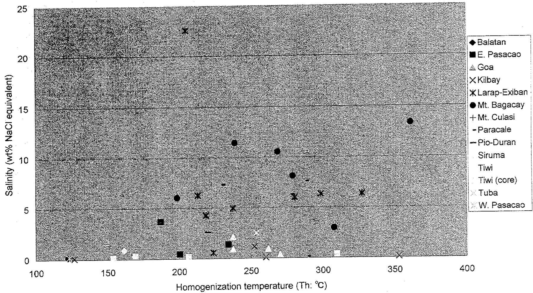
Homogenization temperature vs. Salinity (Average values from each specimen)
