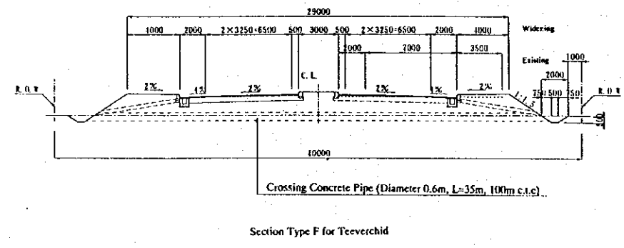
TYPICAL CROSS SECTION Scale 1:400
