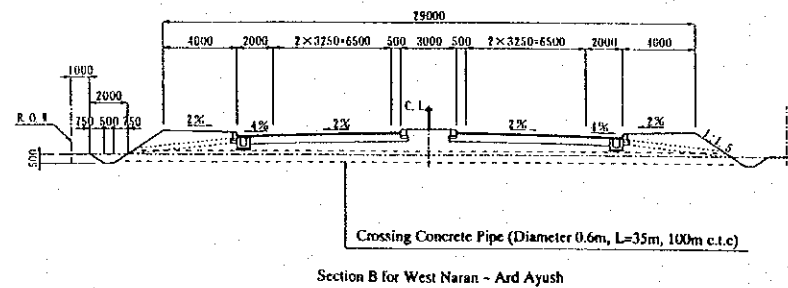
TYPICAL CROSS SECTION Scale 1:400
