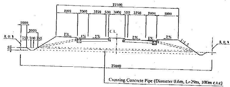
Section B' for South TV - N/Rd. NO.88 (Embankment)
