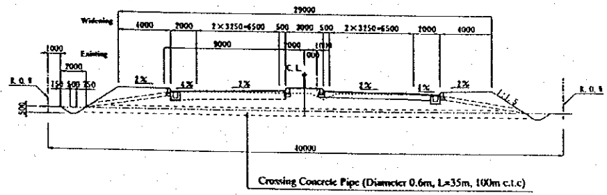
Section Type F for NW Tolgoit
