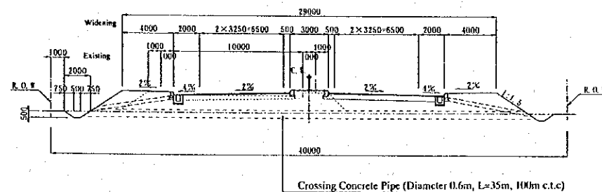
Section Type F for NW Tolgoit
