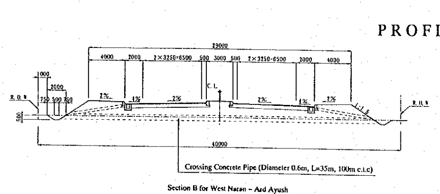
TYPICAL CROSS SECTION Scale 1:400
