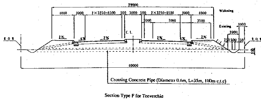
TYPICAL CROSS SECTION Scale 1:400
