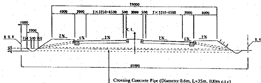
Section B for South Tolgoit (west) (Note: West part of 0.346km length is new construction)
