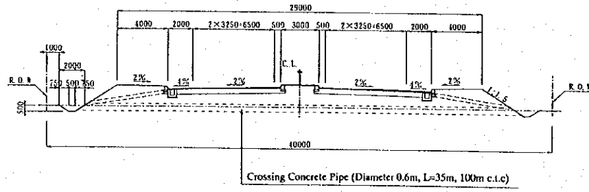
TYPICAL CROSS SECTION Scale 1:400
