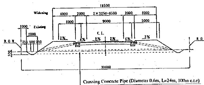
Section Type G for N/Rd.88 - IS11
