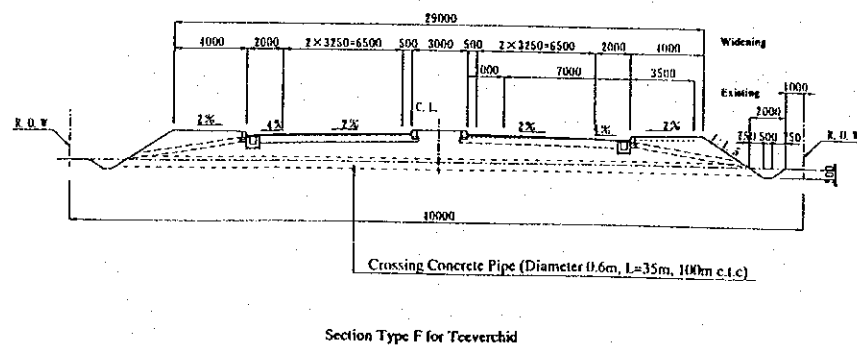
TYPICAL CROSS SECTION Scale 1:400
