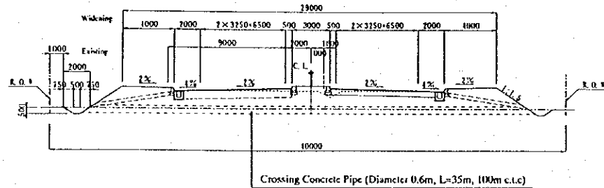
Section Type F for South Tolgoit
