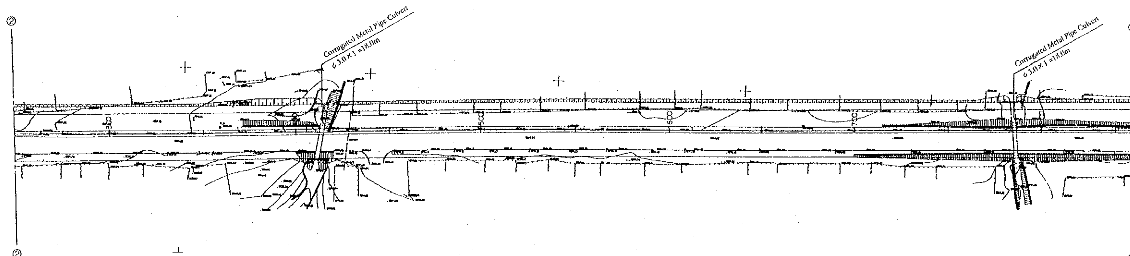
PLAN(-3) Scale 1:2000
