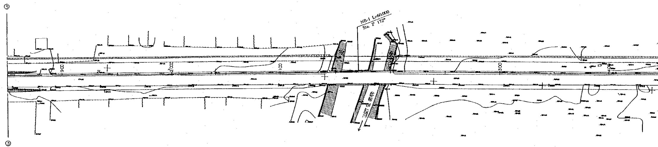
PLAN(-4) Scale 1:2000
