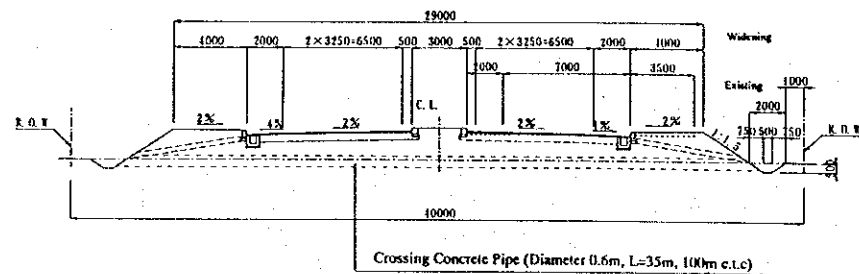
Section Type F for Teverchid
