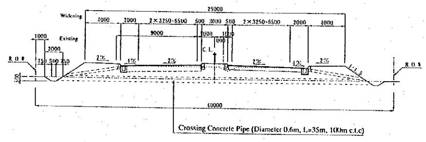
Section Type F for South Tolgoi
