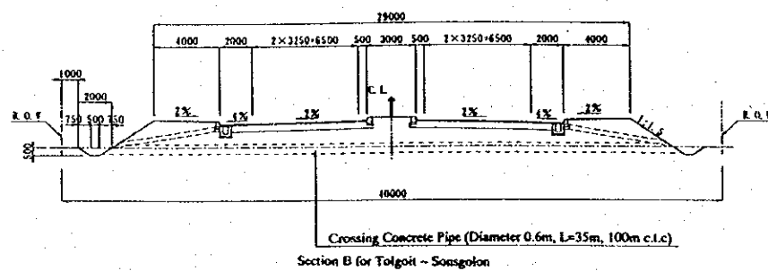
TYPICAL CROSS SECTION Scale 1:400
