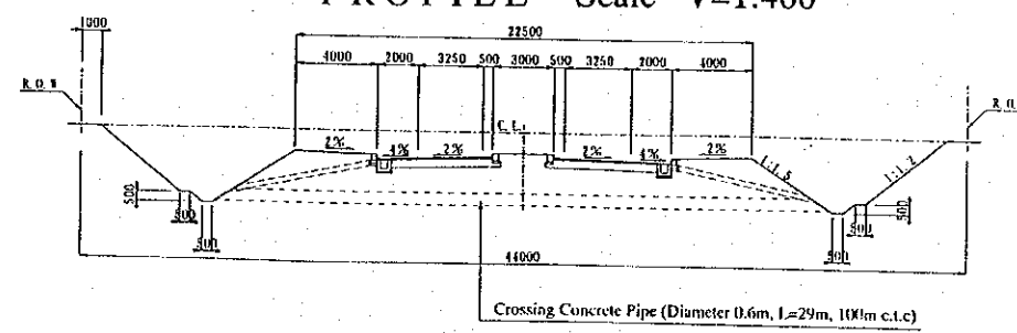
Section B' for South TV - N/Rd. NO.88 (Cut)
