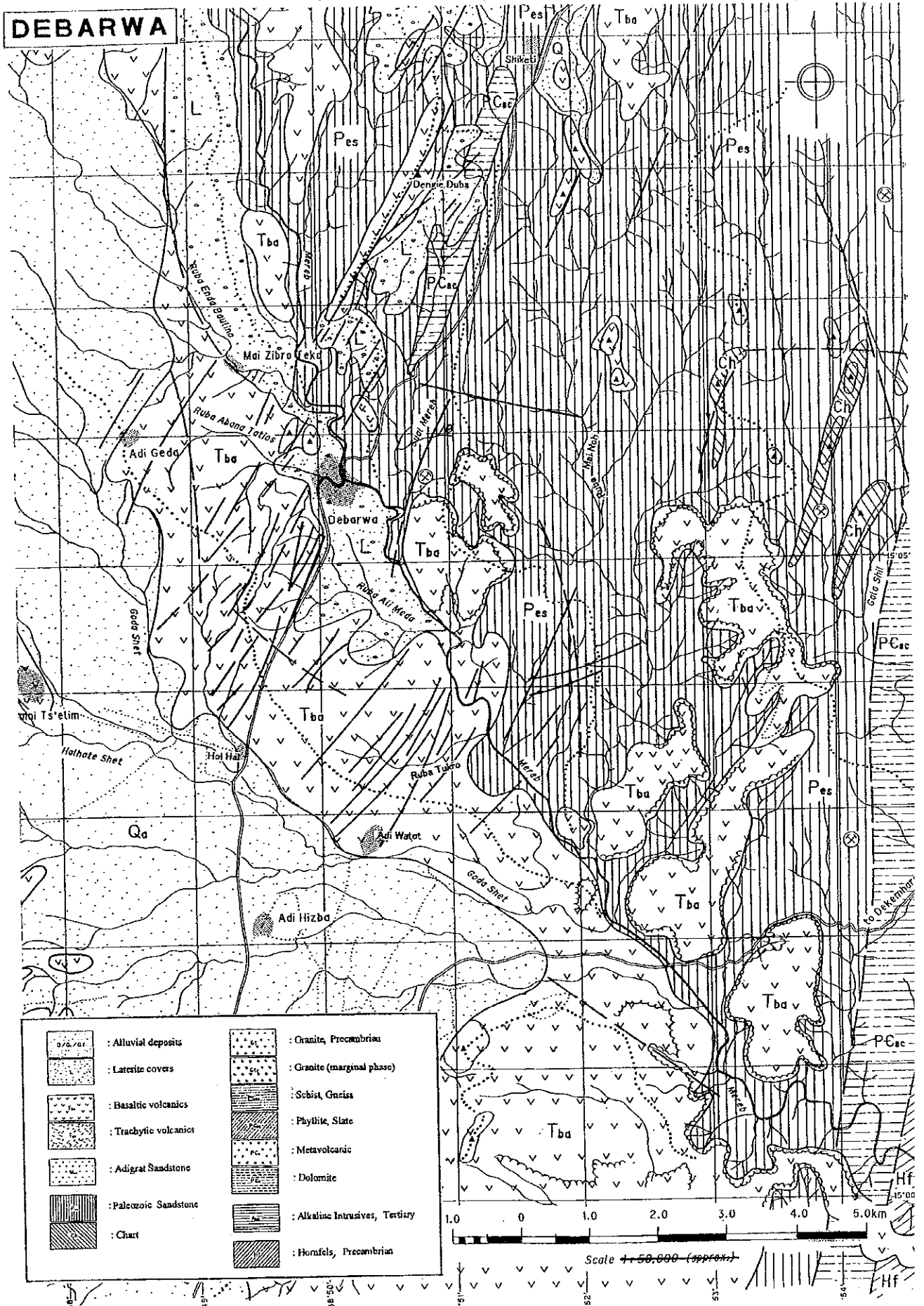
Figure 4.1.2 Geological Map
