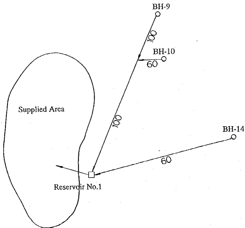
Figure 7.2.1 Plan of Water Sources and Transmission Pipelines (2005)
