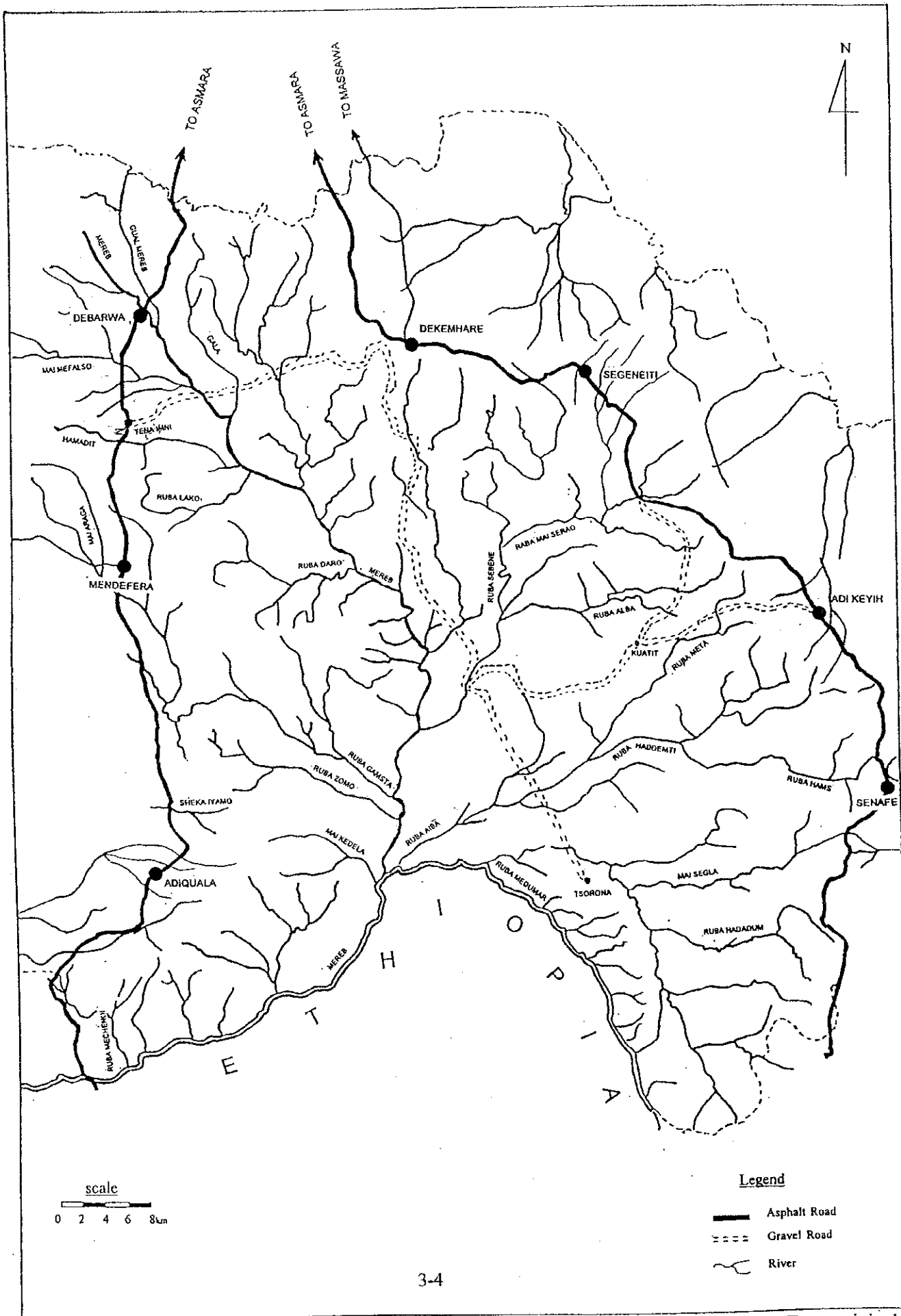
Figure 3.1.2 Drainage Network
