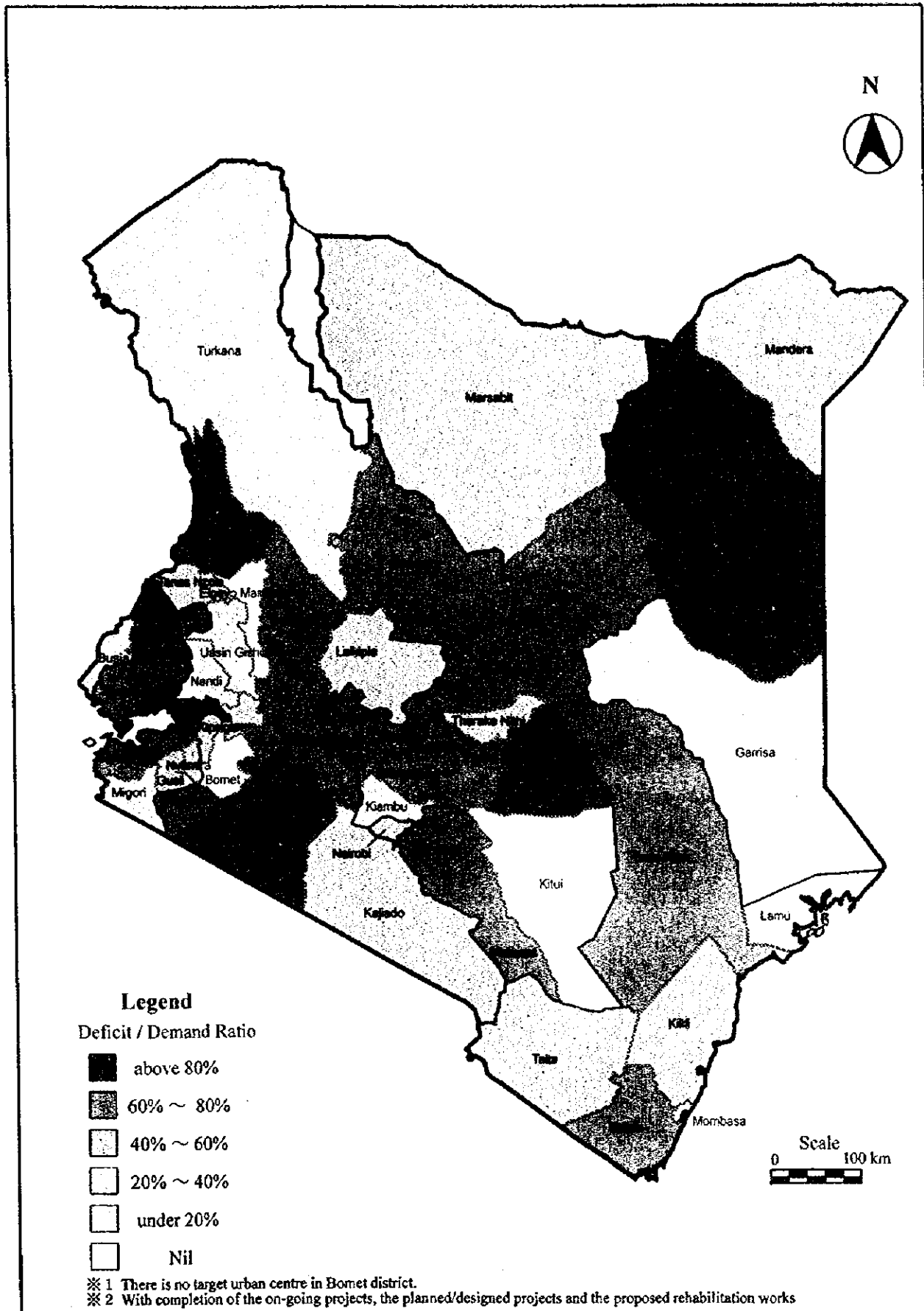
THE AFTERCARE STUDY ON THE NATIONAL WATER MASTER PLAN Figure - 6.3.3 Urban Water Supply Water Deficit in 2010 Under Step 4 JAPAN INTERNATIONAL COOPERATION AGENCY
