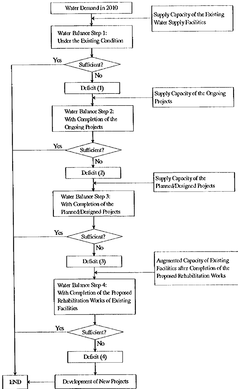
THE AFTERCARE STUDY ON THE NATIONAL WATER MASTER PLAN Figure - 6.3.1 JAPAN INTERNATIONAL COOPERATION AGENCY Flow Chart of Water Balance Calculation
