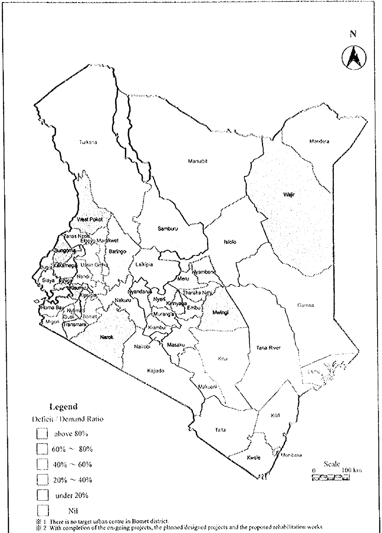
Figure - 6.3.3 Urban Water Supply Water Deficit in 2010 Under Step 4
