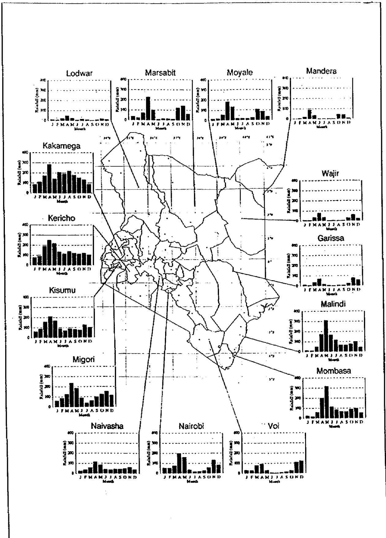
Figure - 2.6.4 Monthly Rainfall Variation at Representative Rainfall Gauging Station
