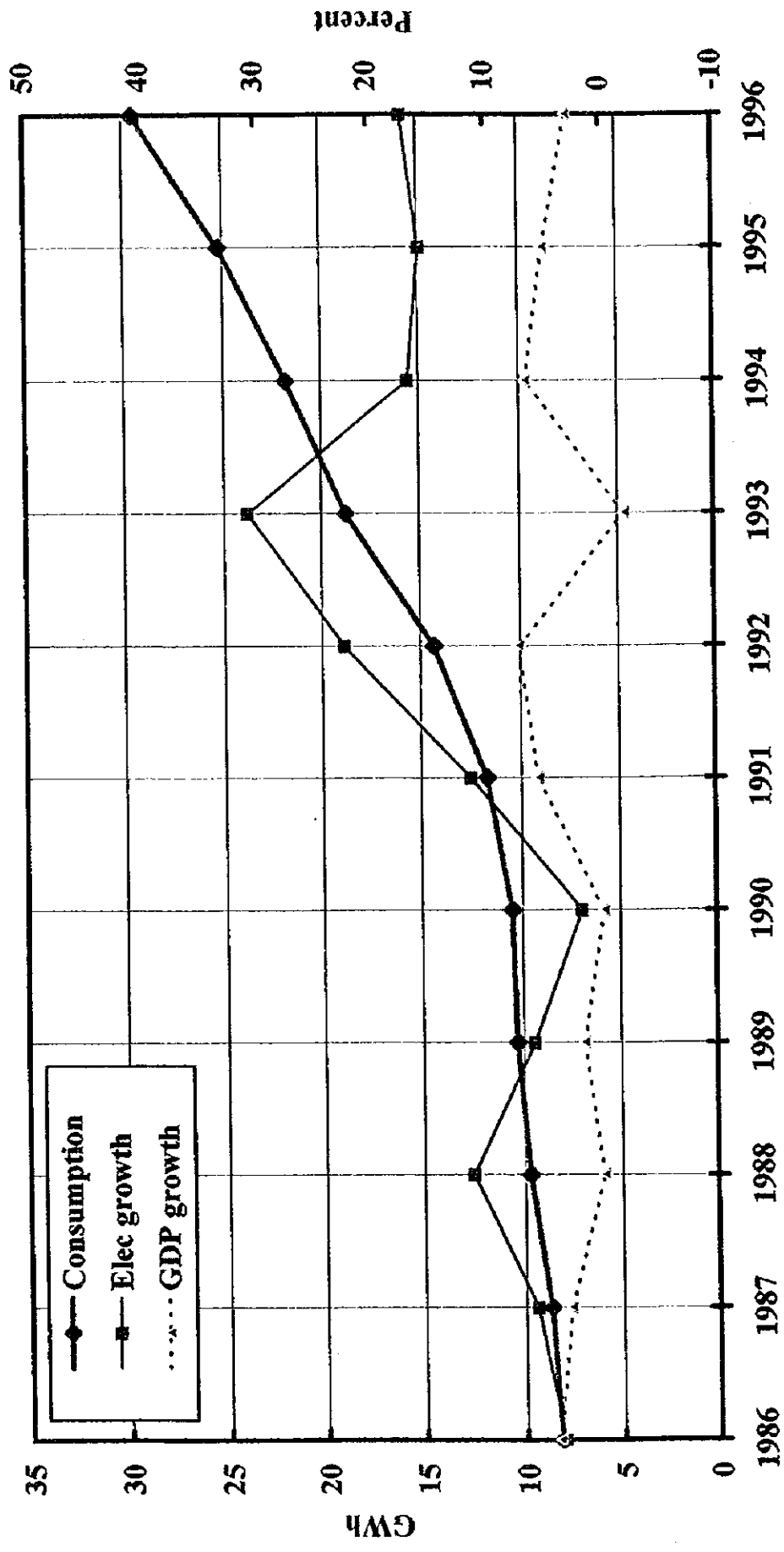
A.7 Luderitz Municipality Electricity Consumption
