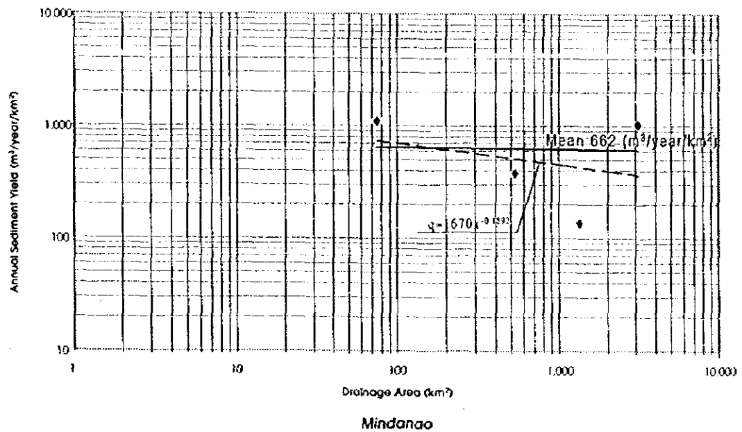
Figure 2-19 ANNUAL SEDIMENT YIELD VERSUS DRAINAGE AREA
