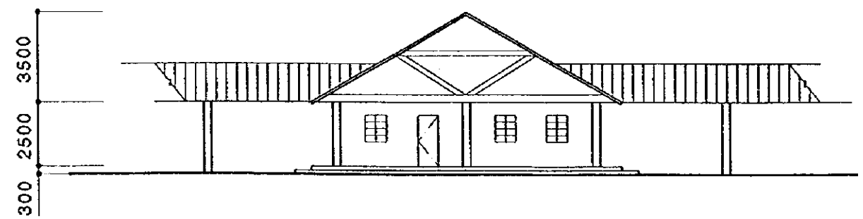
FRONT ELEVATION
