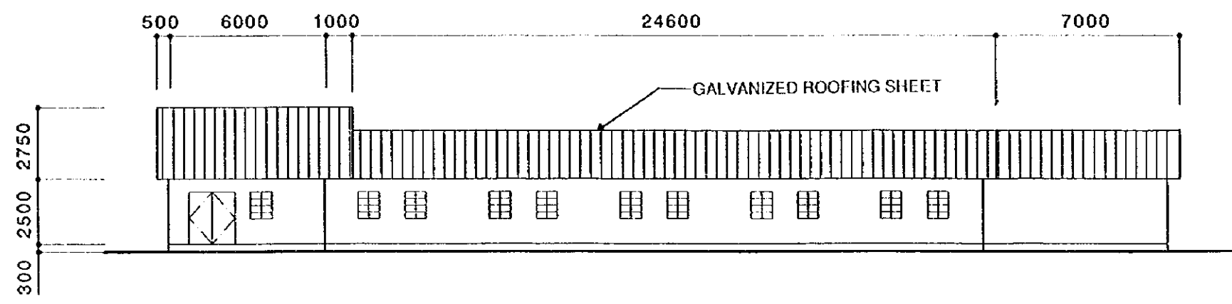
SIDE ELEVATION
