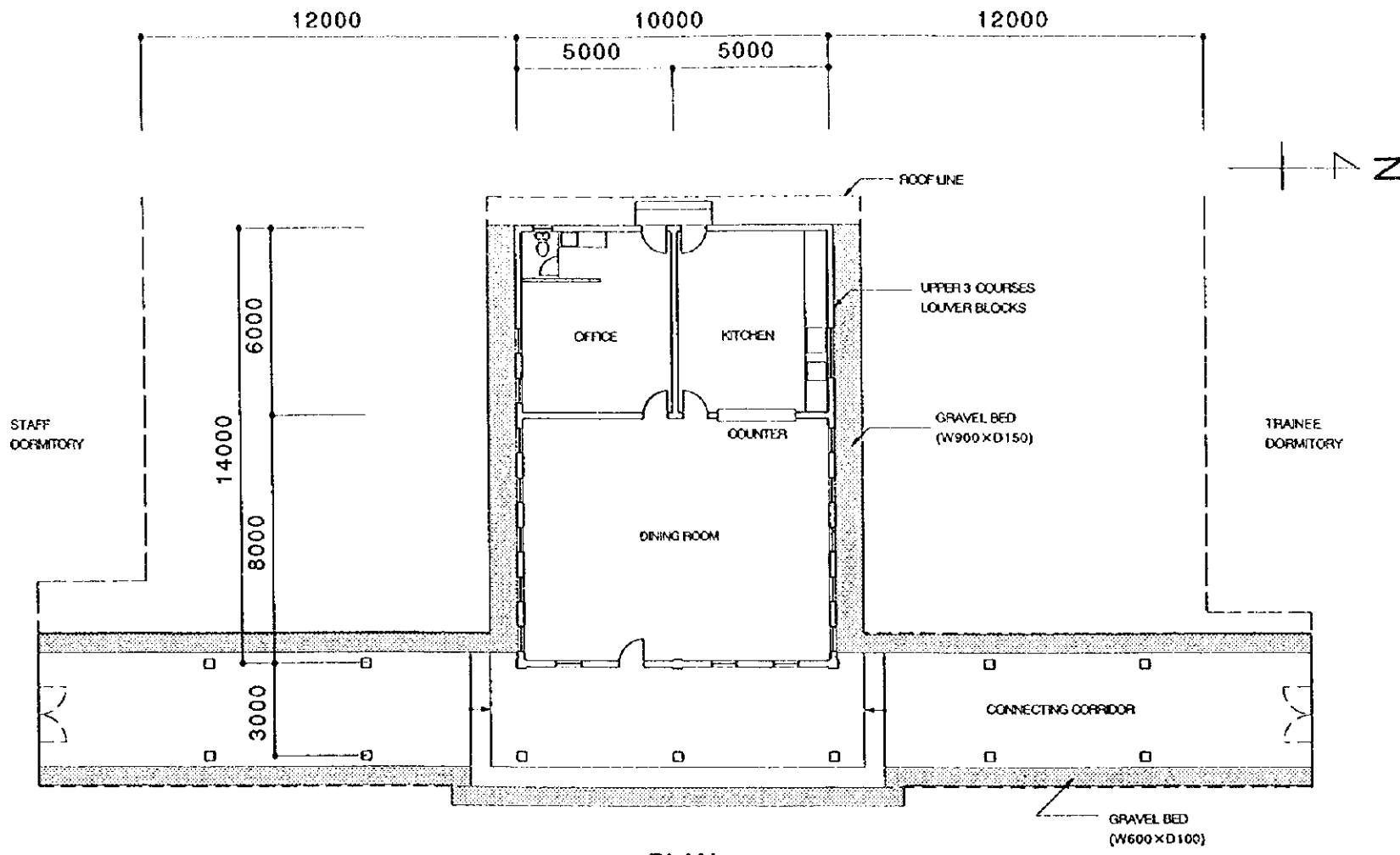
PLAN
