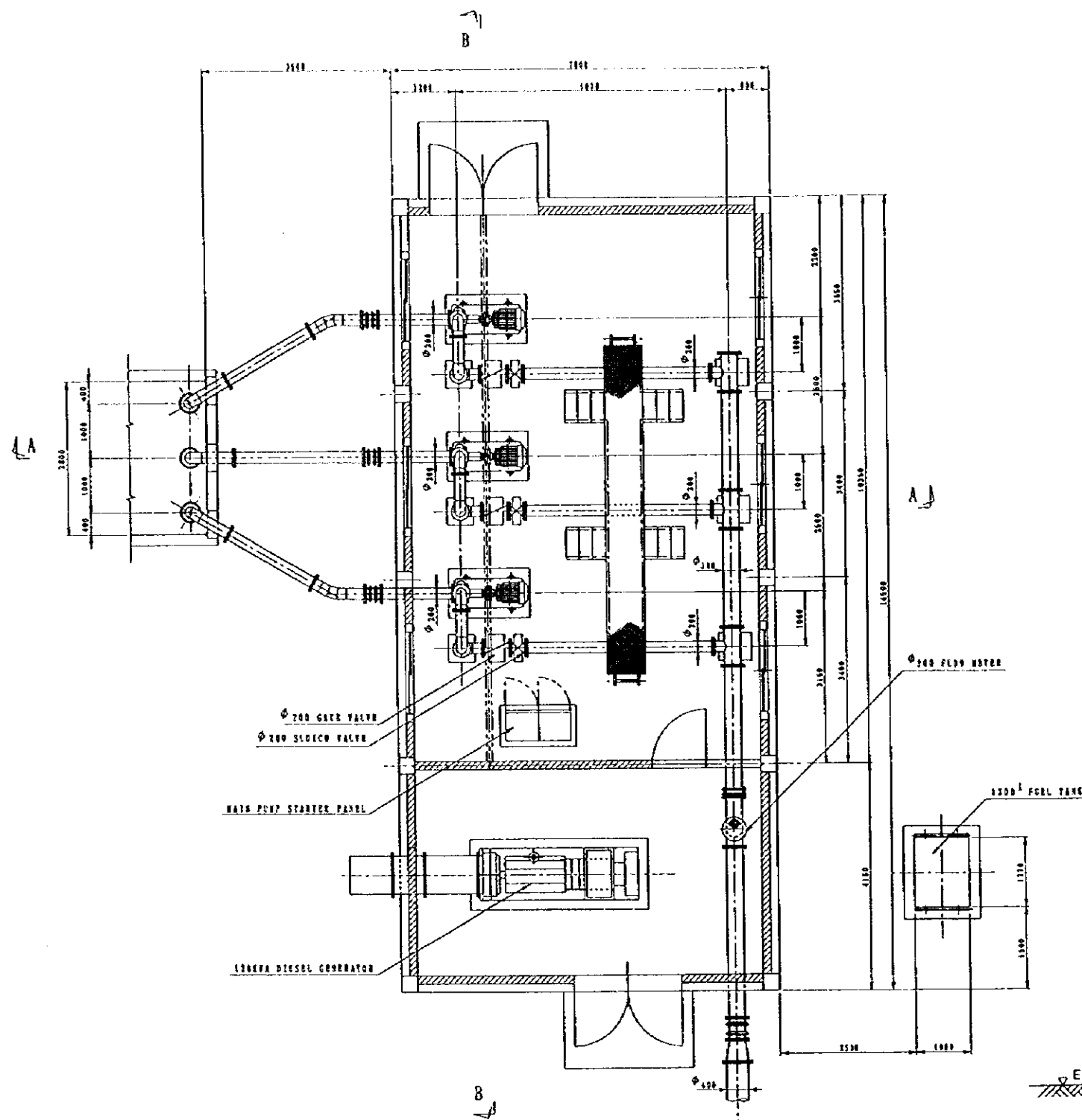
P L A N S-1/50
