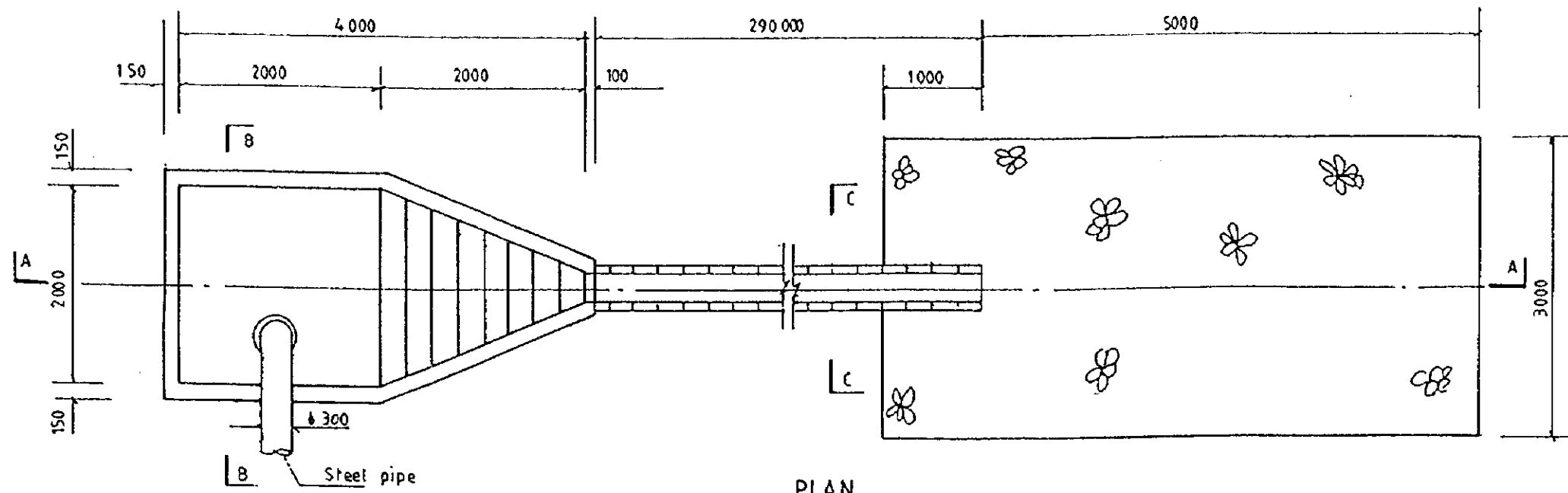
PLAN
