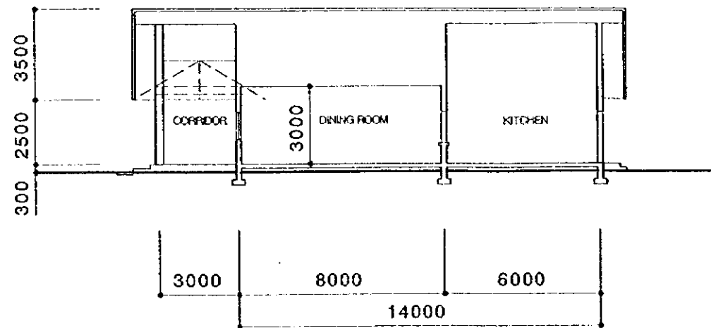
SECTION
