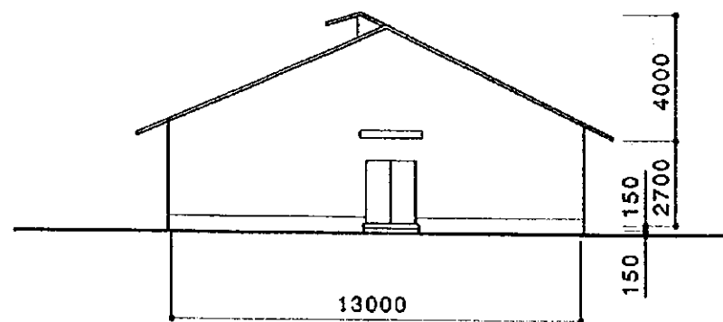
SITE ELEVATION
