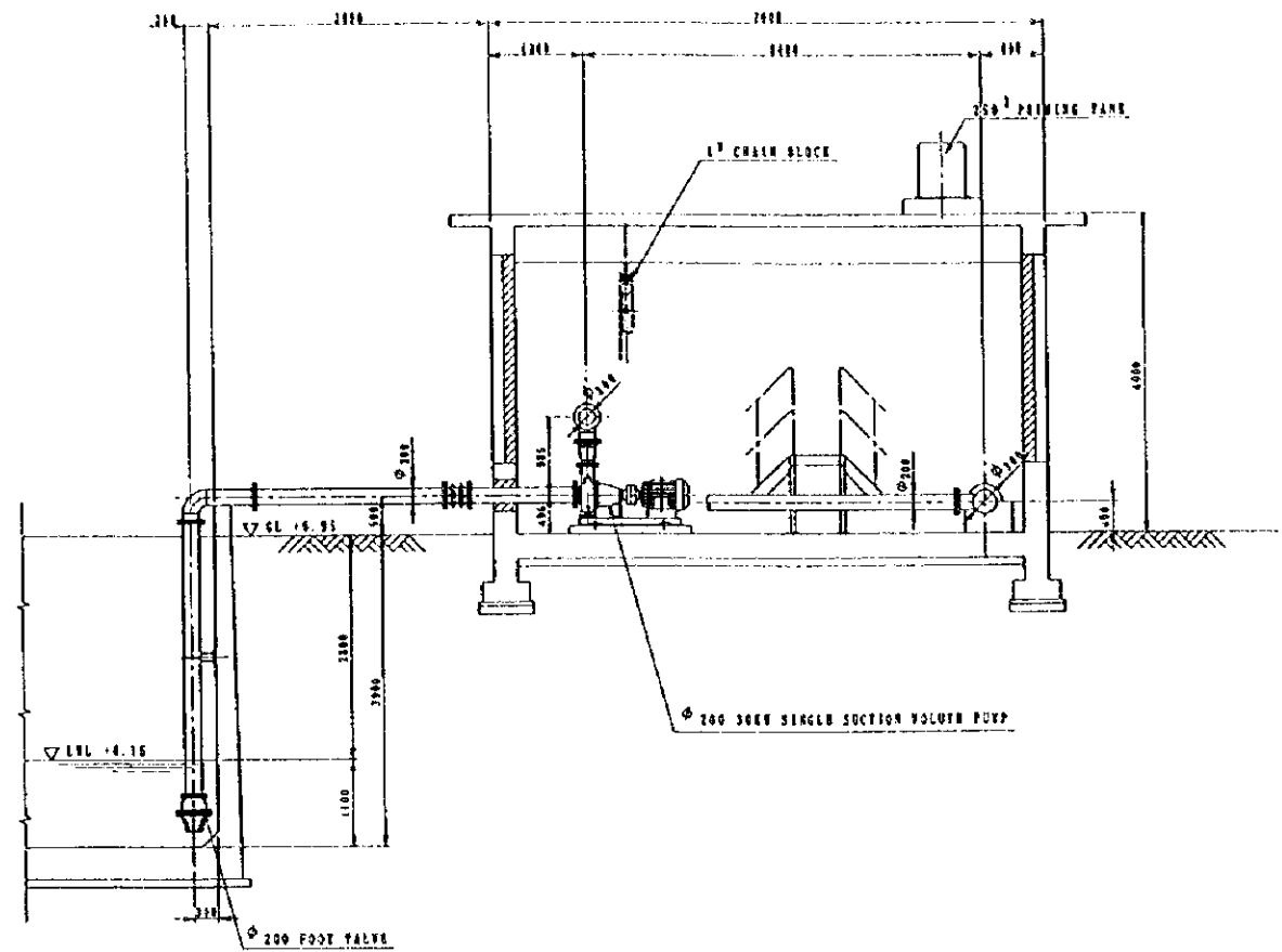
SECTION A - A S-1/50
