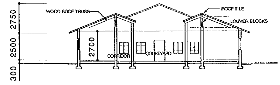
SECTION
