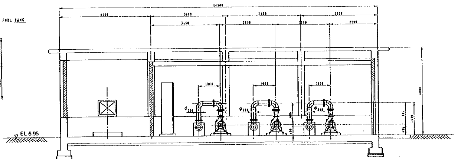
SECTION B - B S-1/50
