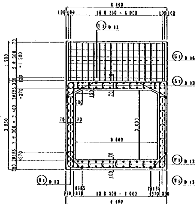
SECTION S=1/100
