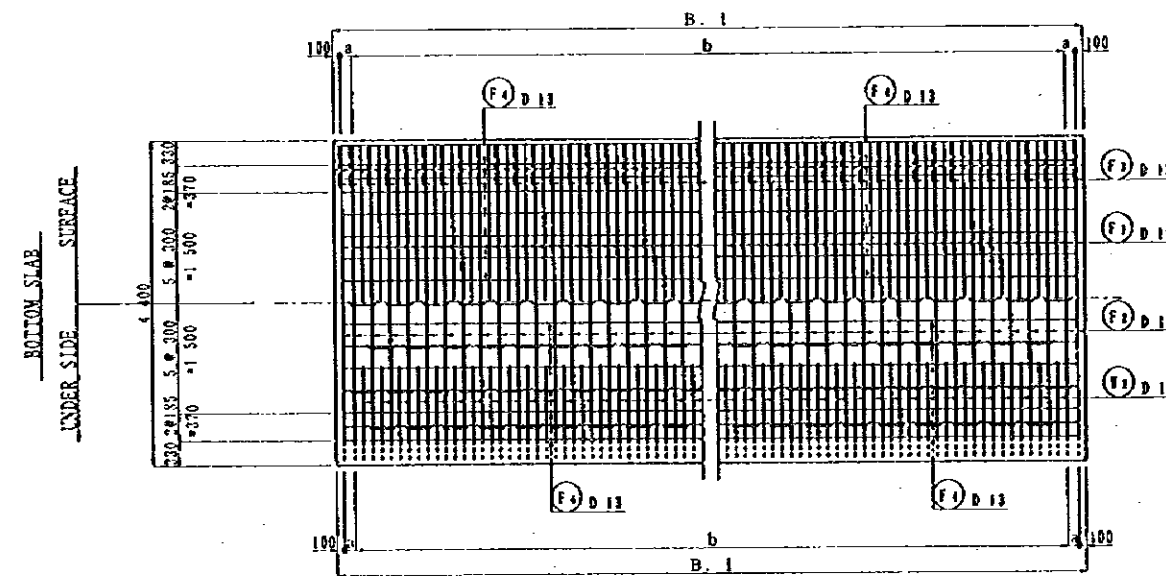
PLAN S=1/100
