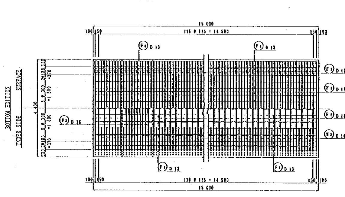
PLAN S=1/100
