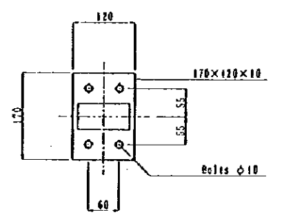
SECTION B-E SCALE 1/10
