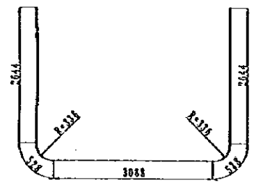
(V1) 2-D32 x 9 440
