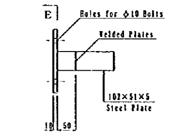
DETAIL d SCALE 1/10
