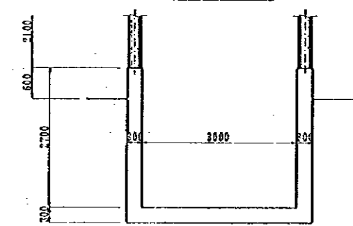
CROSS SECTION E-E SCALE 1/100
