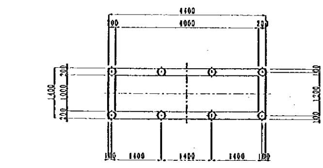
SECTION D-D SCALE 1/100
