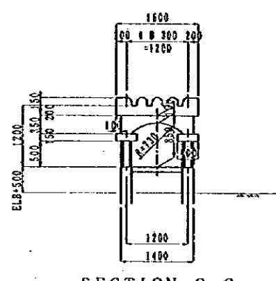
SECTION C-C SCALE 1/100
