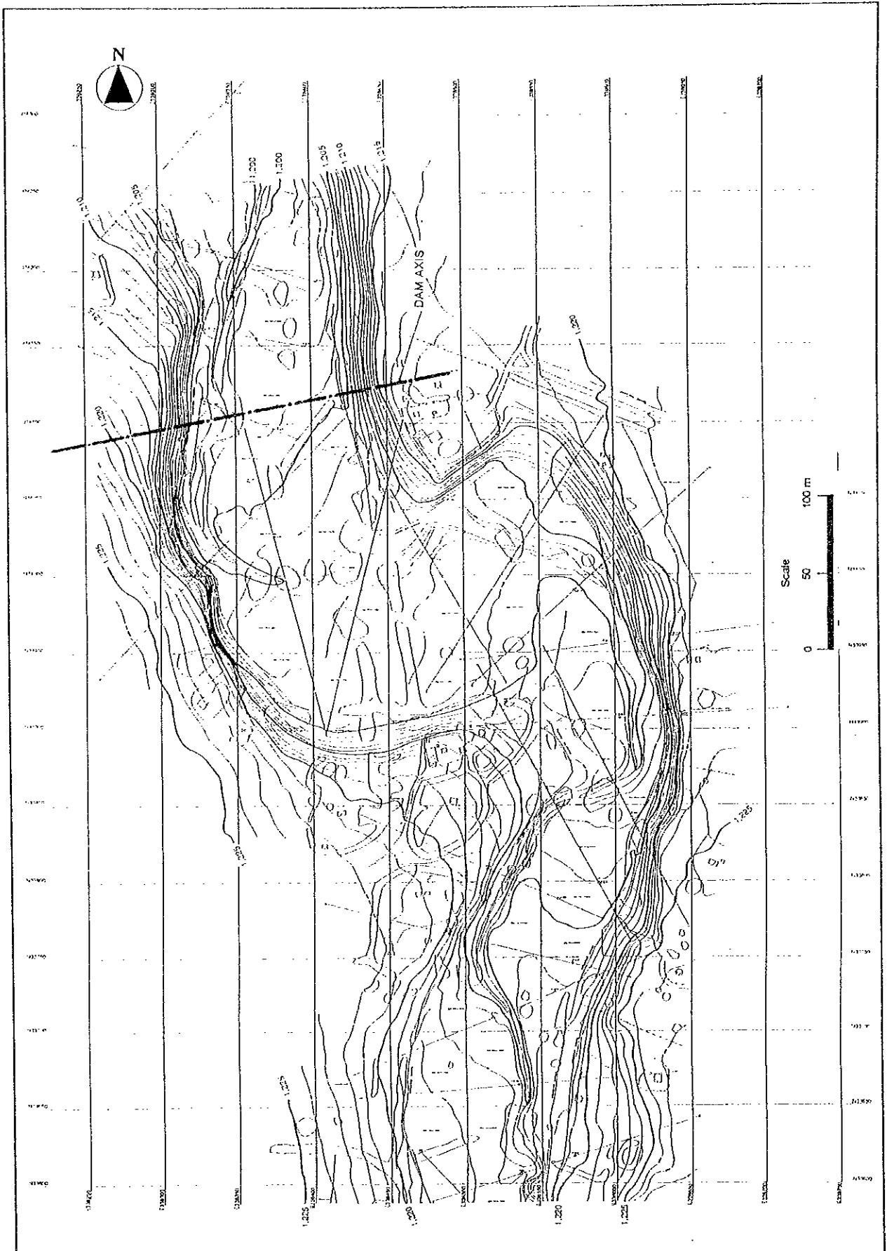
Figure 2.2-9 Topography of Isiolo Dam Site
