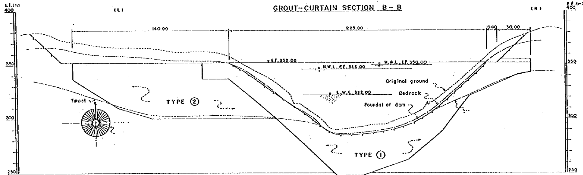
GROUT-CURTAIN
