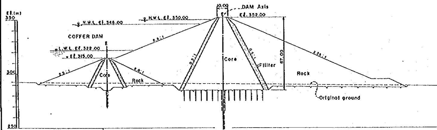
GROUT-CURTAIN SECTION B-B
