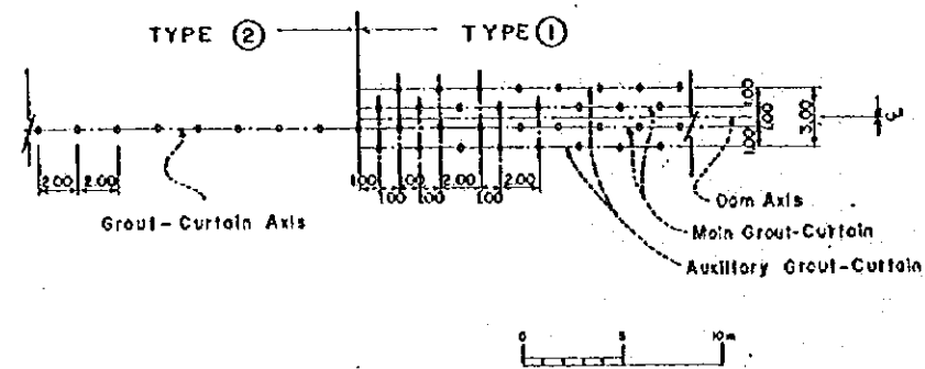
GROUT-CURTAIN
