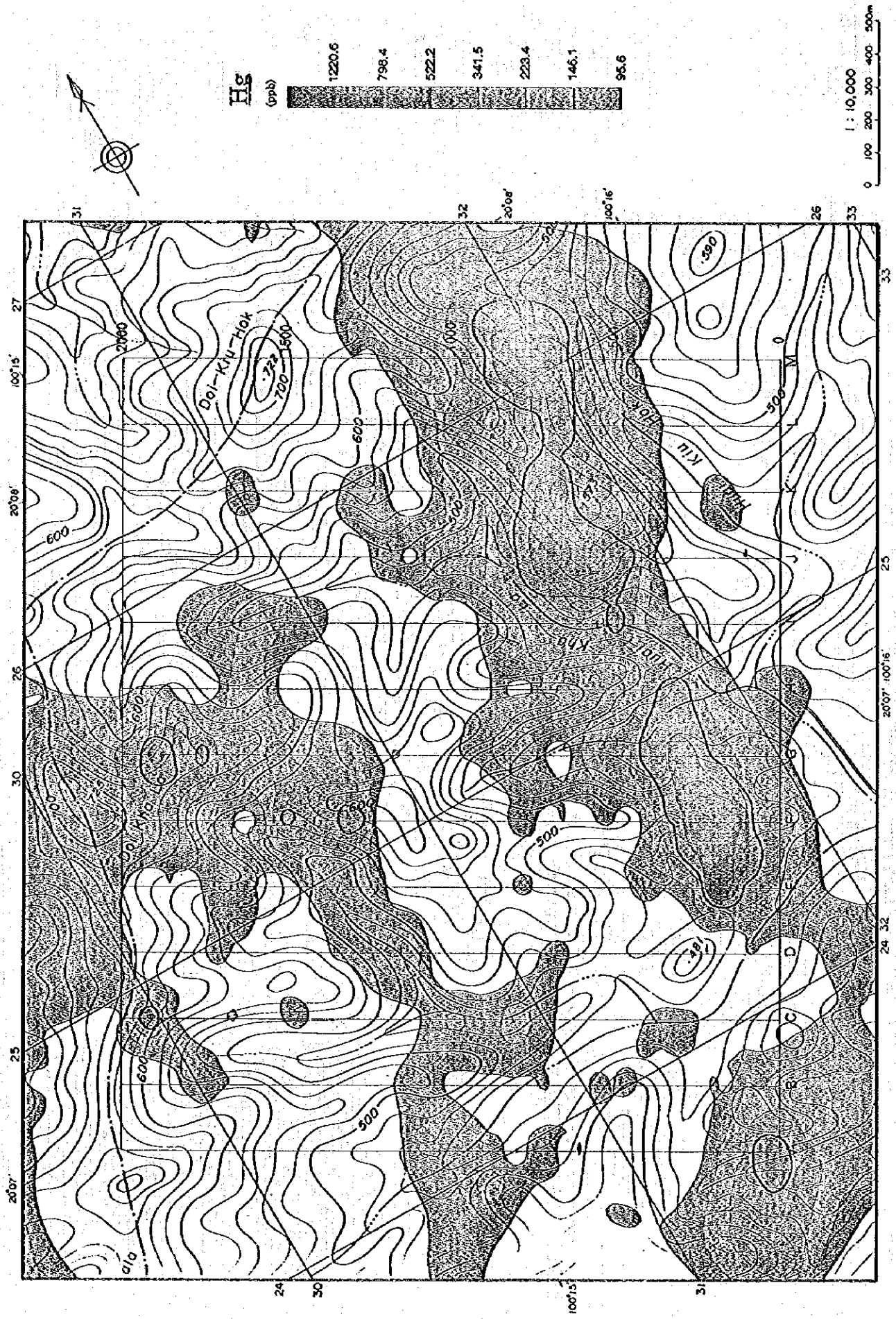
Fig. II-1-10.10 Geochemical Anomaly Map in Detailed Survey Zone (Fig.
