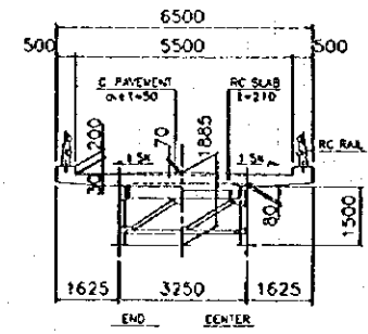
SECTION SCALE = 1/100
