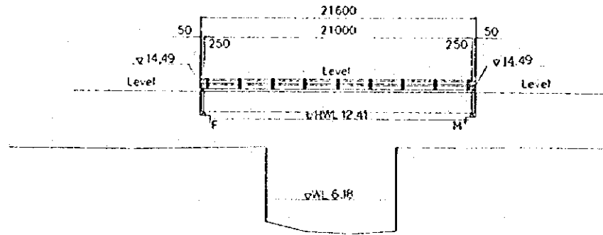
PROFILE SCALE = 1/200
