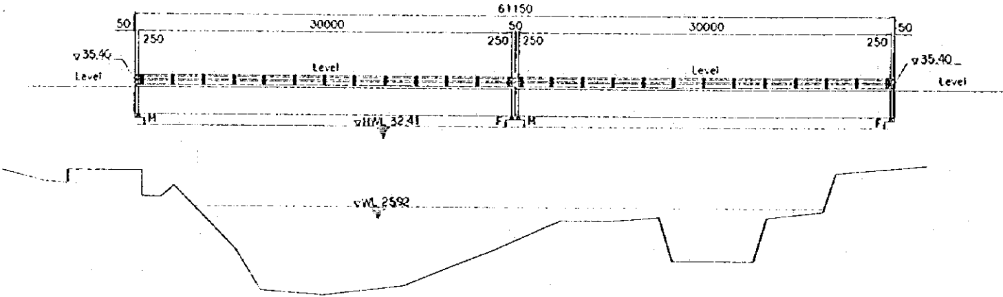
PROFILE SCALE = 1/200
