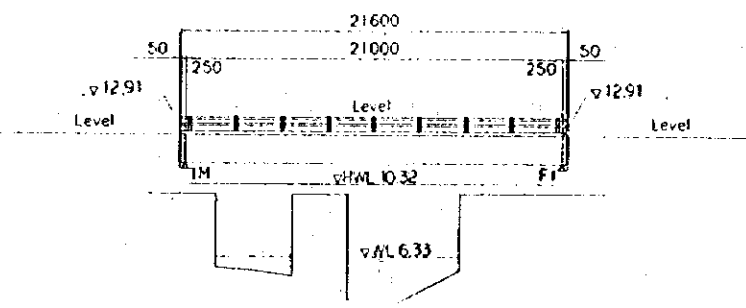
PROFILE SCALE = 1/200
