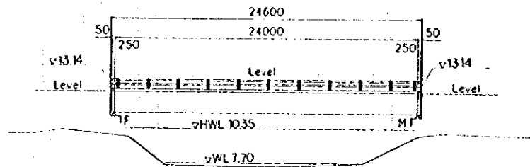
PROFILE SCALE = 1/200
