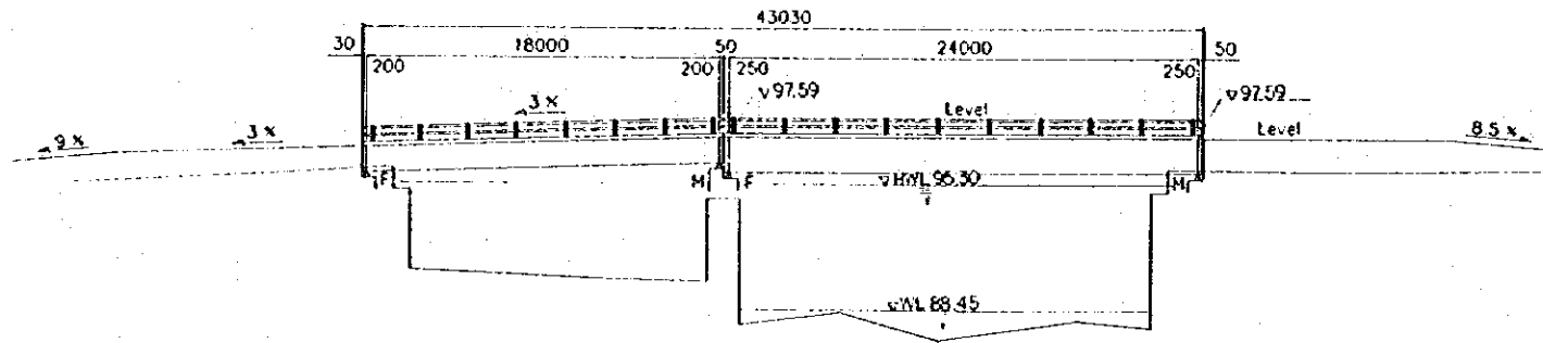
PROFILE SCALE = 1/200
