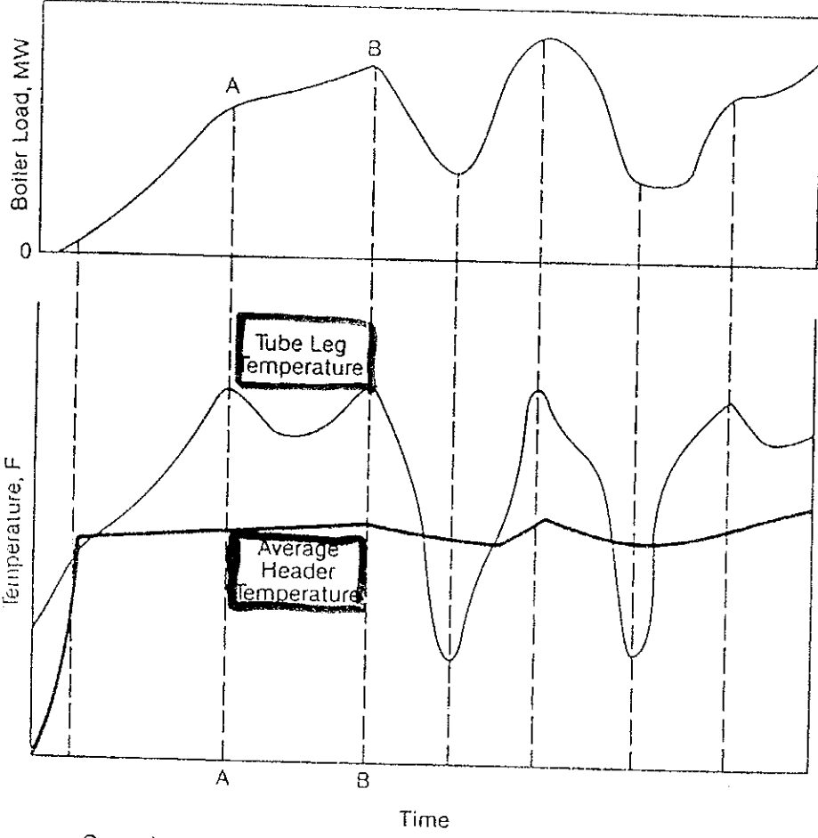
Superheater tube leg temperatures vary with load.
