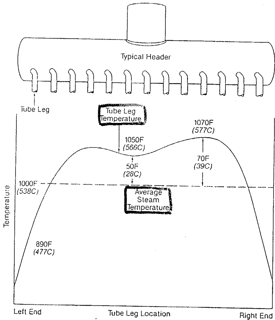
Steam temperature variation in a header.
