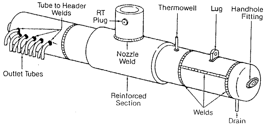
Header locations susceptible to cracking.
