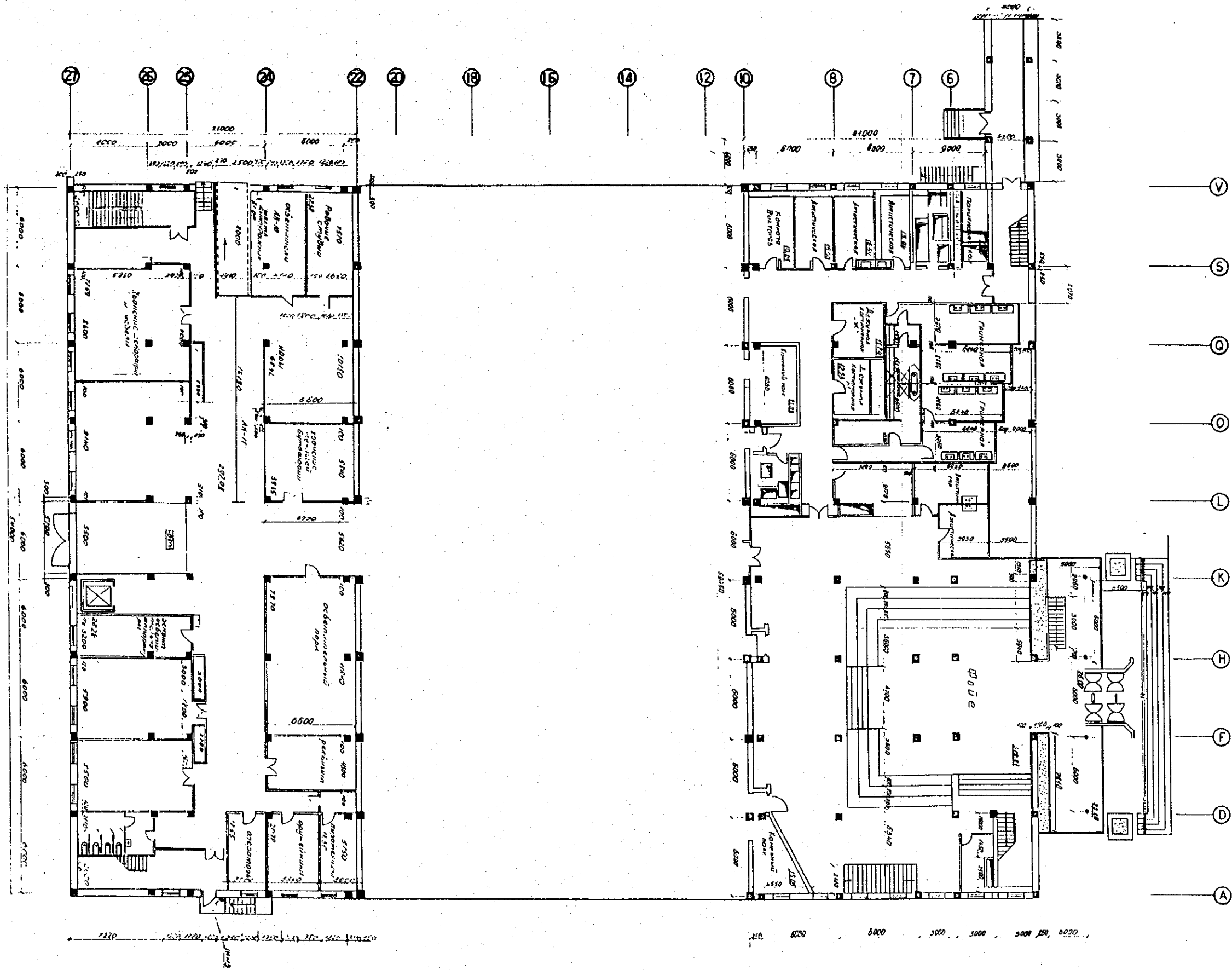
5.2. Floor plan of SNBC's Television Center 1F
