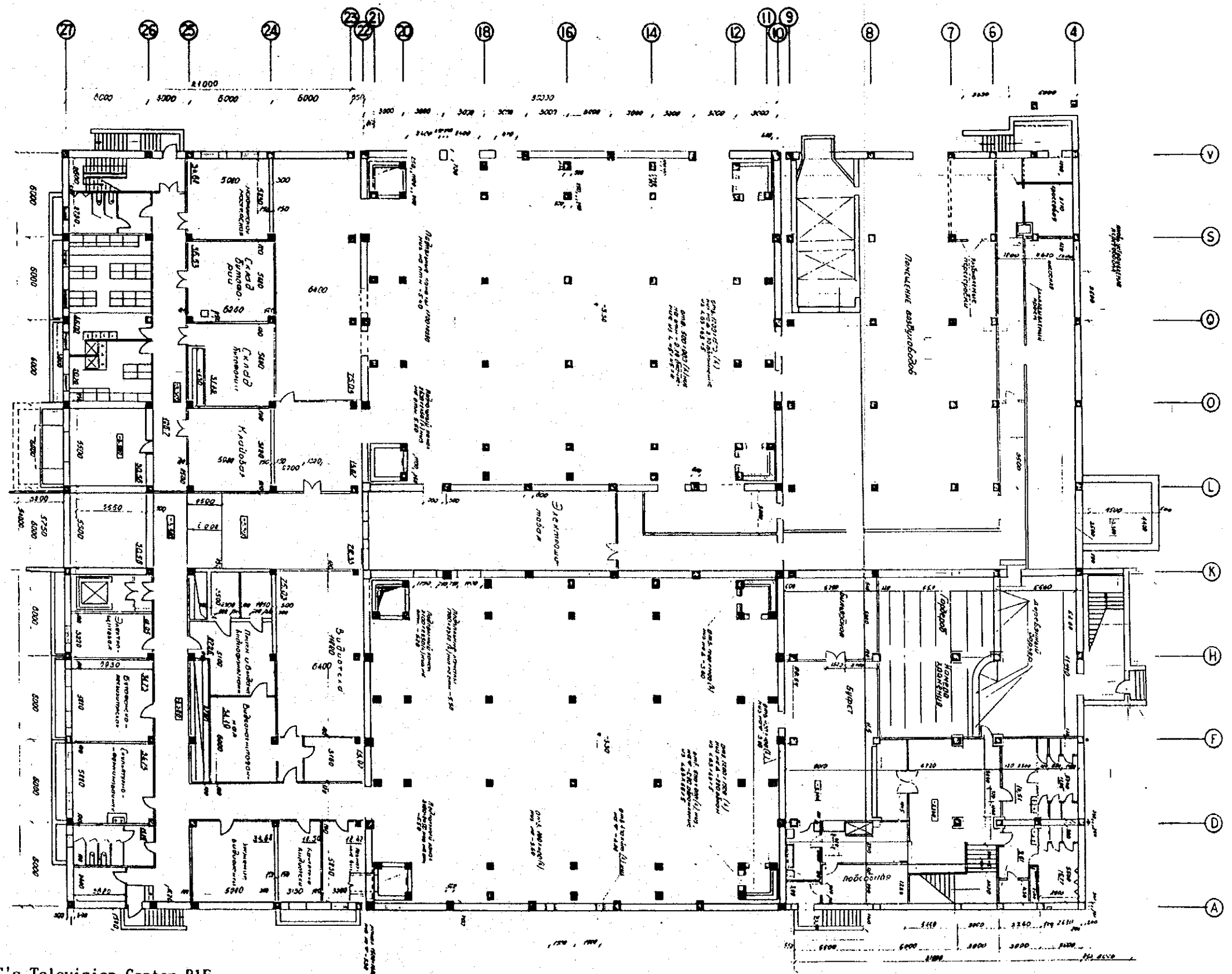
5.1. Floor plan of SNBC's Television Center B1F
