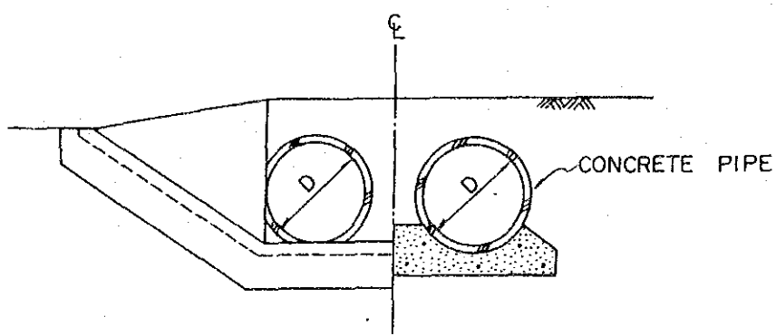
PROFILE SCALE - A
