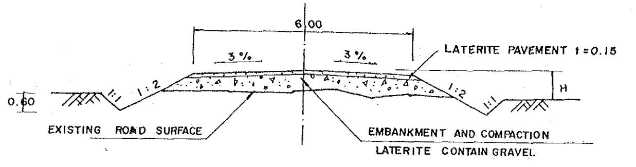
TYPICAL SECTION OF ROAD IMPROVEMENT S=1:100
