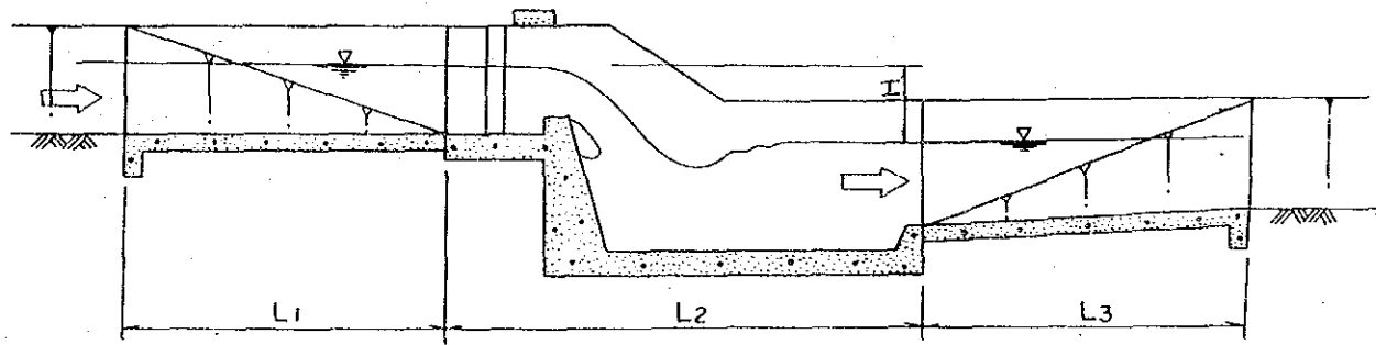
PROFILE SCALE-A
