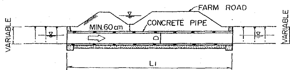
PROFILE SCALE - A
