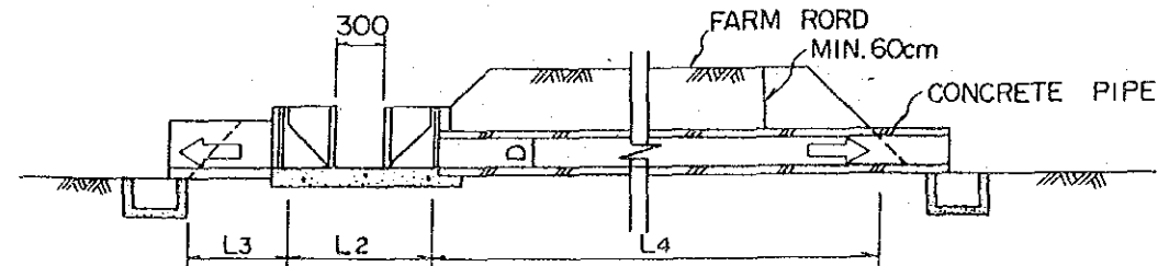
PROFILE SCALE-B
