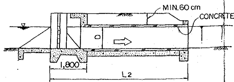
SECTION B-B SCALE-A
