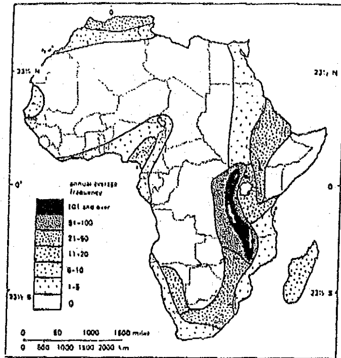
Fig 182. The annual average frequency of earthquakes in Africa. Note the very high frequency associated with the Rift Valley faulted zone in eastern Africa
